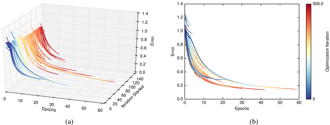
Fig 4: A visualisation of the progression of the optimization curves throughout the optimization procedure on the probabilistic matrix factorization problem. Figure 4a shows for each distinct hyperparameter setting evaluated, the optimization curve run out by the procedure. The curves are ordered by the iteration in the Bayesian optimization procedure that they were started and each epoch of each curve is colored by the iteration of the Bayesian optimization that this section was evaluated. From the figure we can see that the procedure frequently stops running training curves that are not promising and often returns to promising training curves that were previously started. Figure 4b shows a two dimensional cross section of Figure 4a.
