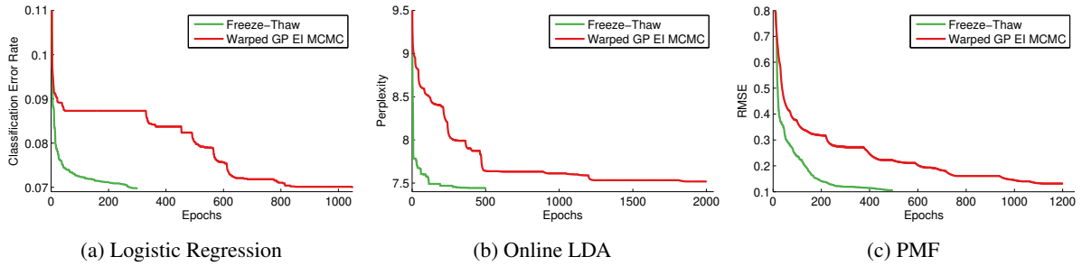
Fig 3: This figure shows the results of the empirical comparison to standard Bayesian optimization on three common machine learning hyperparameter optimization problems. For each problem we report the lowest loss observed over all training epochs evaluated by each method, averaged over five optimization runs.
