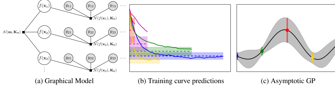
Fig 2: (a) Factor graph representation of the GP model for training procedures. Each row represents a learning curve that is drawn from an independent GP prior, conditioned on its mean. The mean of each learning curve is jointly drawn with the mean of the other curves using another GP prior. (b) Partially completed training curves, and the GP prediction at their eventual asymptotes. (c) The posterior GP prediction at the asymptote. Each colored point represents the GP prediction at the hyperparameter location corresponding to a training curve with the same color.
