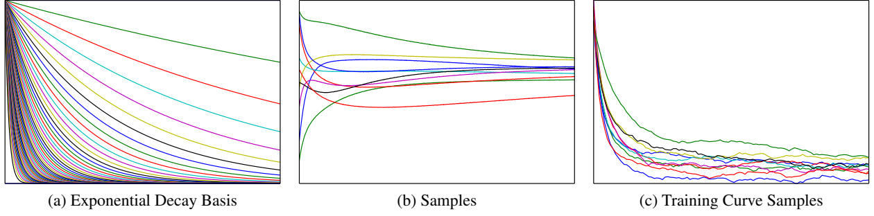
Fig 1: Example functions from the exponential decay kernel. (a) Example functions from our basis set with \alpha = 1.0 and \beta = 0.5 . (b) Samples from a Gaussian process with this covariance function. (c) Samples from a Gaussian process conditioned on the curves starting at a positive number and with an added Ornstein-Uhlenbeck kernel to simulate natural training curves.
