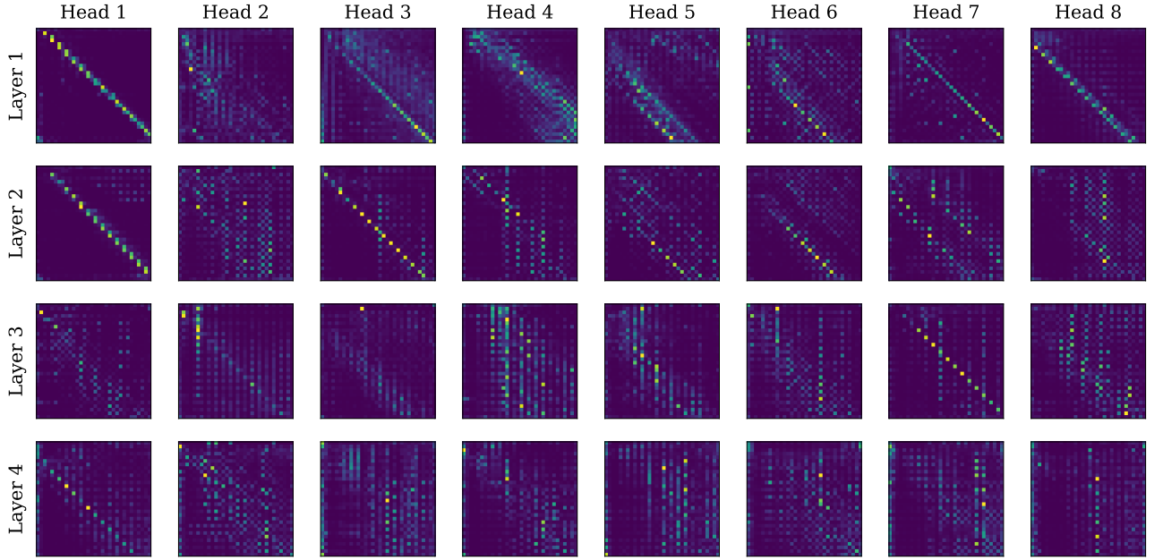
(b) Float
