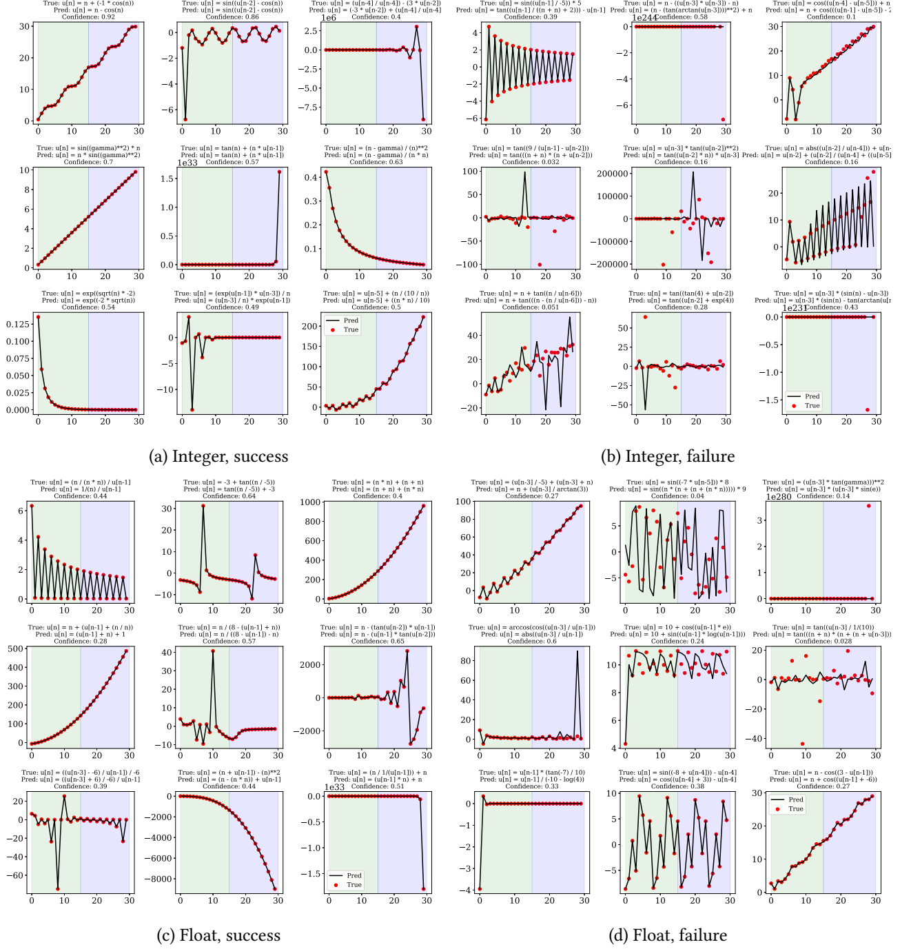
Figure 7: Success and failure modes of our models. The models are fed the first 15 terms of the sequence (green area) and predict the next 15 terms (blue area). We randomly selected expressions with 3 operators from our generator, and picked the first successes and failures.
