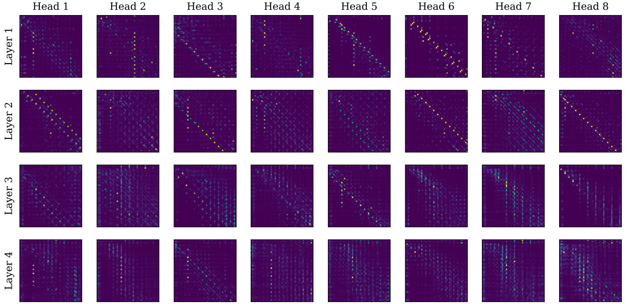
(a) Integer
