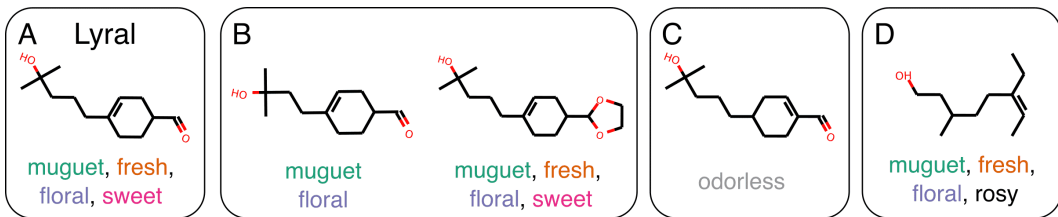
Figure 1: Structurally similar molecules do not necessarily have similar odor descriptors. A. Lyrall, the reference molecule. B. Molecules with similar structure can share similar odor descriptors. C. However, a small structural change can render the molecule odorless. D. Further, large structural changes can leave the odor of the molecule largely unchanged. Example from Ohloff, Pickenhagen and Kraft [28].
