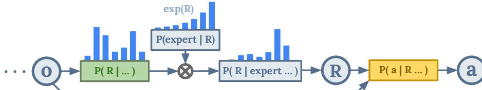
Figure 4: An illustration of our expert-level return and action sampling procedure. P_\theta(R | \dots) and P_\theta(a | R \dots) are the distributions learned by the sequence model.
