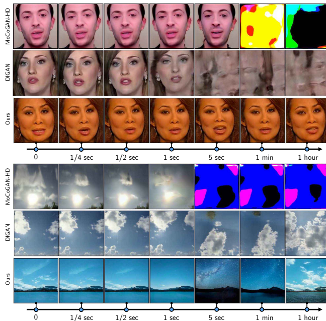
Figure 1. Examples of 1-hour long videos, generated with different methods. MoCoGAN-HD [67] fails to generate long videos due to the instability of the underlying LSTM model when unrolled to large lengths. DIGAN [5] struggles to generate long videos due to the entanglement of spatial and temporal positional embeddings. StyleGAN-V (our method) generates plausible videos of arbitrary length and frame-rate. Also, unlike DIGAN, it learns temporal patterns not only in terms of motion, but also appearance transformations, like time of day and weather changes.
