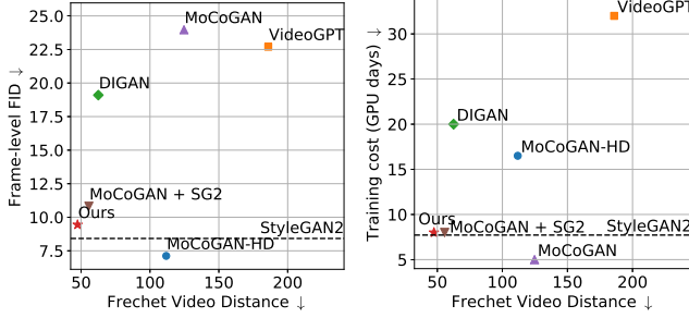
Figure 3. FID scores and training cost by FVD 16 for modern video generators on FaceForensics 256 2 [55]. Our method (denoted by \star ) shows that video generators can be as efficient and as good in terms of image quality as traditional image based generators (like, StyleGAN2 [31], denoted with the dashed line). FID for video generators was computed from 16-frames long videos.
