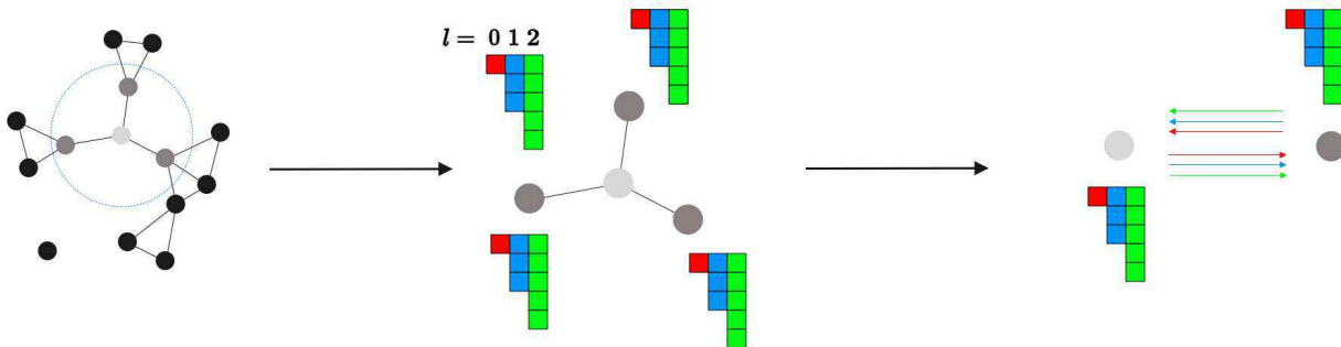
FIG. 1: Left: a set of atoms is interpreted as an atomic graph with local neighborhoods. Middle: every atom carries a set of scalar, vector, and higher-order tensor features with it. Right: atoms exchange information via filters, that are again geometric tensors of increasing order.
