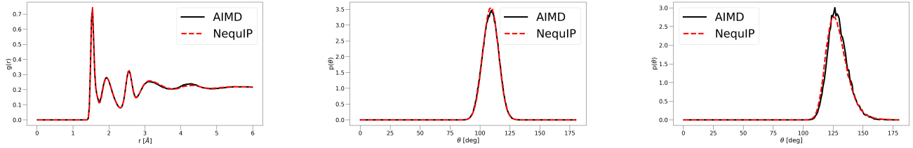
FIG. 5: Left: Radial Distribution Function, middle: Angular Distribution Function, tetrahedral bond angle, right: Angular Distribution Function, bridging oxygen. All are defined as probability density functions; NequIP results are averaged over 10 runs with different initial velocities.
