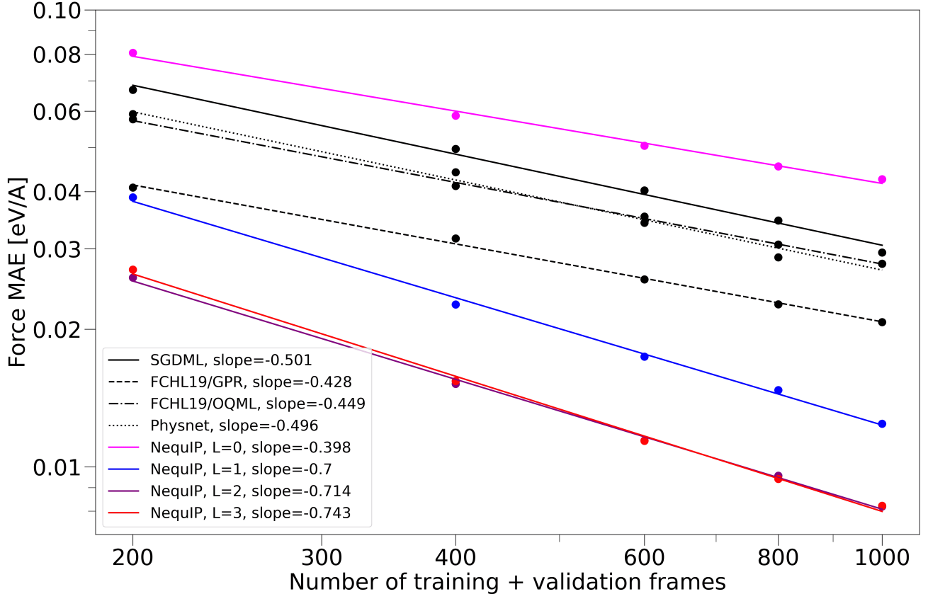
FIG. 8: Log-log plot of the predictive error on the aspirin molecule in MD-17 using NequIP with l \in \{0, 1, 2, 3\} as a function of data set size used for training and validation, measured via the force MAE. The plot also shows errors of a series of other methods, including both kernel and deep-learning approaches.
