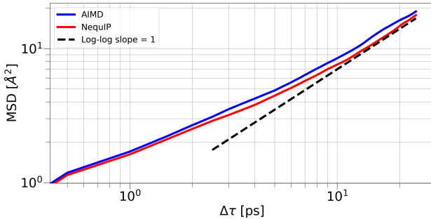
FIG. 6: Comparison of the Lithium mean square displacement of AIMD and an example NequIP trajectory.
