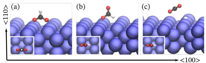
FIG. 3: Perspective view of atomic configurations of (a) bidentate HCOO (b) monodentate HCOO and (c) \text{CO}_2 and a hydrogen adatom on a Cu(110) surface. The blue, red, black, and white spheres represent Cu, O, C, and H atoms, respectively. The subset shown in each subplot is the corresponding top view along the \langle 110 \rangle orientation.
