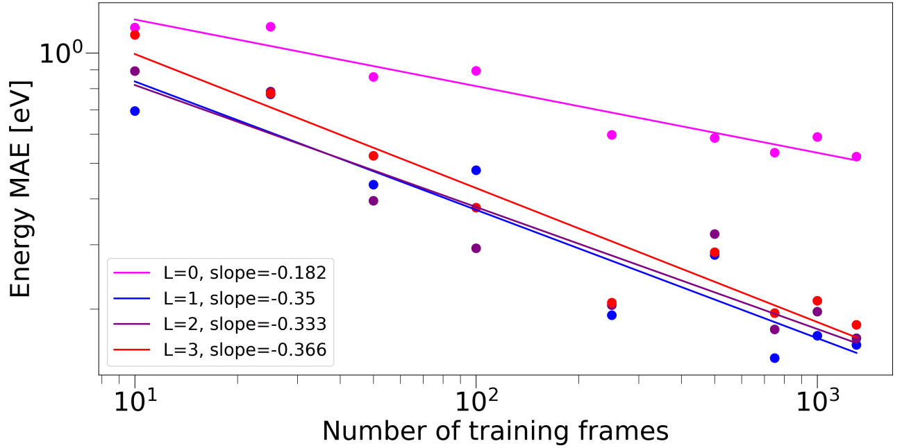
FIG. 10: Log-log plot of the predictive error on the water data set from [50] using NequIP with l \in \{0, 1, 2, 3\} as a function of training set size, measured via the energy MAE.
