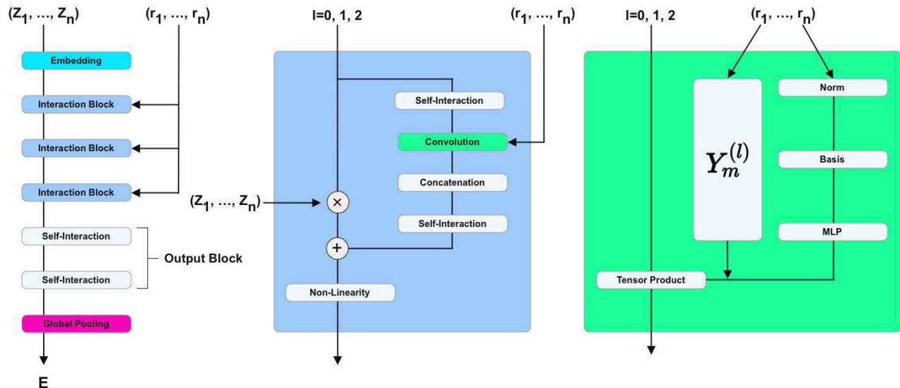
FIG. 2: The NequIP network architecture. Left: atomic numbers are embedded into l = 0 features, which are refined through a series of interaction blocks, creating scalar and higher-order tensor features. An output block then generates atomic energies, which are pooled to give the total predicted energy. Middle: the interaction block, containing the convolution. Right: the convolution combines the radial function R(r) which operates only on interatomic distances with the spherical harmonic projection of the unit vector \hat{r}_{ij} via a tensor product.
