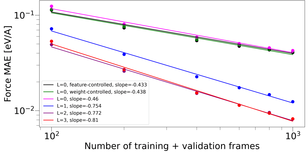
FIG. 11: Log-log plot of the predictive error on the aspirin molecule in MD-17 using NequIP with l \in \{0, 1, 2, 3\} as a function of data set size, measured via the force MAE. The plots also shows the weight- and feature-controlled version of NequIP.
