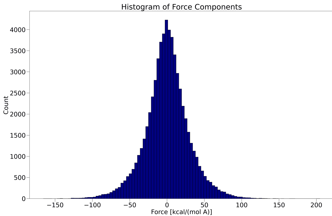
FIG. 13: Histogram of force components of all structures used for training and validation for the aspirin molecule in the revised MD-17 data set.
