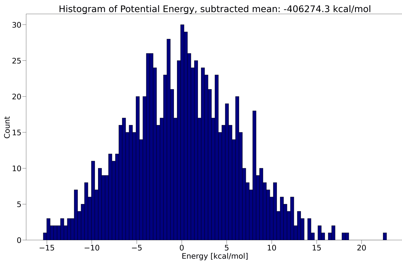
FIG. 12: Histogram of potential energies of all structures used for training and validation for the aspirin molecule in the revised MD-17 data set. The mean energy was subtracted before plotting.
