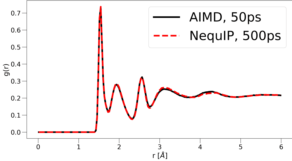
FIG. 9: Comparison of the Radial Distribution of a simulation of \text{Li}_4\text{P}_2\text{O}_7 of length 500 ps driven by NequIP in comparison to a 50 ps simulation driven by AIMD.
