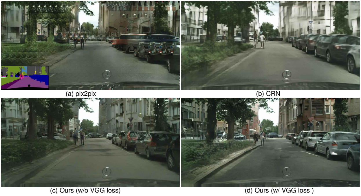
Figure 9: Comparison on the Cityscapes dataset [7] (label maps shown at the lower left corner in (a)). For both without and with VGG loss, our results are more realistic than the other two methods. Please zoom in for details.
