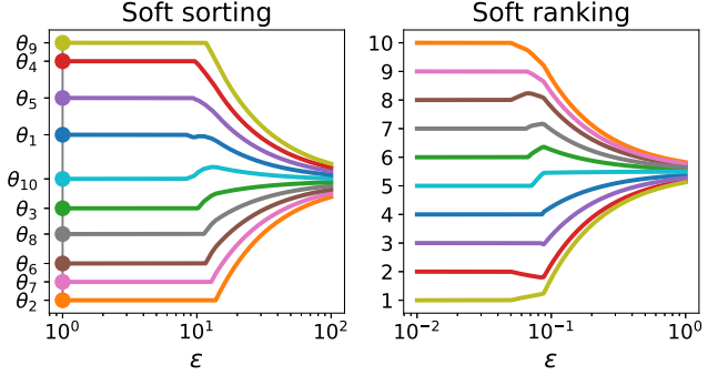
Figure 2. Illustration of the soft sorting and ranking operators, s_{\varepsilon\Psi}(\theta) and r_{\varepsilon\Psi}(\theta) for \Psi = Q ; the results with \Psi = E are similar. When \varepsilon \rightarrow 0 , they converge to their “hard” counterpart. When \varepsilon \rightarrow \infty , they collapse into a constant, as proven in Prop.2.
