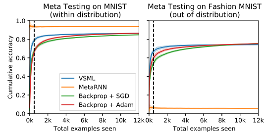
Figure 19: Short horizon bias.
