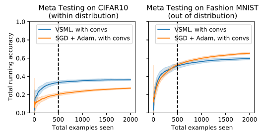
Figure 21: Meta Training on CIFAR10 with a CNN version of VSML.
