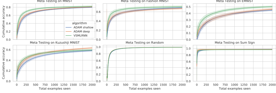
Figure 12: Meta testing learning curves. All 6 meta test tasks are unseen. VSML RNN has been meta trained on MNIST, Fashion MNIST, EMNIST, KMNIST, and Random, excluding the respective dataset that is being meta tested on. Standard deviations are over 32 seeds.
