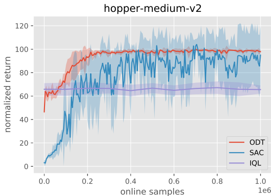
Figure E.1: The training stability comparison of ODT, IQL and SAC. The performance of ODT improves upon pretraining using online interactions, while the performance of IQL stays almost the same as the pretraining result. Both ODT and IQL are stable along the online finetuning yet SAC fluctuates. Results are averaged over 5 training instances with different seeds.
