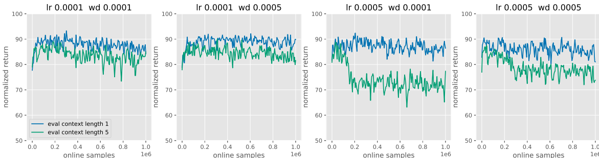
Figure B.1: Comparison of the evaluation context length for finetuning ODT for Ant with medium-replay offline dataset. For varying values of learning rates and weight decays, context length 1 consistently outperforms 5. Results are averaged over 10 training instances with different seeds.
