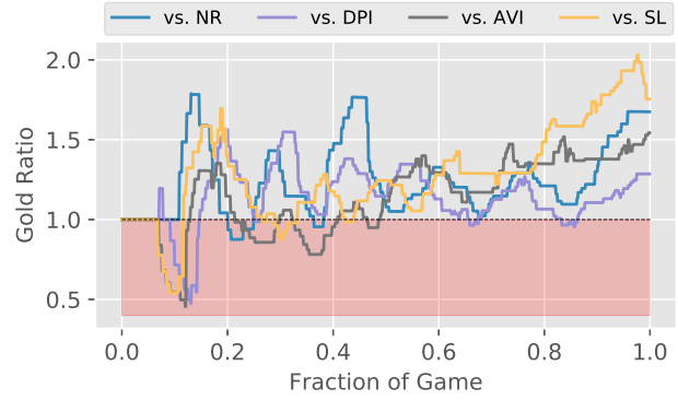
Figure 6. In-game Behavior
