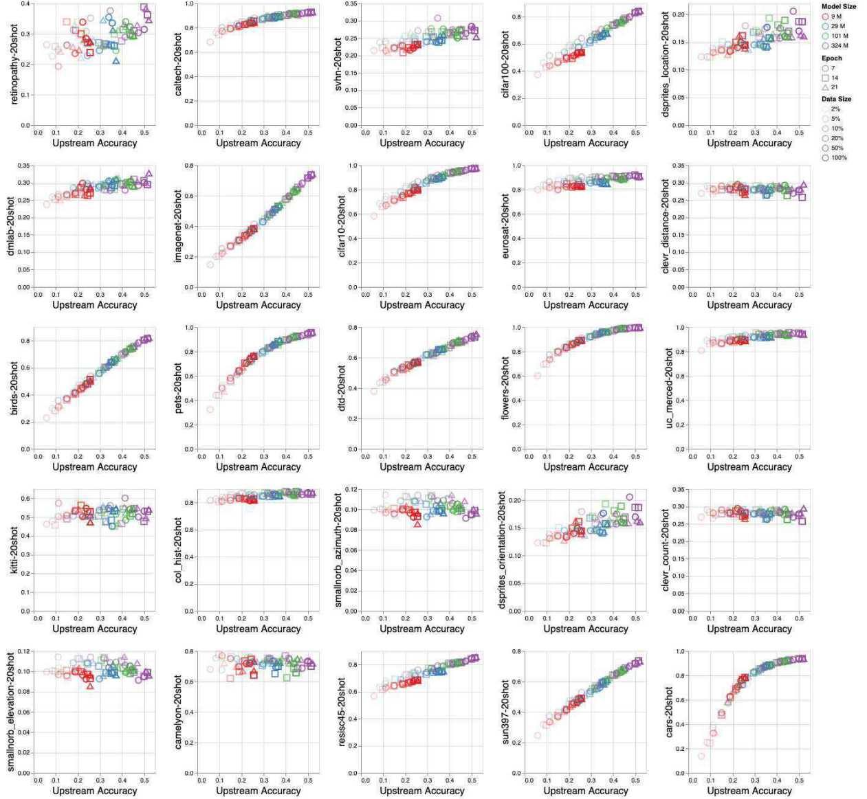
Figure 27: Effect of controlled scale up with respect to the model size (number of parameters), data size (the portion of the pre-trained data), and compute (epochs) on 25 different downstream tasks in the few-shot setup (20-shots).
