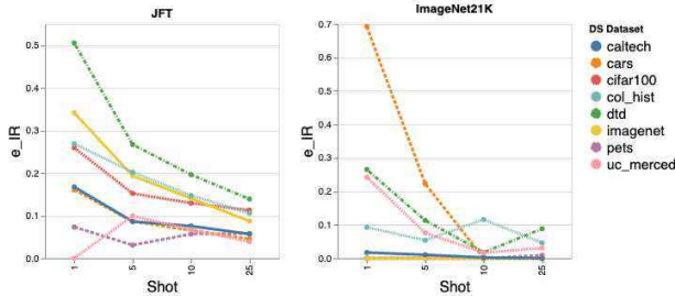
Figure 3: Effect of number of shots and DS/US task on e_{IR} of the power law curves. We note that all of them impact e_{IR} . Figure 15, 16 depicts these plots for all power law parameters.
