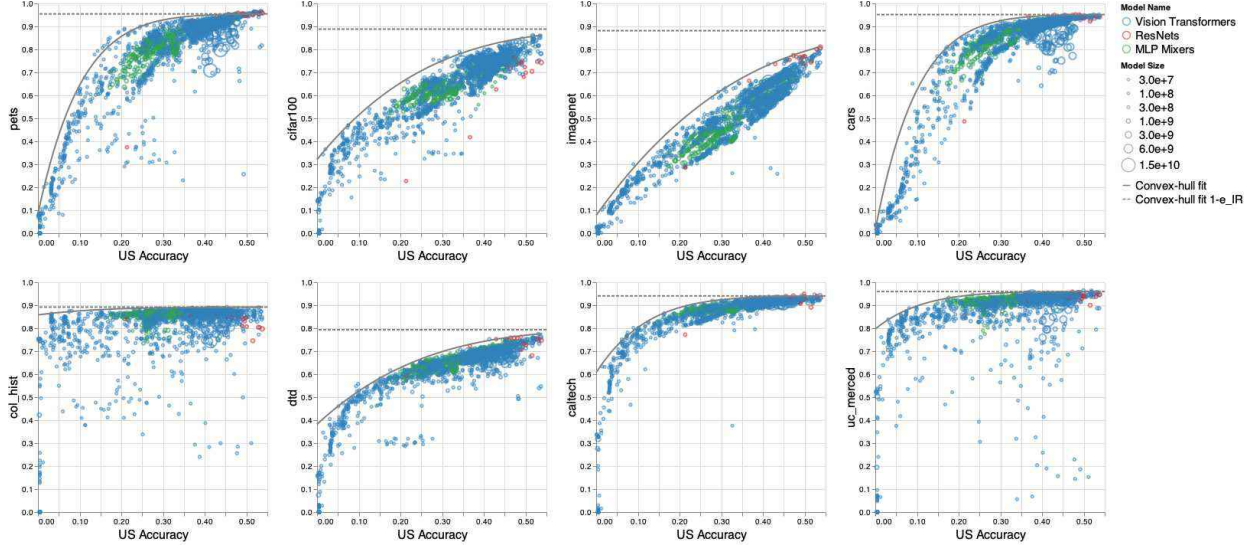
Figure 1: The performance of different downstream (DS) tasks vs of upstream (US) based on more than 1500 different Vision Transformers, 1400 MLP-Mixers and 16 best-performing ResNets (Although the number of ResNet samples is small, this does not hurt our investigations. See Section 1.1 for details), with different configurations. The models are pre-trained on JFT and evaluated in few-shot settings (25 shots). Figure 2 shows the same plot but with more than 4800 experiments including two different upstream tasks of JFT and ImageNet21K for 1 and 25 shots. We consider the convex hull of the points as well since it captures the performance of a randomized classifier made by choosing these models with different probabilities. As the upstream performance improves, the downstream performance starts to saturate. Even if US accuracy reaches 100%, the DS accuracy saturates to a value considerably lower than 100%. We observe a non-linear relationship between upstream and downstream accuracy and model it with a power law function to predict the DS performance given the US performance. The horizontal line is the predicted downstream accuracy if upstream accuracy reaches 100%. We investigate DS-vs-US plots instead of the usual DS-vs-scale plots to capture the effect of hyper-parameter choices and to account for the fact that the scaling impacts DS performance through US performance. Figure 13 depicts the same plot with log scaling of accuracies as done in many related works. Figure 14 depicts the same plot when upstream is ImageNet21K.
