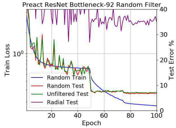
(b) Trained on Randomly Filtered CIFAR-10
