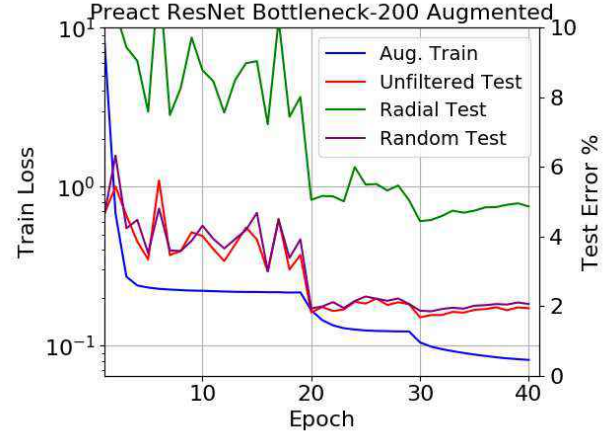
Figure 4: Augmented SVHN Training plots for ResNet-200. Best viewed in color.
