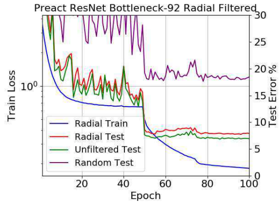
(c) Trained on Radially Filtered CIFAR-10
