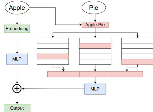
Figure 2: Illustration of multi-head PairConnect layer. Pairwise word embeddings from multiple tables are extracted and concatenated. Then, PairNet passes it through an MLP and sum it with original word embedding. The output serves as input embedding for next layer with independent embedding table for pair.
