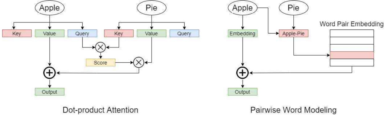
Figure 1: Comparison of pairwise word modelling and attention
