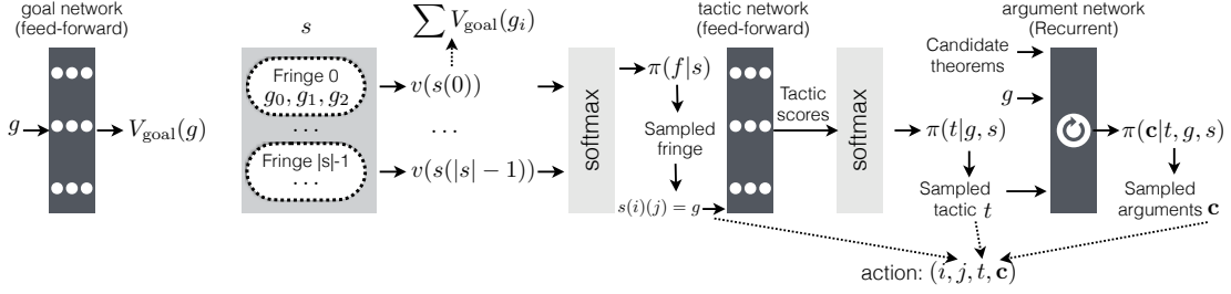
Figure 4: Structure of the model. The functionality of each network is described in subsection 2.2.
