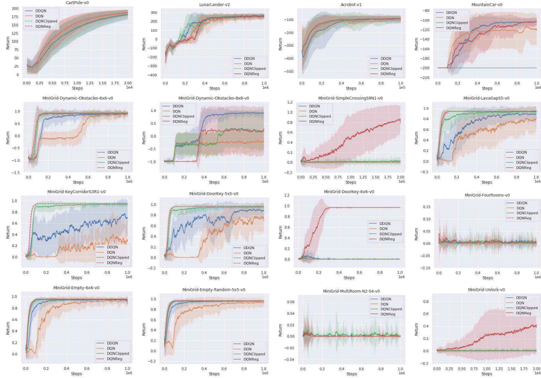
Figure 4: Performance of learned algorithms (DQNCIPPED and DQNREG) versus baselines (DQN and DDQN) on training and test environments as measured by episode return over 10 training seeds. A dashed line indicates that the algorithm was meta-trained on that environment while a solid line indicates a test environment. DQNREG can match or outperform the baselines on almost all the training and test environments. Shaded regions correspond to 1 standard deviation.
