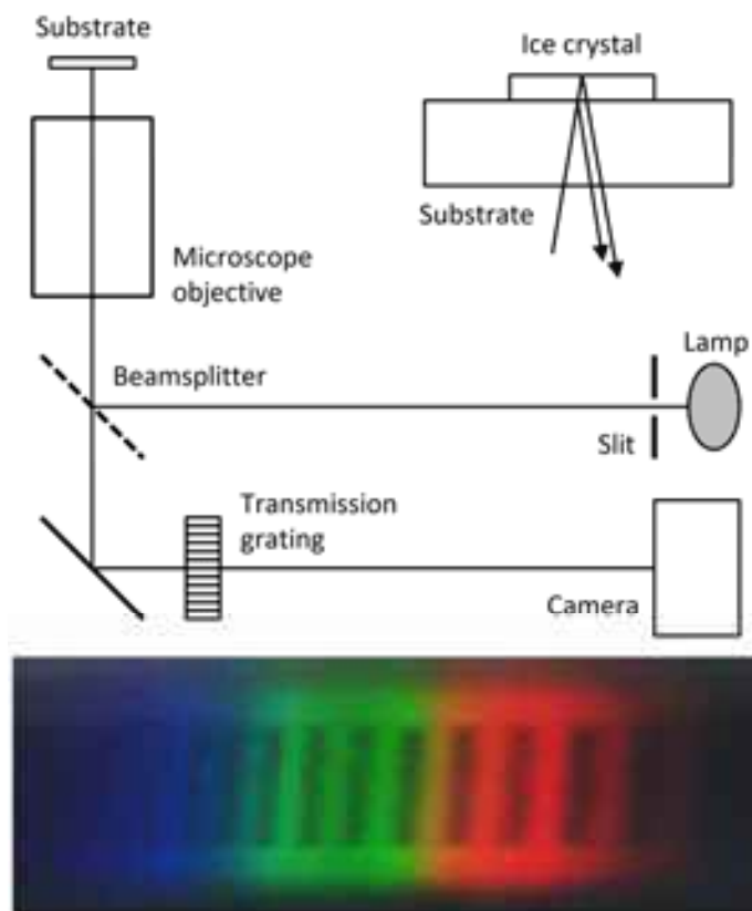
Figure 6.14: (Top) An optical setup for measuring the thickness of thin ice crystal plates using white-light interferometry, described further in the text. The sketch on the upper right shows the interfering reflections from the substrate/ice and ice/air interfaces. (Bottom) An example white-light spectrum, in true color, showing a series of dark interference fringes. The absolute thickness of the ice crystal can be derived from the measured spacing between the optical fringes [2013Lib]. The growth velocity can be determined from the lateral motion of the fringes across the image.
