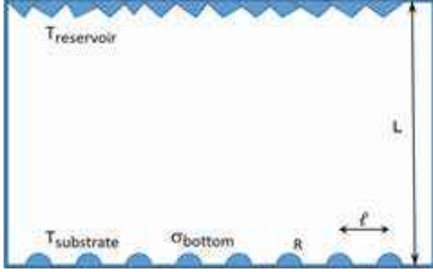
Figure 7.2: If several test crystals are present at the bottom of the growth chamber, they collectively reduce the supersaturation \sigma_{bottom} near the bottom of the chamber. As described in the text, even a small number of ice crystals, covering just a tiny fraction of the substrate area, can have a sizable effect on \sigma_{bottom} .
