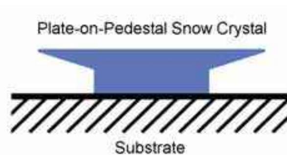
Figure 9.1: A side view of the basic Plate-on-Pedestal (PoP) snow-crystal geometry. A thin plate-like crystal grows outward from the top edge of a small hexagonal prism, while one basal face of the prism rests on a transparent substrate.
