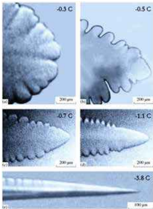
Figure 3.14: Several optical photographs showing ice free-dendrite growth from liquid water as a function of the bath temperature [2004Shi]. Near the freezing point ( -0.3\text{ C} ), the growth is relatively slow, the tip radius is large, and tip splitting can occur. As the bath temperature decreases, the growth rate increases and the tip radius decreases, yielding somewhat different morphological features.
