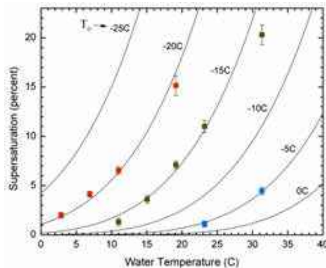
Figure 6.24: The supersaturation in a 1-meter high free-fall convection chamber [2008Lib4] as a function of the water reservoir temperature T_{water} , at several values of the chamber temperature T_0 . Data points show the supersaturation measured using differential hygrometry at -5 C, -15 C, and -20 C. Lines show an empirical model of \sigma(T_0, T_{water}) defined in [2008Lib4].
