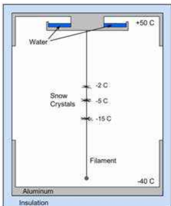
Figure 6.27: This snow-crystal diffusion chamber creates a steep vertical temperature gradient with the top warmer than the bottom. Water vapor evaporates from the warm water reservoir and diffuses downward into the colder air below, yielding highly supersaturated air in the interior of the chamber. In this illustration, snow crystals grow at different temperatures on a vertical filament.
