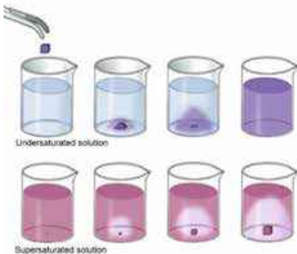
Figure 3.1: The process of diffusion, shown operating in two directions. A crystal dropped into an undersaturated solution will dissolve (top row). Diffusion will then slowly spread the dissolved material throughout the solution. In contrast, a seed crystal placed into a supersaturated solution (bottom row) will grow as diffusion carries material to the crystal and depletes the solution nearby. The first case is analogous to a snow crystal sublimating in undersaturated air, and the second case is analogous to a snow crystal growing in supersaturated air. Adapted from an image found at https://byjus.com/jee/diffusion-of-gases/ .
