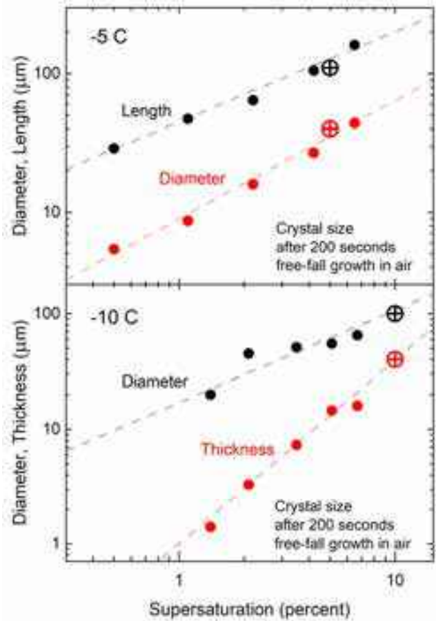
Figure 7.21: Sizes of ice crystals after 200 seconds of growth in free fall through normal air, as a function of the background supersaturation \sigma_\infty . (not equal to \sigma_{surf} ). The solid points are from [2009Lib], and the cross-circle points are from Yamashita in [1987Kob] (reproduced in Figure 6.22). Note that for both columnar crystals at -5 C and plate-like crystals at -10 C, the forms become more isometric with increasing supersaturation.
