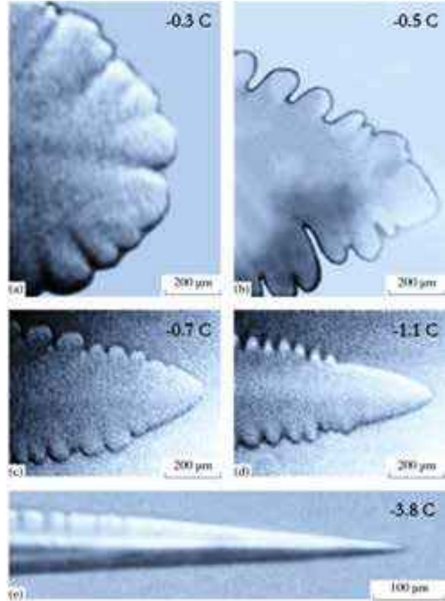
Figure 12.4: Several photographs showing ice free-dendrite growth in a water bath at different bath temperatures [2004Shi]. Near the freezing point ( \Delta T_{bath} = -0.3 C), the growth is relatively slow, the tip radius is large, and tip splitting can occur. As the bath temperature decreases, the growth rate increases, the tip radius decreases, and the overall morphology changes.
