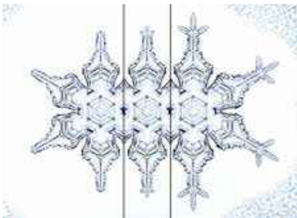
Figure 3.56: This composite photograph shows the phenomenon of induced sidebranching on a laboratory-grown POP snow crystal. The left image shows the crystal after long branch tips were first grown out at high supersaturation, and then the branch tips became faceted after a short period of low supersaturation. Increasing the supersaturation again then caused central branches and sidebranches to sprout simultaneously on the tips of all the primary branches.
