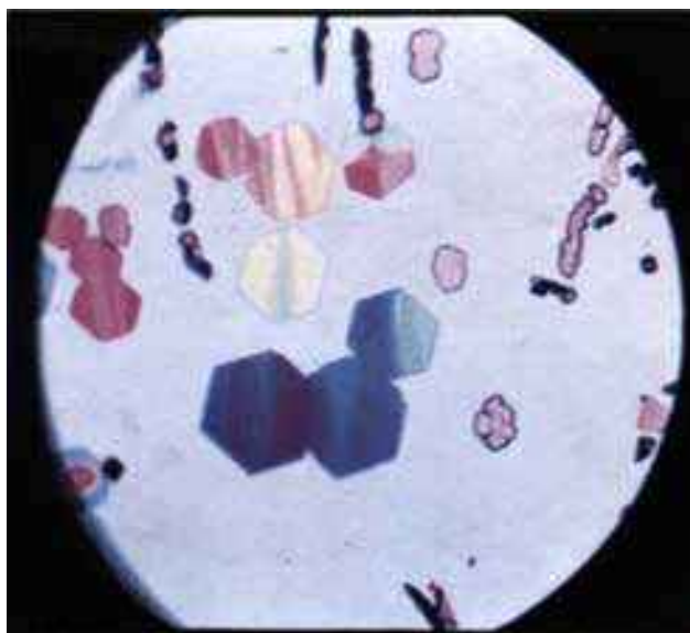
Figure 6.39: Thin ice-crystal plates grow epitaxially on a cleaved covellite crystal. Note the alignment of the different ice prism facets, indicating the orientation of the underlying substrate crystal. Colors arise from the interference of reflections off the ice/air and ice/CuS surfaces, with the overall color depending on the thicknesses of the ice. (Image from [1959Bry].)
