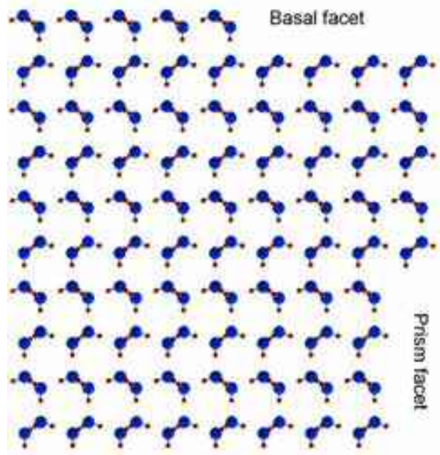
Figure 2.9: A projection of the ice Ih lattice looking along the [11\bar{2}0] direction, showing basal and prism facets and terrace steps. The spacing between basal layers is c_0/2 = 0.37 nm, while the spacing between prism layers is (\sqrt{3}/2)a_0 = 0.39 nm.
