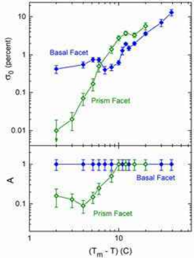
Figure 7.18: Experimental data showing the attachment coefficient fit parameters \sigma_0(T) and A(T) for the basal and prism facets, assuming a functional form \alpha(\sigma_{surf}) = Ae^{-\sigma_0/\sigma_{surf}} for both \alpha_{basal} and \alpha_{prism} . The data were consistent with A = 1 for all the basal data and for the prism data when T \leq -10C , so this constraint was applied when fitting \sigma_0 over these temperature ranges [2013Lib]. The prism data with T > -10C were better described with A < 1 as shown.
