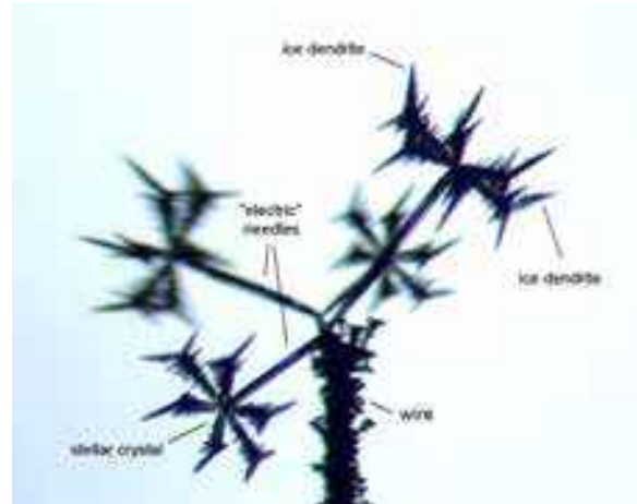
Figure 3.12: The crystal structure of fishbone dendrites can be difficult to discern from optical photographs like those in the previous two figures. Observing their growth on c -axis e-needles (see Chapter 8) allows an unambiguous determination of the sidebranch orientations with respect to the crystal axes, as described in [2009Lib1].
