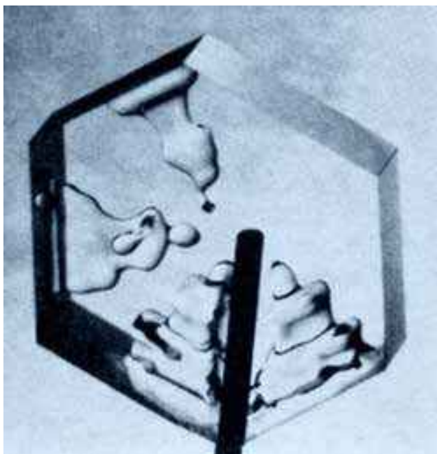
Figure 3.64: A photograph of a “negative” snow crystal growing at -14^{\circ}\text{C} [1965Kni]. The capillary tube (black) has a diameter of 0.45 mm. The overall faceted shape arises from a strong nucleation barrier in the sublimation kinetics, while the protrusions result from thermal-diffusion-limited growth. As with normal snow crystal growth, faceting is a nonequilibrium process dominated by molecular kinetics, while surface energy effects (which define the equilibrium crystal shape) are likely negligible.
