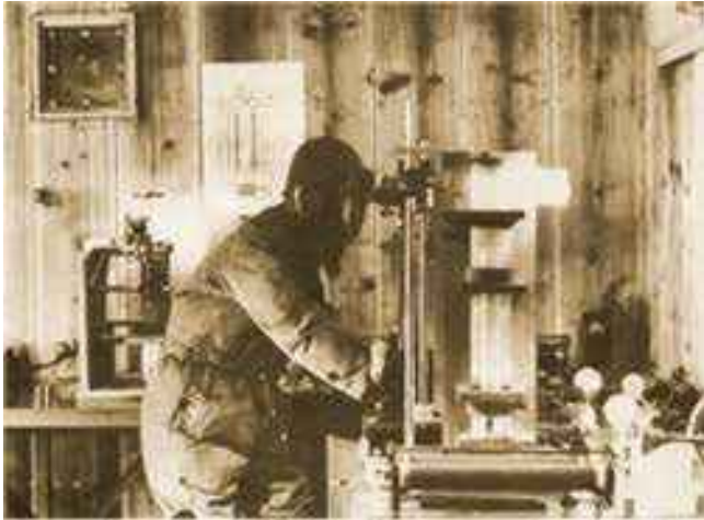
Figure 1.21: Japanese physicist Ukichiro Nakaya working in his refrigerated snow-crystal laboratory in Hokkaido University [1954Nak].
