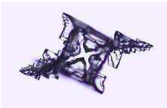
Figure 9.34: A small twinned snow crystal that happened to fall on the PoP substrate.
