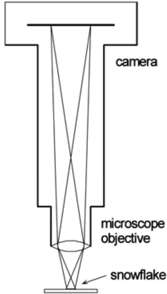
Figure 11.9: A basic DIY photo-microscope consists of little more than a microscope objective, an extension tube, and a camera body. Viewing is done through the camera, for example displaying the image on a TV monitor via the live-feed camera output. The field of view of the camera can be set by choosing an appropriate length for the extension tube, which is the same as with reversed-lens setups.
