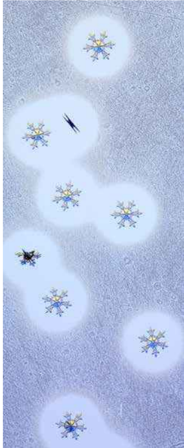
Figure 9.39: (Above, and facing page) Clusters of small PoP crystals all exhibiting about the same growth conditions as a function of time, and thus all growing into similar shapes.
