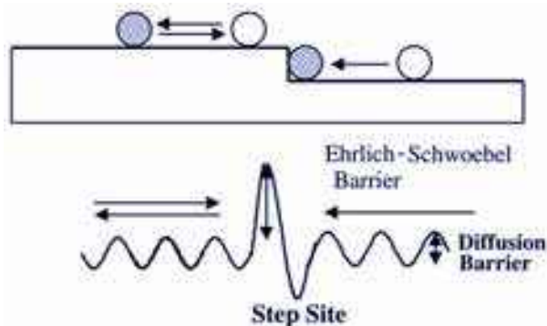
Figure 4.11: On a rigid lattice, admolecule diffusion over abrupt terrace steps is suppressed by the Ehrlich-Schwoebel barrier. An admolecule crossing over the step edge will (temporarily) be in a position nearly removed from the surface, which is energetically quite unfavorable. This creates a potential barrier that impedes such crossings. The step structure will become less rigid in the presence of surface premelting, however, which should substantially reduce the Ehrlich-Schwoebel barrier. Image from [2002He].
