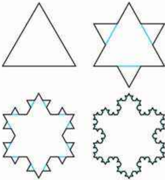
Figure 3.16: This sketch shows the construction of geometrical curve known as the Koch snowflake , first described by Swedish mathematician Helge von Koch in 1904. It is one of the earliest known examples of a fractal structure . As ever-smaller triangular sidebranches are attached ad infinitum , the area of the Koch snowflake converges to 8/5 times the area of the original triangle, while its perimeter length diverges to infinity. Consequently, the Koch snowflake has a finite area bounded by an infinitely long perimeter. Although this fractal structure bears some resemblance to a stellar dendrite snow crystal, there is little real connection between fractal mathematics and the physics of snow crystal formation.
