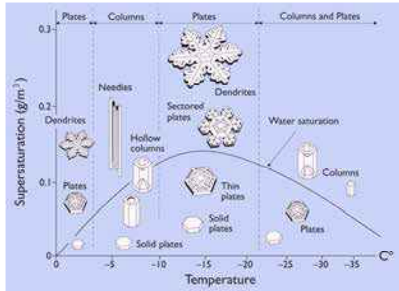
Figure 10.1: The snow crystal morphology diagram illustrates what types of crystals form in air as a function of temperature and water-vapor supersaturation. Note that this chart provides just a rough approximation of the different morphologies, plus it applies only if the growth conditions are constant in time. The “water saturation” line shows the supersaturation found in a dense cloud of liquid water droplets.
