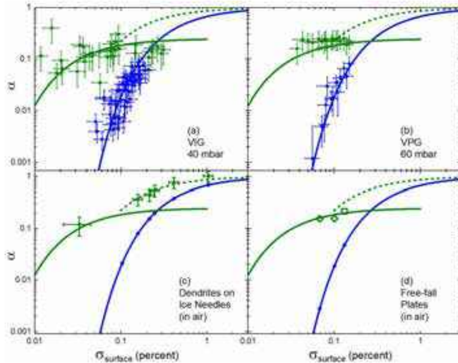
Figure 4.24: A collection of snow-crystal growth data obtained at a fixed temperature of -2^{\circ}\text{C} [2020Lib]. (a) Data from the VIG experiment at low background pressure, showing good agreement with the CAK model. (b) Similar data from the VPG experiment, confirming the earlier VIG results and the CAK model. (c) Observations of ice crystals growing on the ends of electric ice needles, analyzed using the witness-surface method on the basal facets. These data show rapid prism growth at high supersaturations, in agreement with the SDAK-2 phenomenon in the CAK model. (d) Additional data from a free-fall growth chamber, again analyzed using the witness-surface method. Although the overall phenomenology at -2^{\circ}\text{C} is not as rich as at -5^{\circ}\text{C} , the data show quite good agreement with the CAK model on all fronts.
