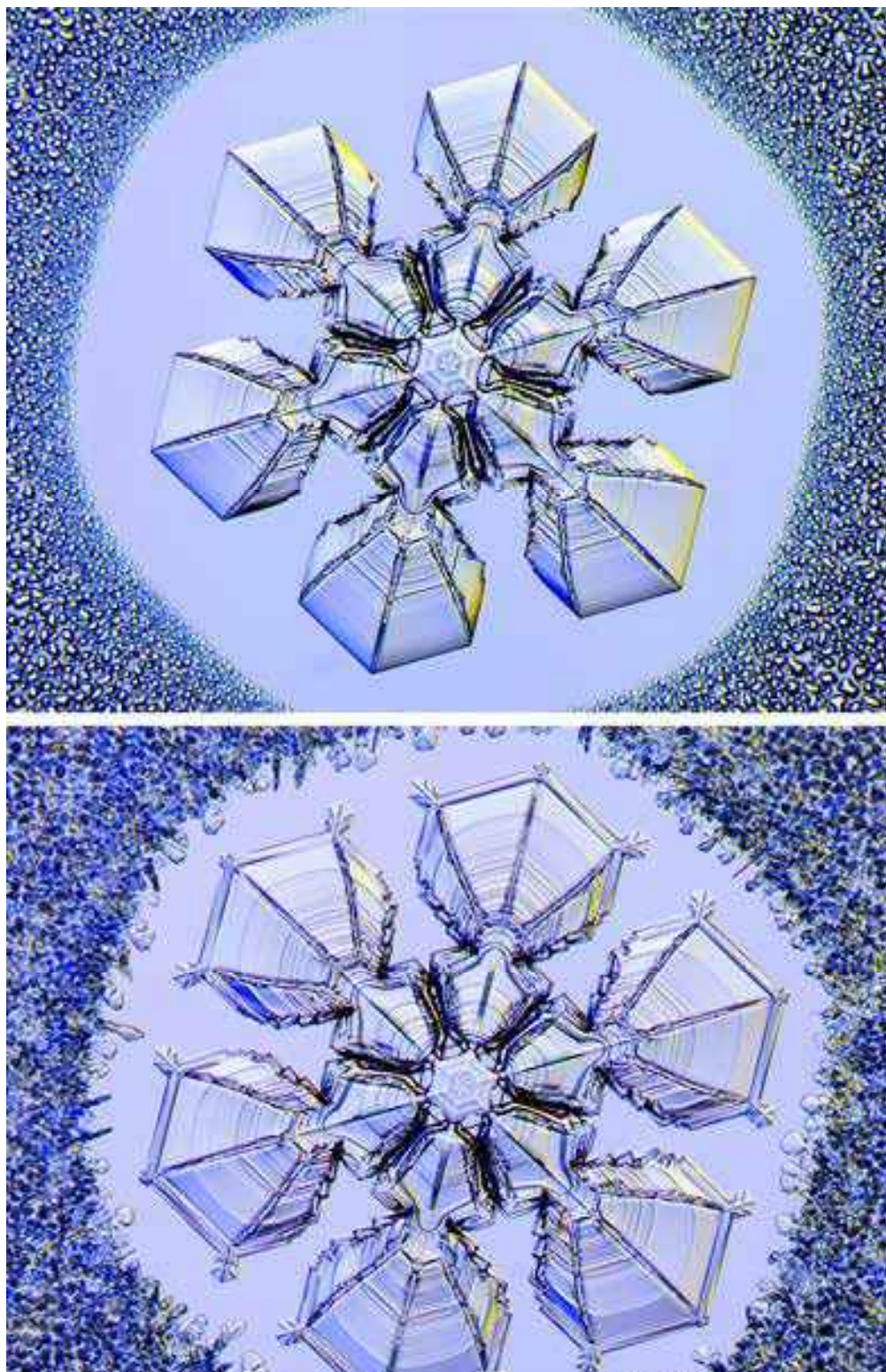
Figure 9.41: (Above and facing page) In these sets of images, the top photos show PoP crystals surrounded by fields of water droplets, taken soon before the droplets froze. The lower images show further development of the crystals, now framed by frost, after the air flow was substantially increased to boost the supersaturation.
