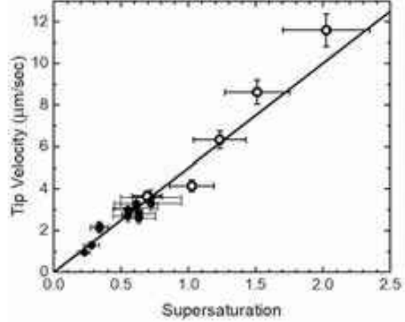
Figure 3.24: Measurements of the tip velocity of fernlike free dendrites growing near -15 C as a function of the far-away supersaturation. The data indicate a linear relationship between these variables, and the line shows v_{tip} = 5\sigma_{far} \mu\text{m/sec} . This supports the theoretical expectation that attachment kinetics provides the dominant selection perturbation in solvability theory for the case of snow-crystal free dendrite growth. (The data are from [2002Lib] with additional later measurements added to the plot.)
