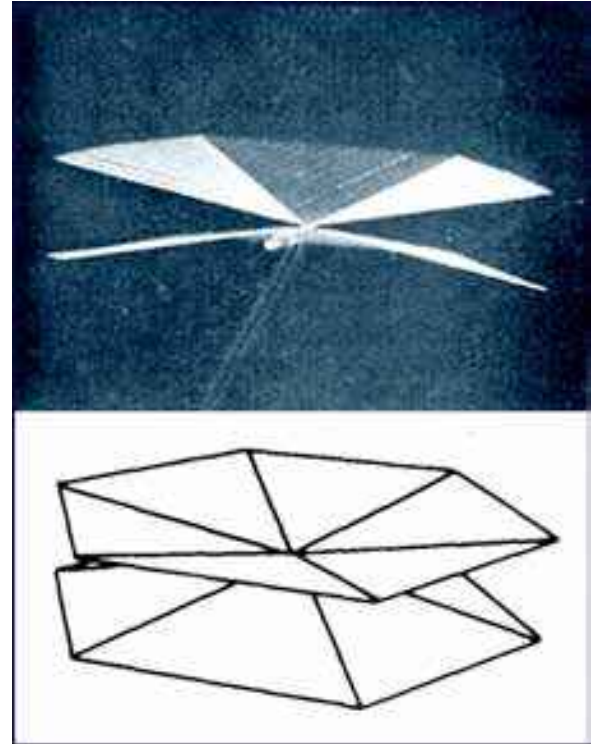
Figure 12.6: This unusual ice structure, formed at -5.2\text{ C} supercooling, consists of plate-like dendrites where the sidebranches have fused together into nearly solid plates [1965Mac]. The dual-plate structure is somewhat analogous to the double-plate snow crystals described in Chapter 10. In both cases, the overall double-plate morphology reflects the full history of the growth and boundary conditions, particularly at early times.
