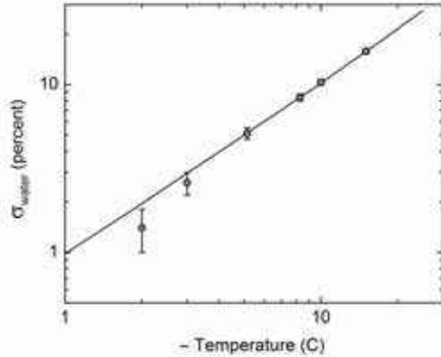
Figure 7.6: Measurements of \sigma_{\text{water}} at the substrate, as determined by the temperature difference \Delta T_{\text{stable}} at which water droplets are stable. The line is not a fit to the data, but shows the theoretical expectation with no adjustable parameters.
