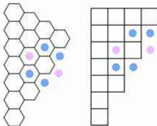
Figure 5.28: This diagram shows the 1/12^{\text{th}} slice of horizontal space needed to model a symmetrical snow crystal. Reflection boundary conditions apply on the two long edges, and colored dots illustrate some reflected pixels on the “ragged” edge. The short upper edge is the far-away boundary of the model.
