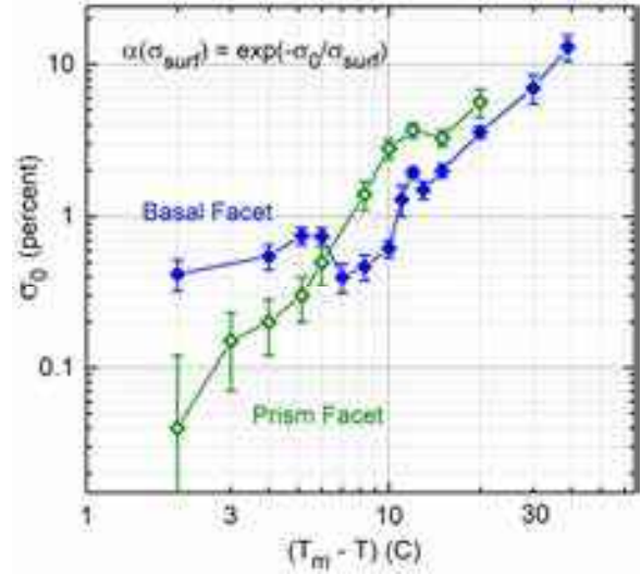
Figure 7.19: A reanalysis of the data in Figure 7.18, now assuming A = 1 for both the basal and prism facets, yields the measured \sigma_0(T) shown above. This analysis reflects a theoretical bias toward a purely nucleation-limited growth model with A = 1 , plus the suspicion of possible unmodeled systematic errors in the prism data at high temperatures.
