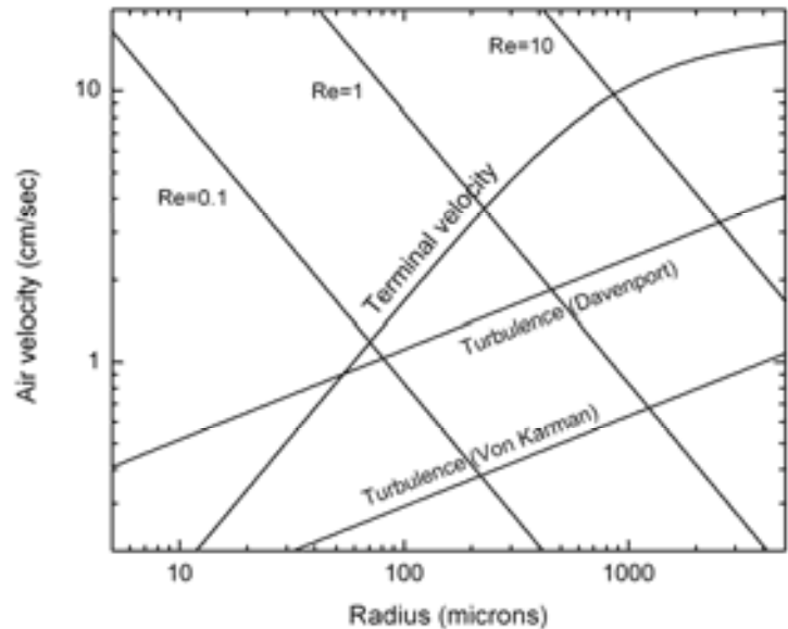
Figure 3.28: The terminal velocity curve on this plot shows the fall velocity of a 2- \mu m -thick snow crystal disk as a function of disk radius, while approximate scaling with disk thickness is given by Equations 3.48 and 3.49. The turbulence curves show two models of root-mean-squared air velocities when the average air speed is 1 m/sec. When R is large enough that the terminal velocity curve is above the turbulence curves, then gravity can align the crystal horizontally [2009Lib3].
