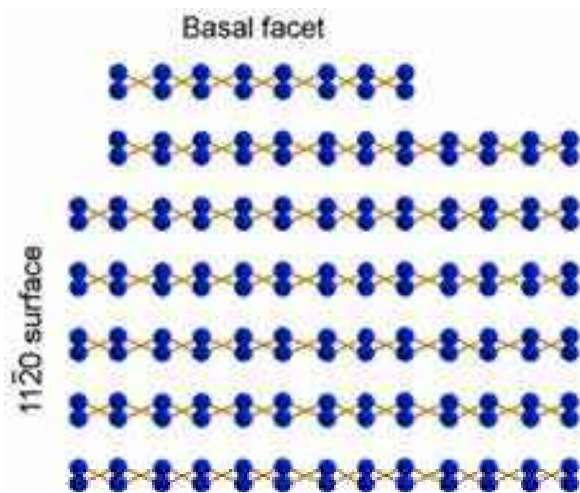
Figure 2.11: A projection of the ice Ih lattice looking along the [1010] direction, showing basal and (11\bar{2}0) surfaces and terrace steps. From this perspective, it is easy to see why the basal terraces are sometimes called molecular bilayers.
