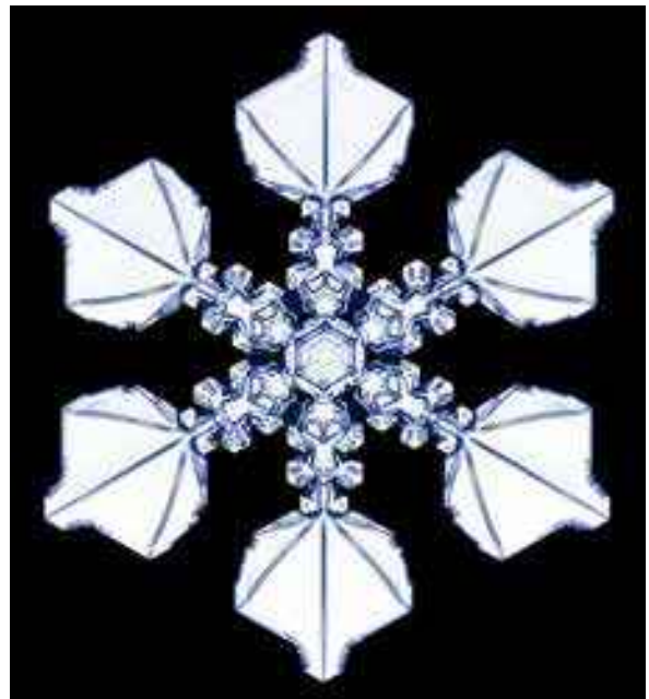
Figure 9.9: Setting the background black in Figure 9.8 yields this image, looking similar to snow crystal photographs taken by Wilson Bentley (see Chapter 1).
