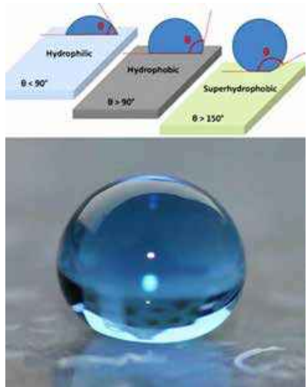
Figure 6.13: A superhydrophobic substrate surface could greatly reduce unwanted substrate interactions. (Images from [2016Lui] and mandegar.info.)
