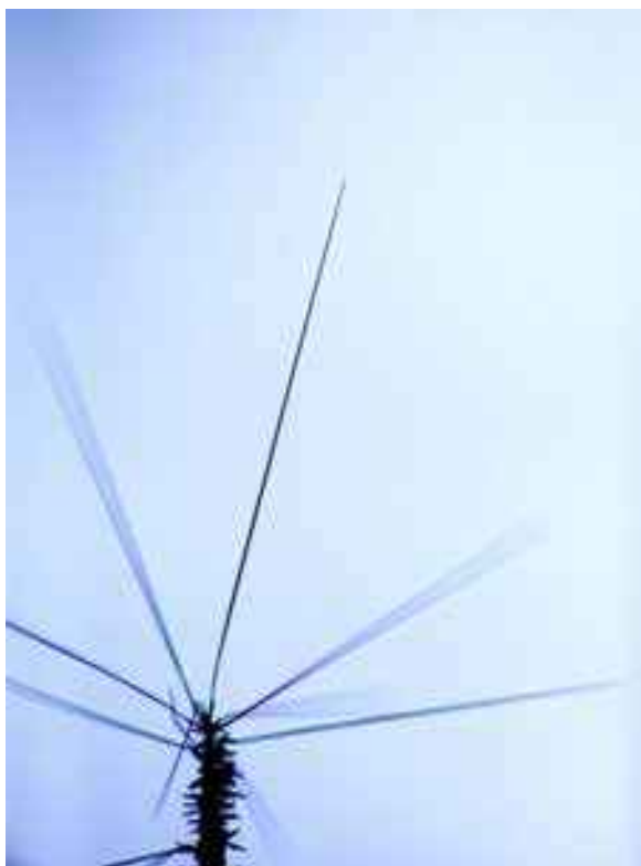
Figure 8.1. A set of slender “electric” ice needles (e-needles) growing on the end of a frost-covered wire. The e-needle centered in the image is about 3 mm in length. The needles formed when +2000 volts was applied to the frost-covered wire at the bottom of the photo, which was simultaneously exposed to highly supersaturated air at a temperature near -6 C. The e-needle phenomenon is the result of an electrically induced growth instability.
