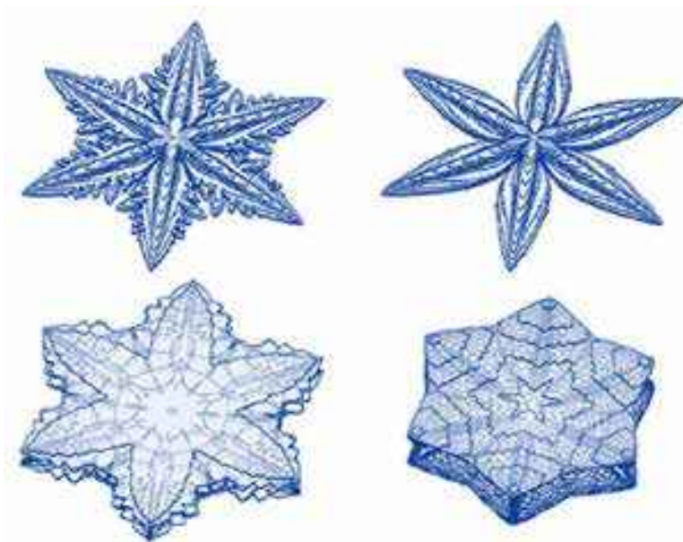
Figure 5.13: A few representative 3D snow crystal models created by Kelly and Boyer [2014Kel], using CA rules derived from physically realistic calculations. More examples can be found at the front of this chapter. Again, these models exhibit several morphological features found in real snow crystals.
