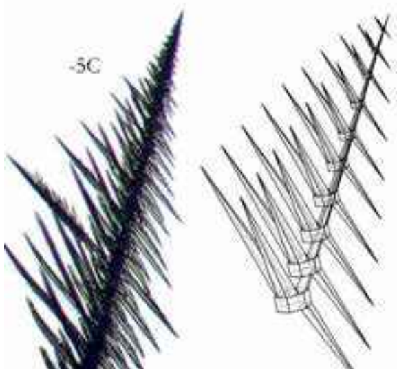
Figure 6.31: “Fishbone” dendritic snow crystals form at temperatures near -5\text{ C} in highly supersaturated air, such as in Figure 6.30. They grow readily in snow-crystal diffusion chambers, but are not found in nature. The sketch on the right illustrates their overall structure, with hexagonal prisms showing the crystal axes [2009Lib1].
