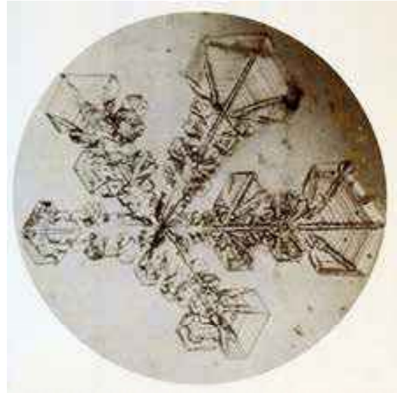
Figure 1.22: The world's first synthetic snow crystal, grown by Ukichiro Nakaya on March 12, 1936 [1954Nak].
