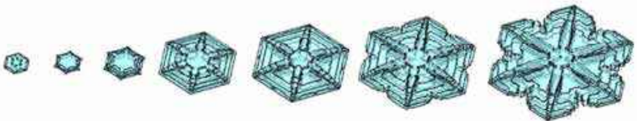
Figure 3.44: (Below) Another 3D numerical model showing clear ridge structures on slightly convex basal surfaces. Image from [2009Gra].
