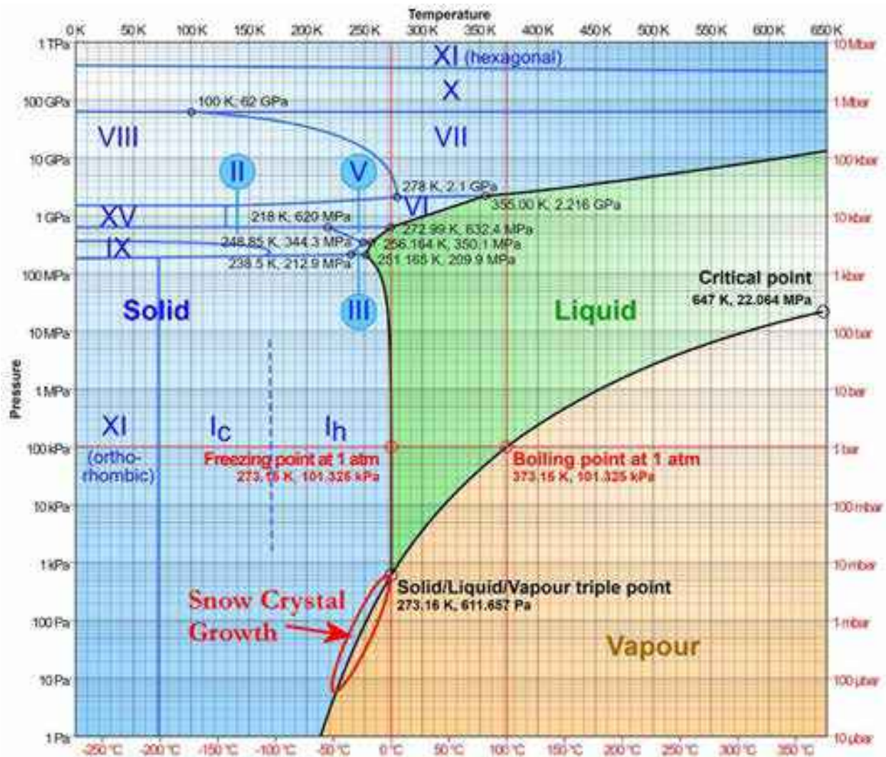
Figure 2.1: The phase diagram of water as a function of temperature and pressure. Snow crystal growth occurs on the ice/vapor boundary below the triple point, mostly at temperatures between 0 C and -40 C. Note that most of the known phases of ice exist only at extremely high pressures. Image from https://en.wikipedia.org/wiki/Ice .
