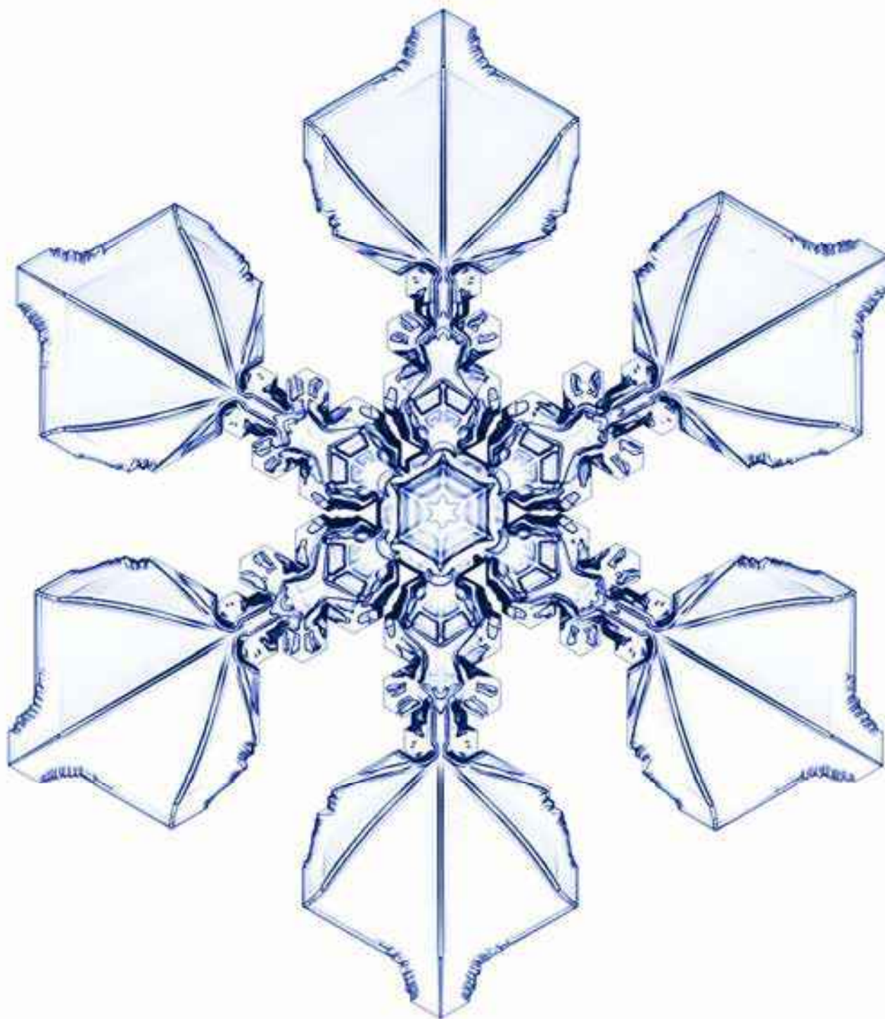
Figure 9.8: Plain white-light illumination from behind yields a particularly high-resolution image, revealing exceptionally sharp facets and fine details in the surface structures. Five images were combined to make this image, using focus stacking to improve the resolution slightly. Minimal post-processing was applied, mainly just adjusting to background to full bright white and applying a slightly bluish hue to the image.
