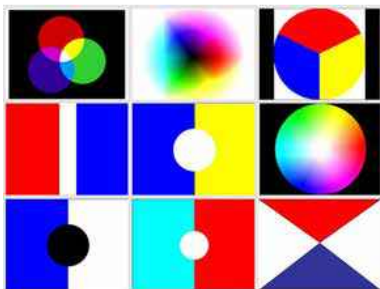
Figure 9.13: (Below) A sampling of nine color filters I have used for Rheinberg illumination of PoP snow crystals. A filter design using bright colors with abrupt transitions often yields images that exhibit rich shading and vibrant highlights.
