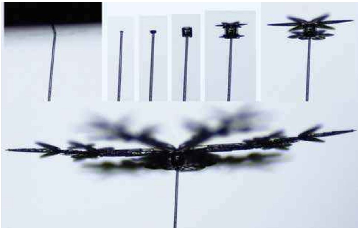
Figure 6.38: Growing an oriented snow crystal on a 20- \mu\text{m} -diameter capillary tube. In the upper left image, the basal surface of an ice crystal touches the tip of a water-filled capillary, freezing the water with the ice c-axis (nearly) collinear with the capillary axis. With the ice plate removed, the other images show subsequent development of the crystal in a diffusion chamber. The stellar snow crystal in the lower image measures 3 mm from tip to tip, but this crystal eventually grew to 12 mm from tip to tip. (Photos by the author.)
