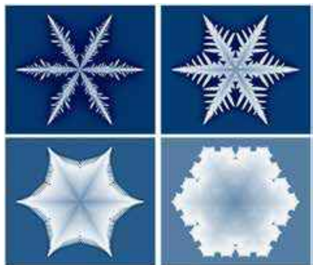
Figure 5.8: Several 2D cellular automata models of diffusion-limited growth on a six-fold symmetrical lattice, exhibiting faceted and branched structures [2005Rei].
