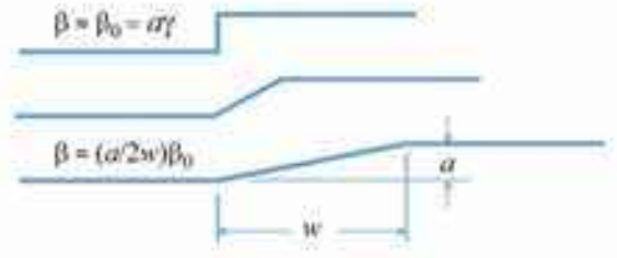
Figure 2.17: A simple geometrical model describing how surface relaxation reduces the terrace step energy. In this picture, the additional surface area added by a terrace step depends on the step width, and this additional surface area is taken to be the step energy.
