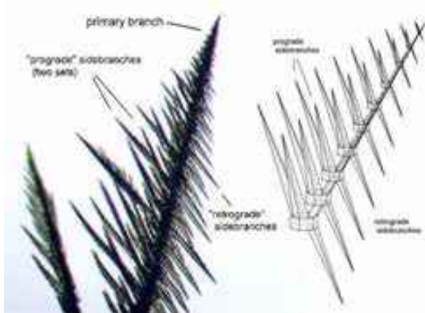
Figure 3.11: The sidebranch structure of a fishbone dendrite is more three-dimensional than a fernlike dendrite. This figure compares a photograph with a sketch that shows the orientations of the different sidebranches with respect to the ice crystal axes (defined by the hexagonal prisms in the sketch). Unlike fernlike dendrites, fishbone dendrites are clearly not confined to a flat growth plane.
