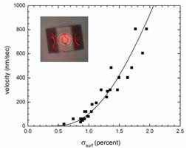
Figure 7.15: Sample measurements of the prism growth velocity as a function of supersaturation at the facet surface. Data points were taken at -15 C with a background air pressure of 20 mbar, using oscillations in the brightness of the laser spot to interferometrically measure the growth velocity [2013Lib]. The line shows v_n = \alpha v_{kin} \sigma_{surf} with \alpha(\sigma_{surf}) = \exp(-\sigma_0/\sigma_{surf}) and \sigma_0 = 3 percent. Note that the data fit this model well at growth velocities up to nearly 1 micron/second. The inset photo shows a test crystal being measured.
