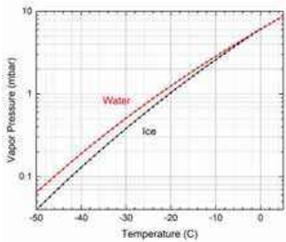
Figure 2.13: The vapor pressure of ice and supercooled water as a function of temperature. The points are measured values, and lines show the approximate Arrhenius models described in the text.
