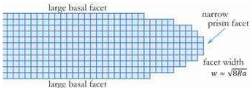
Figure 4.9: The shape of a thin hexagonal platelike crystal is largely defined by the growth of the basal and prism facets. While the basal facets are quite large, the six prism facets have widths w \approx \sqrt{8Ra} , where R is the radius of curvature of the edge and a is the molecular size. In many common circumstances, the attachment kinetics on these extremely narrow facets is markedly different from the attachment kinetics on large faceted surfaces.
