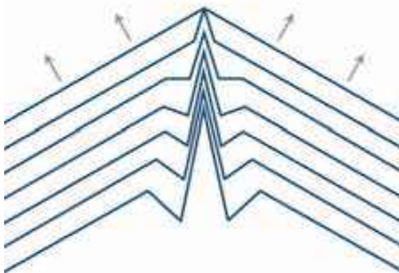
Figure 3.46: A sketch showing the development of a snow-crystal ridge flanked by two grooves on a convex basal surface. As the ridge structure develops, it depletes the water-vapor supply in its proximity. This suppresses the advancements of steps near the ridge, thereby creating grooves.
