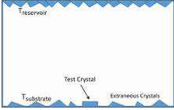
Figure 3.18: An example of a poorly designed experimental set-up. As described in the text, the boundary conditions are so ill-defined that it is essentially impossible to do a quantitative analysis of the growth of the test crystal. Removing the extraneous crystals largely remedies this situation, but only if all of them are removed.
