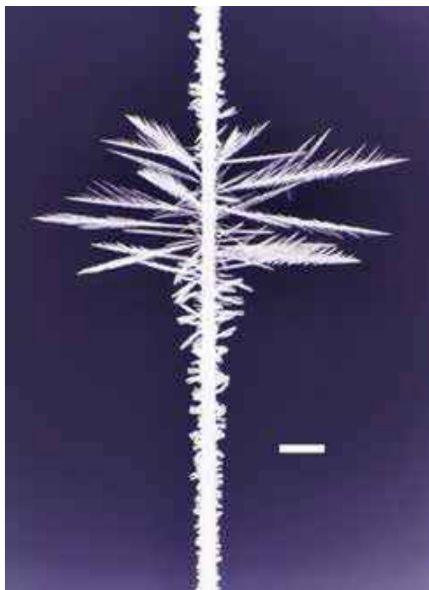
Figure 8.13. An image showing ice crystals growing on a segment of 200-micron-diameter nylon fishing line hanging in the center of DC1. The scale bar is 1 mm long, and the crystal growing time was 19 minutes. [2014Lib]. The crystal morphology is strongly temperature dependent, with the fast-growing “fishbone” dendrites appearing near -5^{\circ}\text{C} . The best wire tip location for producing c-axis electric needles is just below the fishbone peak, where the temperature is near -6^{\circ}\text{C} . Hollow columnar crystals appear at this position.
