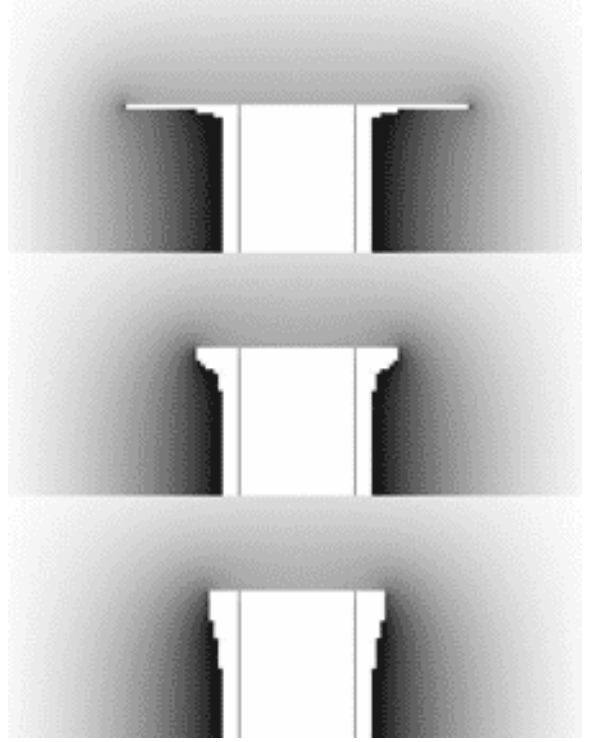
Figure 2.18: Three examples modeling the growth of a thin snow-crystal plate on the end of a columnar crystal (here shown in side view) [2013Lib1]. Setting d_{sv} = 0 (top model) yields an unrealistic 0.1-micron-thick plate growing out from the column when the applied supersaturation is low. Using a realistic value of d_{sv} (bottom model), the plate-growth is suppressed. Without including the Gibbs-Thomson effect, snow-crystal models would not give physically realistic results at exceedingly low supersaturations. In many environmental circumstances, however, the Gibbs-Thomson effect is so small that it is essentially negligible.
