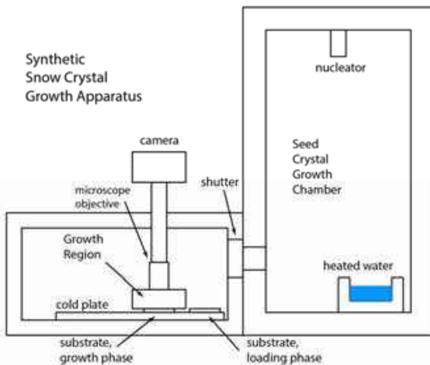
Figure 9.3: (Right) The apparatus used to grow and photograph PoP snow crystals. Small, freely falling ice prisms in the seed-crystal chamber first pass through a shutter, and some of them fall randomly onto a waiting sapphire substrate (loading phase). The substrate is then moved to the growth region for subsequent PoP crystal growth.
