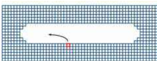
Figure 3.40: Even if the equilibrium shape of an enclosed bubble is spherical, a faceted bubble may evolve exceedingly slowly toward that final form. It is difficult to remove molecules from a fully faceted surface (red), and this presents a strong hole-nucleation barrier that can greatly slow equilibration. For this reason, even very thin bubbles in plate-like crystals can retain their shape for long periods of time.
