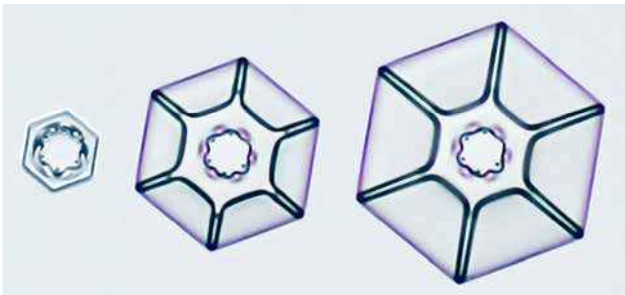
Figure 9.14: Starting with an initial seed crystal (left), a Plate-on-Pedestal geometry develops. In this example, the initial hexagon grew out slightly before the upper plate formed. The odd central patterning reflects some surface structure on the bottom basal surface that became trapped by contact with the substrate. In contrast, the top basal surface soon grew into a nearly perfect faceted form, filling in any surface structure that had been present on the seed crystal. The seed crystal shown measures 90 \mu\text{m} from facet-to-facet, while the final thin plate measures 300 \mu\text{m} .
