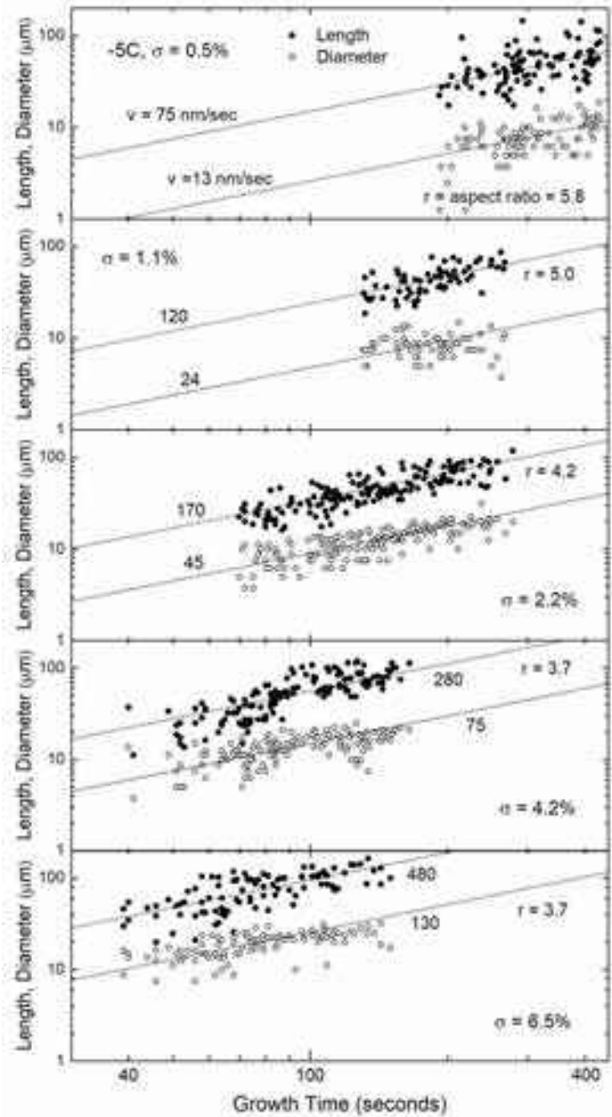
Figure 7.22: Free-fall growth data at -5 C from [2009Lib], showing crystal sizes as a function of fall times for several different supersaturations (here \sigma = \sigma_\infty , which is generally not equal to \sigma_{surf} ). Each pair of points (length and diameter) represent one observed crystal. Lines show constant-velocity trajectories, and the aspect ratio is the ratio of these velocities. Note that the aspect ratio tends toward unity with increasing supersaturation.
