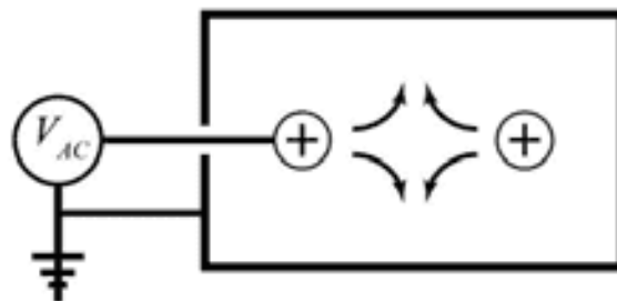
Figure 6.36: A single ring electrode (seen here from the side, labeled \oplus ) inside a conducting box creates a 3D quadrupolar electric field near its center, shown by the arrows. Applying a sinusoidal voltage to the ring creates electrodynamic forces that push charged particles toward the ring center. (Image from [2018Lib].)
