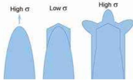
Figure 3.55: Induced Sidebranching. When the supersaturation is sufficiently high near -15 C (left), \alpha_{prism} will be near unity at the tip of a growing dendrite, yielding a rounded shape with little prism faceting. Upon lowering the supersaturation (middle), \alpha_{prism} is reduced and the tip becomes faceted. Increasing the supersaturation once again (right), branches sprout from the three exposed corners of the faceted tip. One branch continues in the primary direction while the other two become sidebranches. Looking at the whole crystal, this mechanism creates a coordinated set of sidebranches on all six primary branches. Induced sidebranching is thus responsible for much of the complex symmetry seen in stellar dendrite snow crystals.
