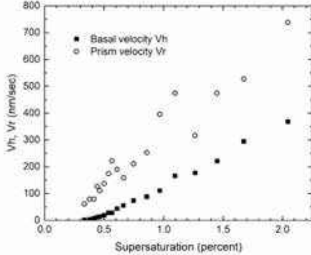
Figure 7.12: The growth sequence in Figure 7.11 after being converted to velocities versus supersaturation \sigma_{bottom} just above the substrate surface. Note that \sigma_{bottom} is not generally equal to the supersaturation \sigma_{surf} at the crystal surface.
