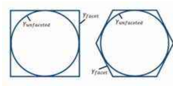
Figure 2.19: Basic limits on equilibrium shapes in 2D. The square shape has a lower surface energy than its inscribed circle if \gamma_{facet} < (\pi/4)\gamma_{unfaceted} = 0.79\gamma_{unfaceted} , and the hexagon has a lower surface energy if \gamma_{facet} < (\pi\sqrt{3}/6)\gamma_{unfaceted} = 0.91\gamma_{unfaceted} .
