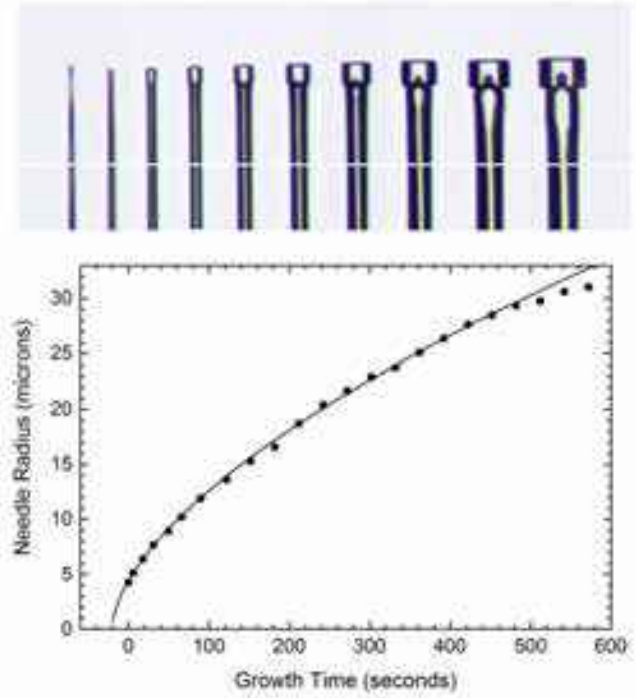
Figure 8.17. Example observations at -2 C of the growth of a single electric ice needle after being transported into DC2. The composite image shows the needle at several different times, and the graph shows measurements of the needle radius as a function of time, measured at the position of the white horizontal line in the image, which is approximately 100 \mu\text{m} below the needle tip [2016Lib].
