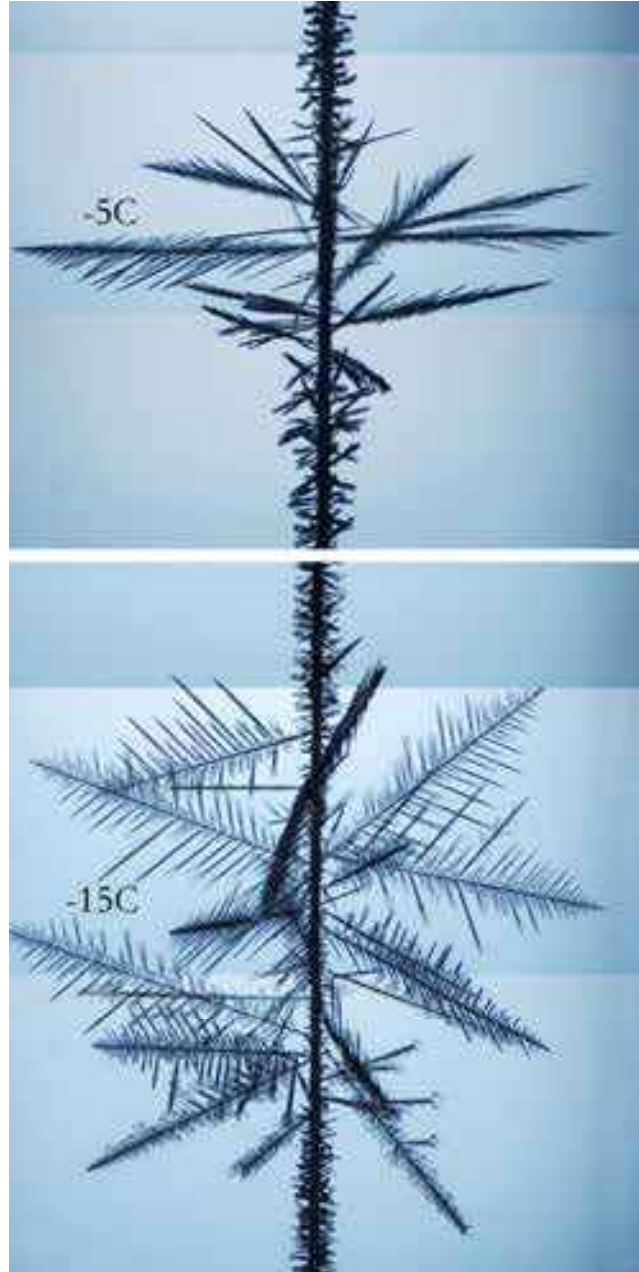
Figure 6.30: Higher resolution images of a string of snow crystals similar to that shown in Figure 6.29. The cluster at -5^{\circ}\text{C} is made of “fishbone” dendrites (see Figure 6.31), while the cluster at -15^{\circ}\text{C} is made from individual branches of fernlike stellar dendrites. As soon as these fast-growing crystals extend out away from the filament, they tend to shield water vapor from reaching smaller crystals nearer the filament, stunting their growth.
