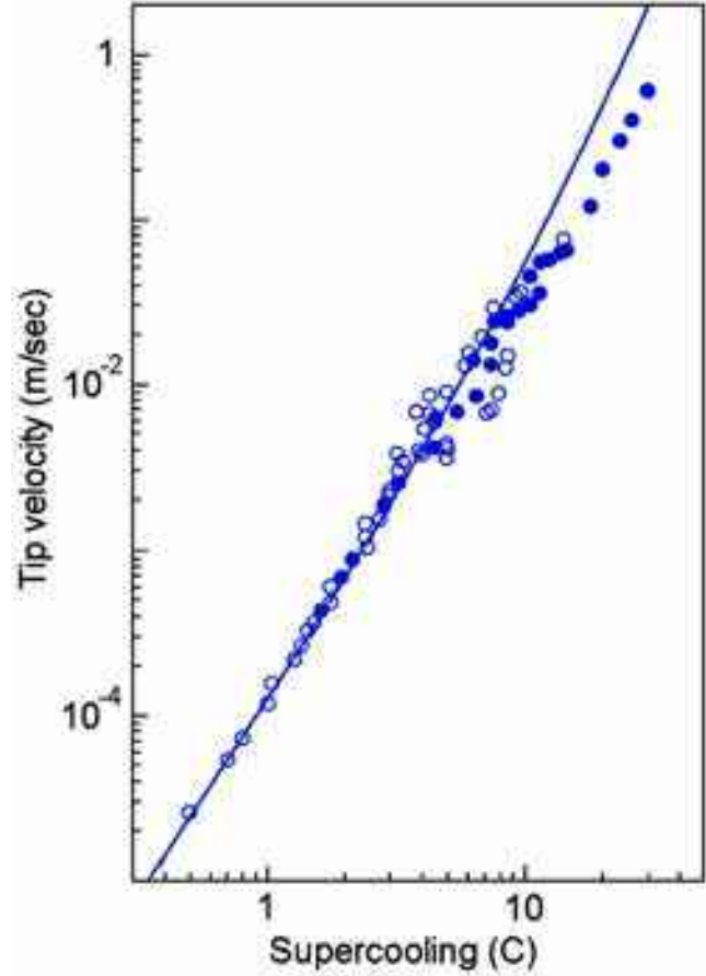
Figure 12.11: Measurements of the free dendrite tip velocity v_{tip} for ice growing from liquid water as a function of the bath supercooling. The line shows a calculation using a surface-energy-dominated version (neglecting attachment kinetics) of solvability theory. Figure adapted from [2005Shi].
