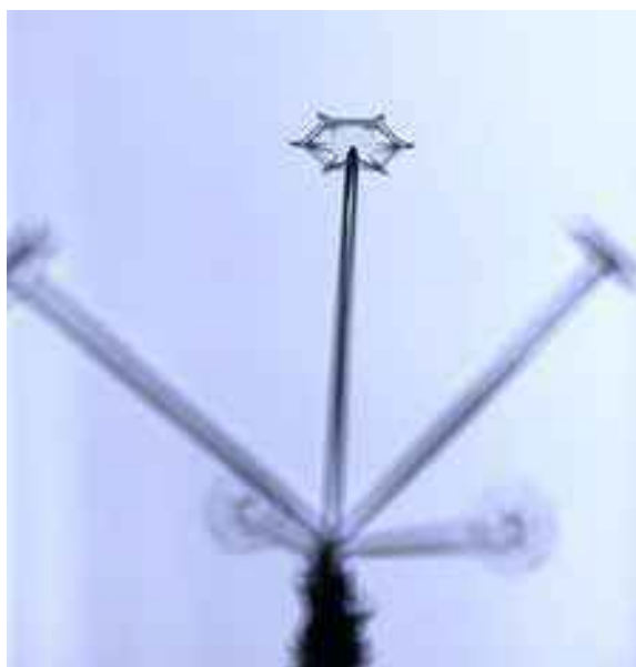
Figure 8.2. Thin, plate-like snow crystals growing on the ends of c-axis electric ice needles. This example illustrates how e-needles can be used to cleanly support isolated snow crystals as they growth and develop.
