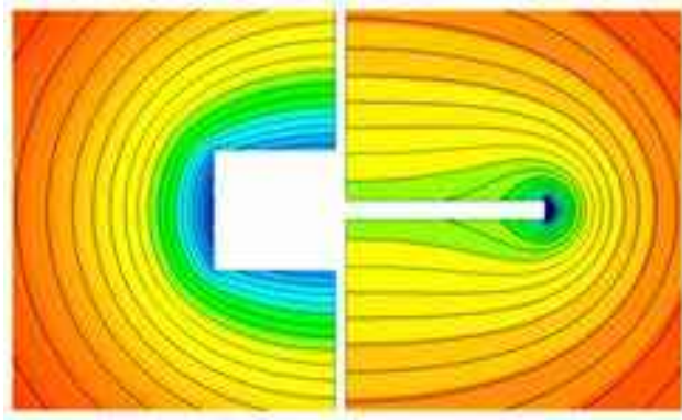
Figure 3.29: Calculated contour plots of supersaturation levels around two growing ice crystals, shown here in (r,z) coordinates. Around a blocky crystal (left), the supersaturation is highest near the corners of the faceted prism, a phenomenon called the Berg effect. Around a thin-plate crystal, the contour lines are tightly bunched at the plate edge, and the supersaturation is highest at the center of the basal facets. The model on the left assumed \alpha_{basal} \approx \alpha_{prism} < 1 , while the model on the right assumed \alpha_{basal} \ll \alpha_{prism} .
