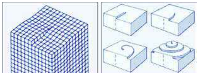
Figure 4.25: Left: The lattice structure of a screw dislocation. Right: As the dislocation edge grows from ad molecule attachment, it creates a spiral pattern that can propagate indefinitely, yielding growth in the absence of additional terrace nucleation.
