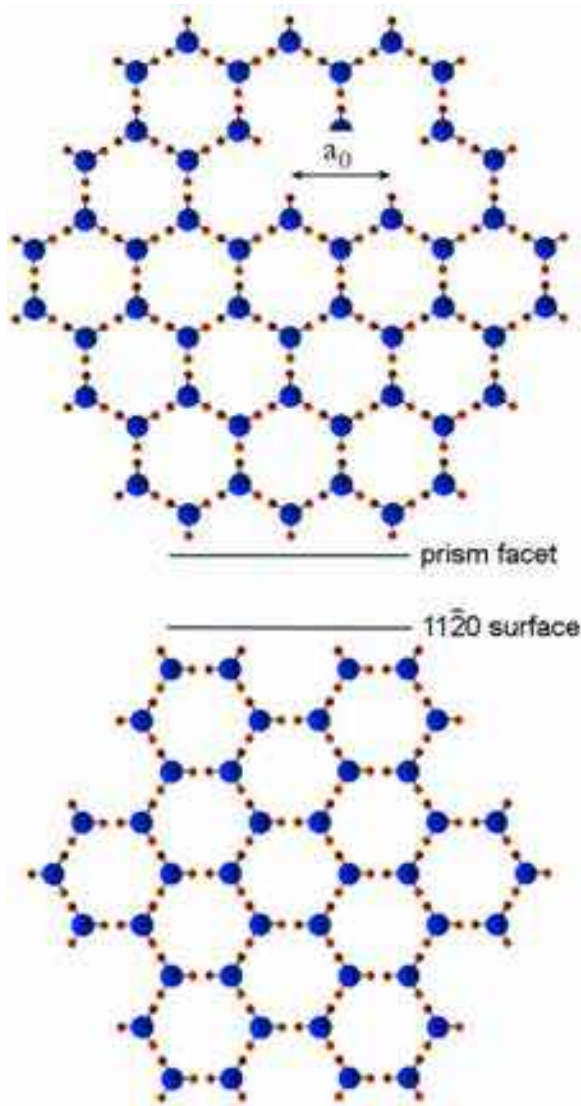
Figure 2.7: Two projections of the ice Ih lattice looking down along the [0001] direction (perpendicular to a basal facet). A prism \{1010\} facet and a \{11\bar{2}0\} surface are labeled. (The latter is sometimes called a secondary prism surface, although it does not exhibit any known faceting.)
