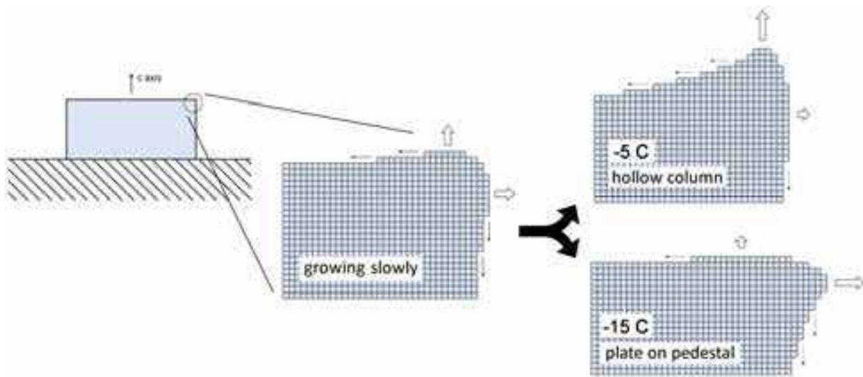
Figure 4.15: The Edge-Sharpening Instability (ESI). This sketch illustrates how the SDAK phenomenon can bring about an edge-sharpening growth instability on either the basal or prism facets. As described in detail in the text, as the uppermost terrace becomes narrower, the attachment coefficient on that terrace can increase via the SDAK mechanism, thus increasing the growth and further narrowing the upper terrace. This brings about a positive feedback effect, and thus a growth instability, that promotes the formation of sharp edges, either as hollow columns (upper right sketch) or thin plates (lower right sketch). In the comprehensive attachment kinetics (CAK) model presented in this chapter, the ESI mechanism in air is largely responsible for the formation of thin plates at -15 C and hollow columns at -5 C.
