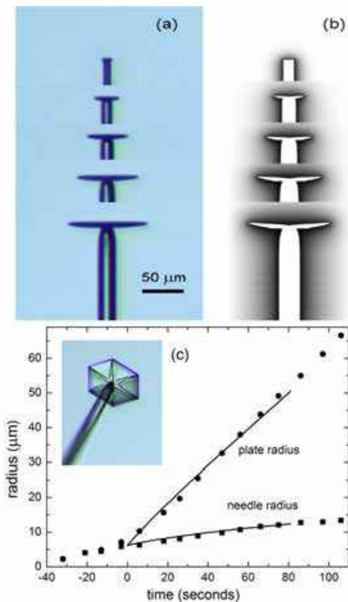
Figure 8.4. These figures show one example of a quantitative comparison of laboratory and computational snow crystals [2008Lib, 2013Lib]. (a) A composite image made from five photographs showing the growth of a plate-like snow crystal on the end of an electric ice needle, viewed from the side. (b) A computational model of the same crystal, showing the water-vapor diffusion field around the crystal. (c) A quantitative comparison of experimental data (points) and the computational model (lines). The inset photo shows the crystal in (a) from a different angle.
