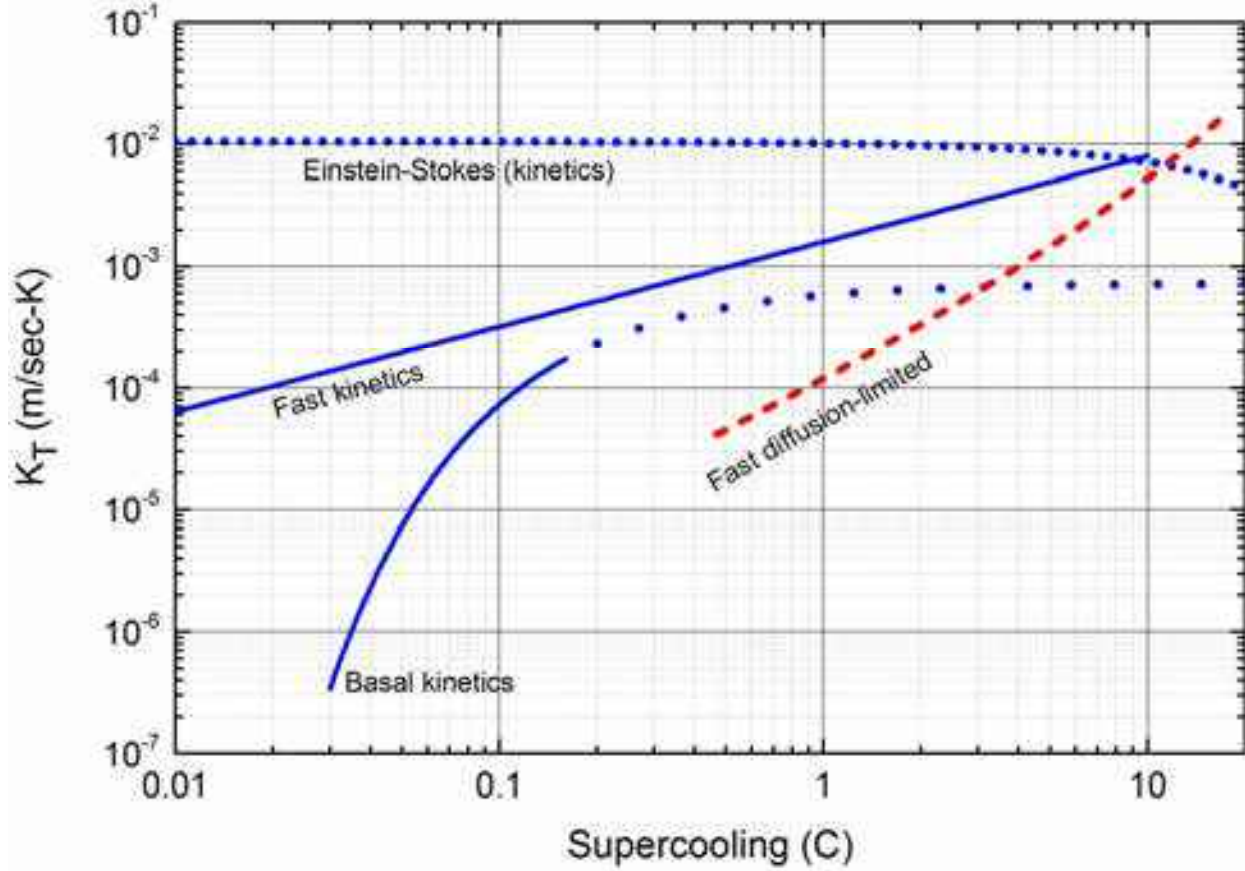
Figure 12.9: The blue curves in this plot show the kinetic coefficient K_T(\Delta T_{surf}) for ice growth from liquid water for the basal facet (labeled basal kinetics) [2014Lib] and for fast-growing unfaceted surfaces (fast kinetics) [2017Lib]. The thick portion of the basal line derives from ice growth data, while the dotted portion is extrapolated to larger \Delta T_{surf} . The remaining blue short-dotted curve shows K_T from Einstein-Stokes theory [1996Sai, 2017Lib]. For comparison, the red dashed curve shows K_T(\Delta T_{bath}) for the tips of growing dendrites [2005Shi]. Note that the abscissa in this graph does double duty, equal to either \Delta T_{surf} (blue curves) or \Delta T_{bath} (red curve).
