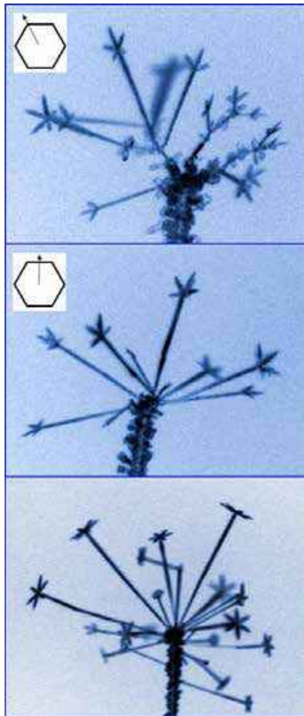
Figure 8.8. (Above right) Under different experimental conditions, e-needles can grow preferentially along the a-axis (top photo), the [1\bar{1}00] axis (middle photo), or the c-axis (bottom photo). In many conditions, e-needle growth is not along a well-defined crystalline axis but appears to be somewhat random and likely dependent on the orientation of the seed crystal from which the e-needle formed. In these photos, a period of e-needle growth was followed by a period of normal growth, during which there was no applied voltage. The orientation of the e-needle could then be determined by the orientation of the subsequent normal growth.
