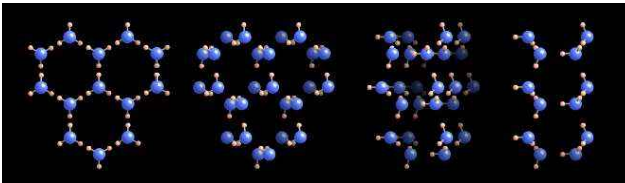
Figure 2.2: A molecular model of the ice Ih crystal rotated by 0, 18, 72, and 90 degrees about the [01\bar{1}0] axis. The large blue spheres represent oxygen atoms, and the smaller spheres represent hydrogen atoms. The first image is looking down the c-axis, revealing the hexagonal lattice structure.
