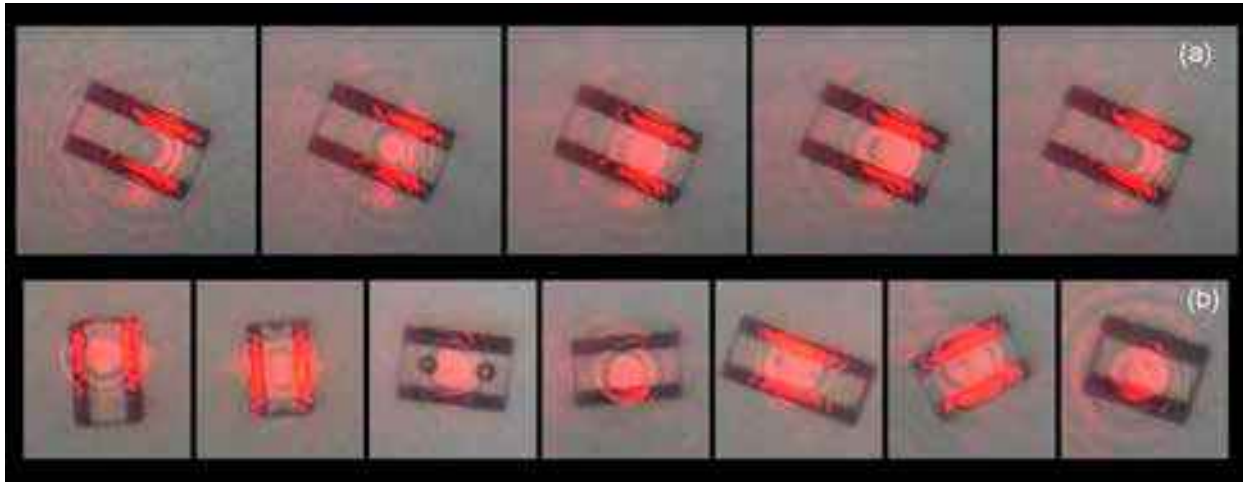
Figure 7.10: (a) Several images of a columnar ice crystal showing the interference of two reflections from an incident Helium-Neon laser beam, one from the substrate/ice interface and one from the ice/vacuum interface. As the crystal grew (left to right) the spot brightness oscillates from dim (first image) to bright (middle image) and back to dim (last image). (b) Snapshots from several other example crystals.
