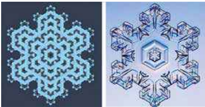
Figure 5.1: A Packard snowflake (left), generated using simple nearest-neighbor rules in a cellular automaton, compared to a photograph of a natural snowflake (right). Although there are obvious structural similarities between the two images, the model has little basis in the physical processes underlying snow crystal growth. (Image adapted from [2008Gra].)
