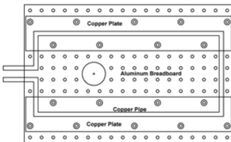
Figure 6.5: A temperature-controlled aluminum breadboard, complete with an array of tapped holes, can serve as versatile starting point for many snow-crystal growth chambers. Cold fluid from a recirculating chiller flows through the copper pipe to cool the breadboard.
