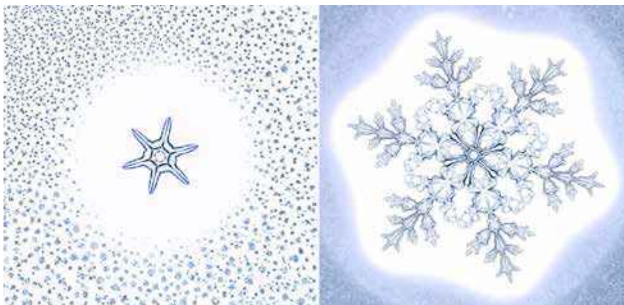
Figure 9.16: (Below) At high magnification (left), one can see individual droplets that recently nucleated on the surface in this photo. At lower magnification (right), the droplets take on the appearance of a continuous fog. In this case, the \sigma \approx \sigma_{water} contour is not circular, but follows the overall shape of the PoP crystal.
