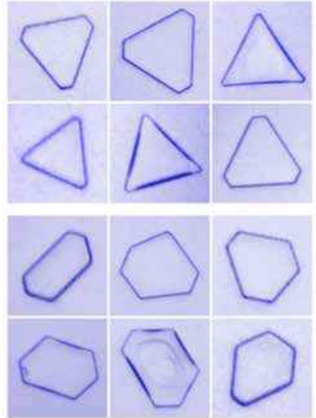
Figure 3.59: A selection of non-hexagonal plates observed in a free-fall growth chamber at -10^\circ\text{C} with \sigma_\infty \approx 1.4 percent. The top six images show crystals with an overall triangular symmetry, while the lower six images show crystals that are neither hexagonal nor triangular in appearance.
