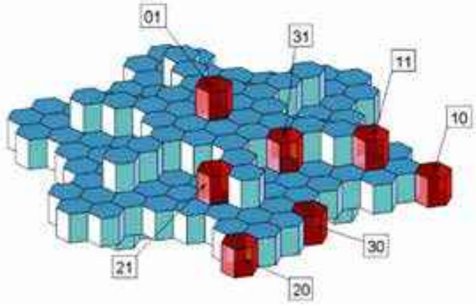
Figure 5.26: A 3D hexagonal grid of cells for a cellular-automata snow-crystal model. Here the blue-green pixels represent ice and the red pixels show a few representative boundary pixels. Vapor pixels are not shown. The boundary pixels are labeled with [HV] nearest-neighbor data, where H is the number of adjacent horizontal ice pixels and V is the number of adjacent vertical ice pixels. Image from [2009Gra].
