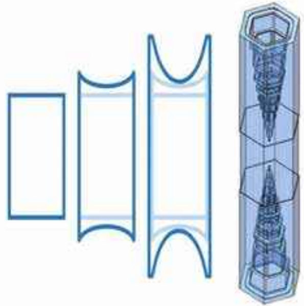
Figure 3.31: A schematic diagram illustrating the transition from solid columnar growth (first sketch, showing a side view of a solid column) to the formation of a hollow columnar snow crystal (third sketch) via the Mullins-Sekerka instability. The image on the right shows a 3D numerical simulation of hollow-column growth, from [2009Gra].
