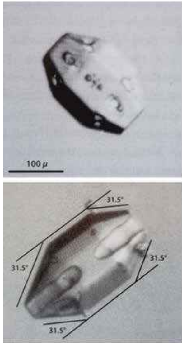
Figure 2.6: South-pole snow crystals displaying pyramidal facets. Image from [2006Tap].
