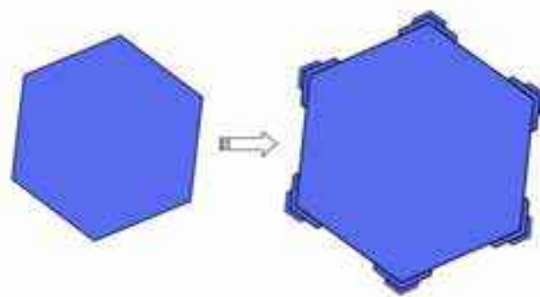
Figure 1.9: The six corners of a thin hexagonal plate stick out into the humid air around it. Water vapor condenses preferentially on the corners as a result, making them stick out even farther. This leads to a branching instability (described in Chapter 3) that causes six branches to sprout from the corners of the hexagon.
