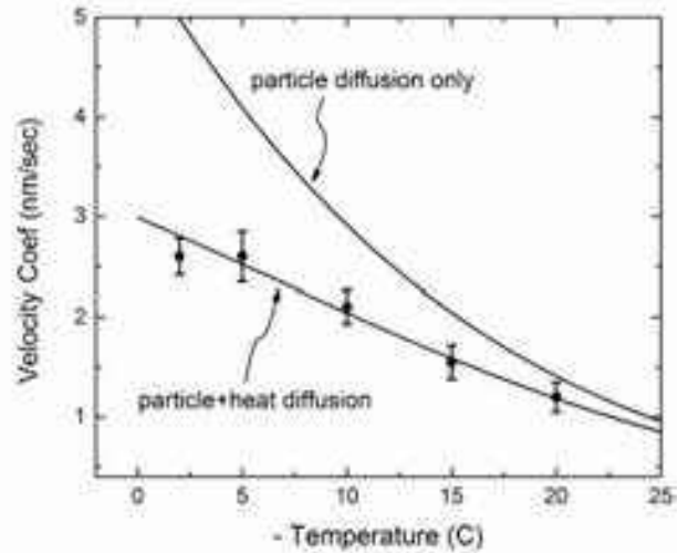
Figure 8.19. The cylindrical growth parameter A(T) extracted from the observations of needle growth in DC2, as a function of temperature. The top theory line is that predicted when the growth is limited entirely by particle diffusion (setting \chi_0 = 0 in the theory), while the lower theory curve includes both particle and heat diffusion. From [2016Lib].
