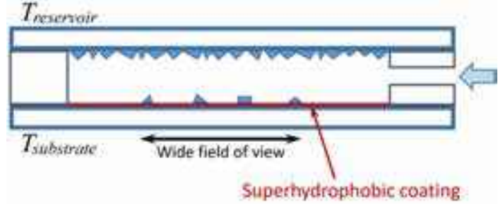
Figure 7.20: A possible experimental setup for observing the growth of small ice crystals on a superhydrophobic surface. Once the temperatures are stable, an expansion nucleator (blue arrow) injects a pulse of nano-ice-crystals into the test chamber, where some land on the coated sapphire substrate at random positions with random orientations, where a wide-field camera records their subsequent growth. All diffusion-related corrections are reduced when the crystal sizes are in the few-micron range, allowing accurate measurements even at fairly high gas pressures. The compact chamber size allows rapid turn-around between nucleation pulses for efficient experimental throughput.
