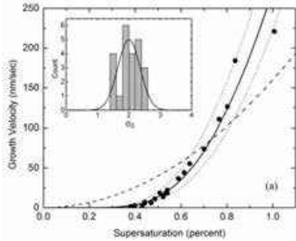
Figure 7.14: Sample corrected measurements showing the growth velocity of the basal surface of a single ice crystal as a function of \sigma_{surf} at -12 C, where data points were taken as the supersaturation was slowly increased. The line through the points gives the model v_{basal} = \alpha_{basal} v_{kin} \sigma_{surf} with \alpha_{basal}(\sigma_{surf}) = \exp(-\sigma_0/\sigma_{surf}) and \sigma_0 = 2.3 \pm 0.2\% . The dashed line shows a spiral-dislocation model with v \sim \sigma_{surf}^2 , which gives a poor fit to the data. The inset graph shows an unweighted histogram of measured \sigma_0 values for 23 crystals. A weighted fit to these data gives an estimated mean \langle \sigma_0 \rangle = 1.95 \pm 0.15\% .
