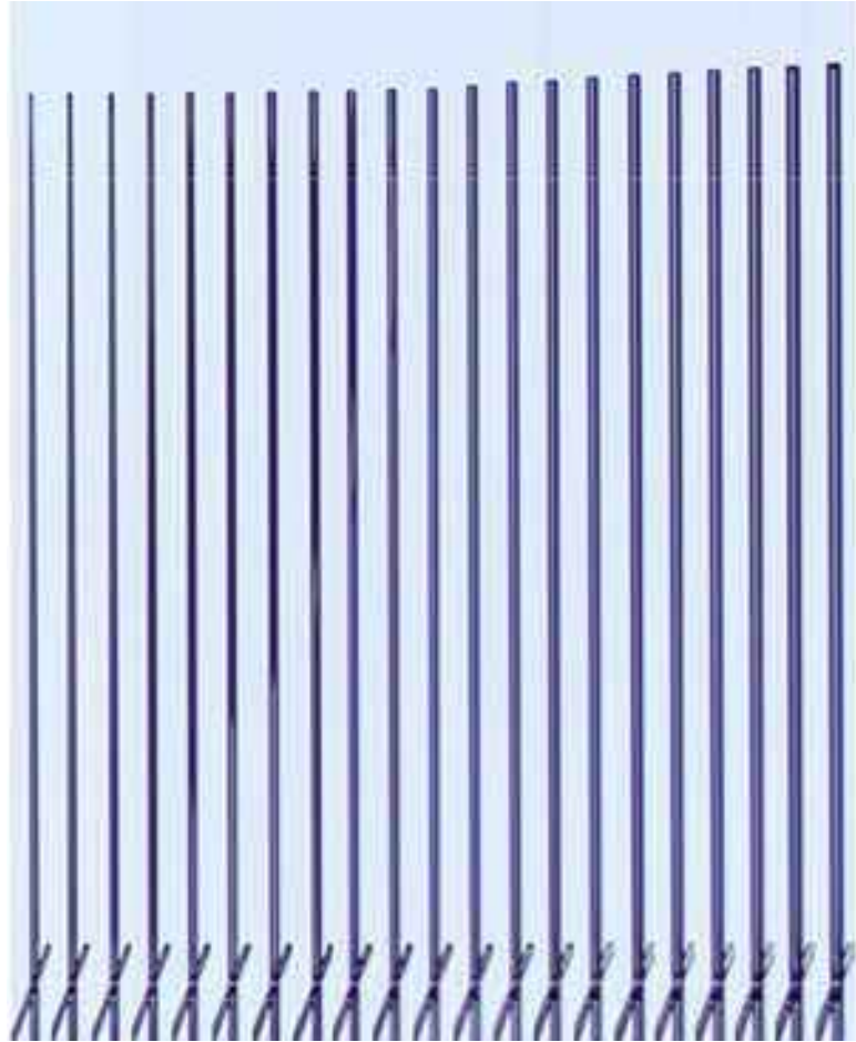
Figure 8.29. A composite image showing the growth of an e-needle at -5 C in a supersaturation of \sigma_\infty=1.8 percent. The near-constant structure near the base of the needle was used to align the images, allowing an accurate measurement of the axial growth rate. The radial growth was measured from direct imaging of the needle widths. Note how the axial growth is slow at first, but then transitions to a faster rate. The transition occurs just as the needle goes from slightly tapered to fully faceted.
