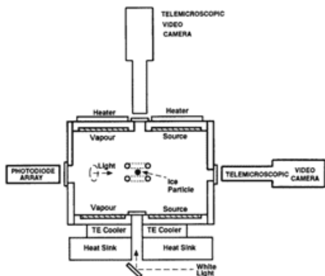
Figure 6.35: An electrodynamic levitation chamber for examining the growth of ice crystals [1999Swa]. A pair of ring electrodes driven with a high-voltage 60-Hz sinusoidal signal traps a charged ice particle, while the surrounding diffusion chamber creates a supersaturated environment. The closely spaced pair of rings creates a quadrupole electric field around its central point, much like that from a single ring ion trap illustrated in Figure 6.36.
