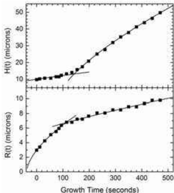
Figure 8.30. Measurements of R_{needle}(t) and H_{needle}(t) obtained from the image data in Figure 8.29. Here H_{needle}(t) is the needle length minus a constant offset. Lines were drawn through the data to guide the eye. The needle growth shows two distinct behaviors: 1) rapid radial growth and slow axial growth at times t < 130 seconds, and 2) slower radial growth and faster axial growth for t > 130 seconds. The images reveal that the transition occurred when the needle morphology changed from slightly tapered to fully faceted.
