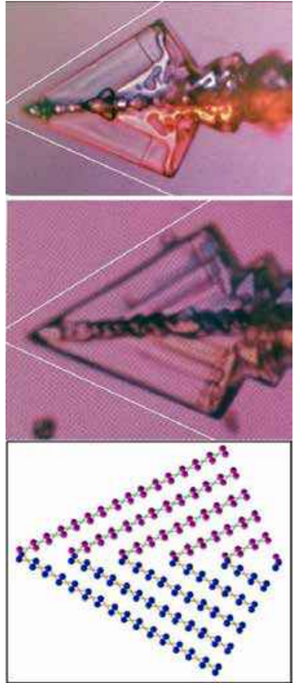
Figure 2.28 Arrowhead Twins Variant II. The top and middle photos above show two examples of this arrowhead-twin variant [2011Kik]. The lattice projection in the lower sketch is similar to that in Figure 2.26, giving a theoretical apex angle of 2 \tan^{-1}(c_0/3a_0) = 57.0 degrees. The pairs of white lines in the photos subtend this angle, showing good agreement with theory.
