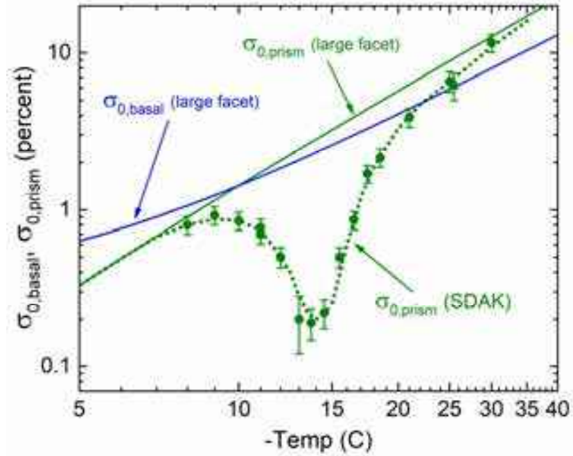
Figure 4.26: Measured values of \sigma_{0,prism,SDAK}(T) as a function of temperature (data points), revealing a substantial “SDAK dip” centered near -14 C [2020Lib1]. For comparison, the solid lines show the CAK model parameters \sigma_{0,basal} and \sigma_{0,prism} for broad-facet growth.
