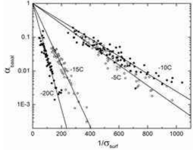
Figure 7.17: Experimental data showing the attachment coefficient \alpha_{\text{basal}} plotted as a function of 1/\sigma_{\text{surf}} , including measurements taken at four different temperatures. Plotted this way, data exhibiting a nucleation-limited growth behavior with \alpha_{\text{basal}}(\sigma_{\text{surf}}) = Ae^{-\sigma_0/\sigma_{\text{surf}}} appear as straight lines. The data at each temperature extrapolate to \alpha \approx 1 at large \sigma_{\text{surf}} , indicating rapid kinetics in the absence of a nucleation barrier. The values of \sigma_0 at different temperatures can be extracted from the slopes of the lines [2013Lib, 2017Lib].
