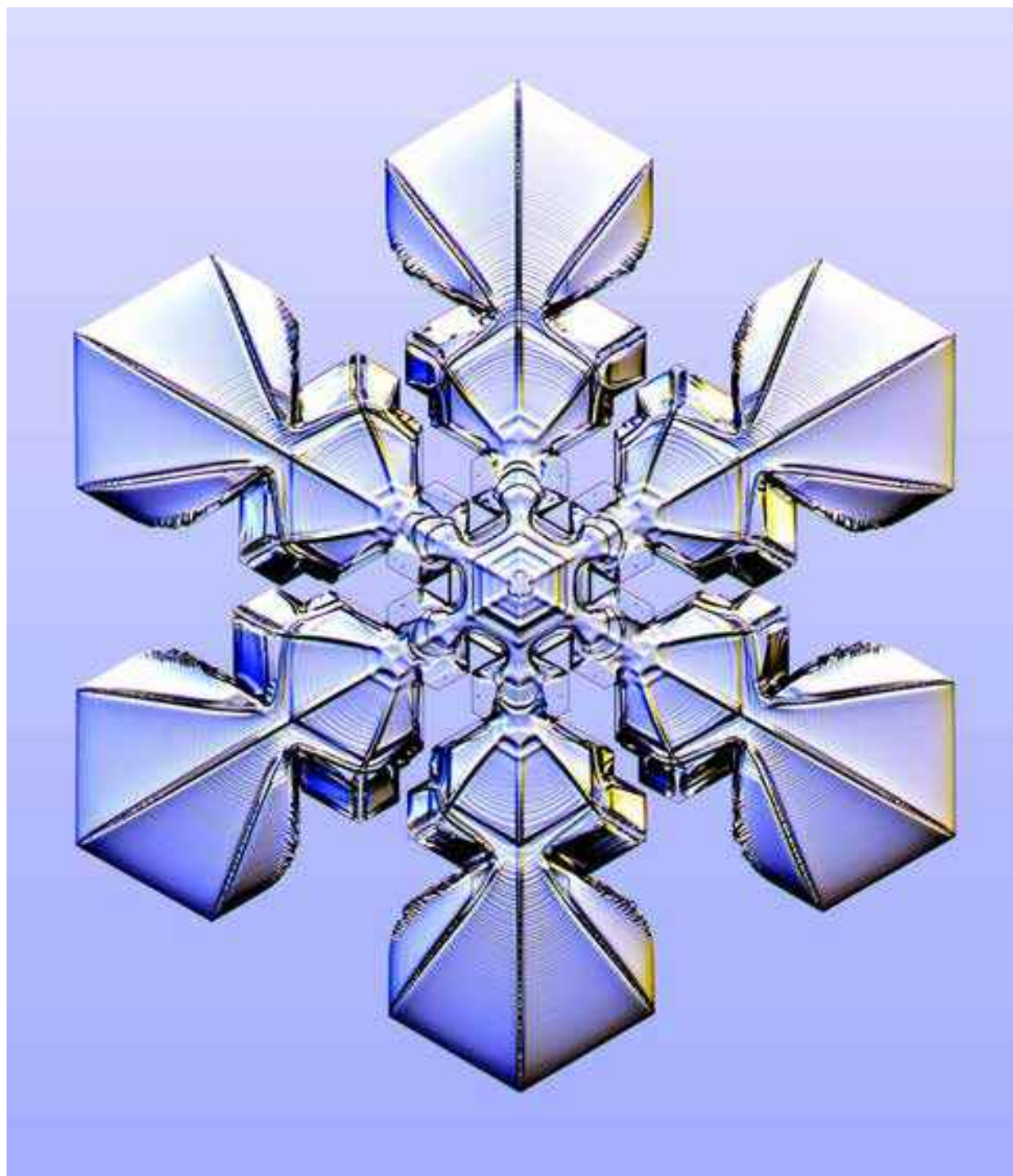
Figure 9.40: (Above and facing page) Snow crystal portraits. The PoP technique is well suited for creating large stellar crystals with complex designs and nearly flawless symmetry. When photographing natural snowflakes, beautiful specimens like these are hard to find! Moreover, PoP snow crystals often exhibit razor-sharp facets and exceptionally crisp surface features, because they are photographed while they are being grown. In contrast, natural snow crystals usually experience a bit of sublimation after they leave the clouds, rounding their features and generally giving them a bit of a “travel-worn” appearance.
