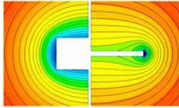
Figure 8.28. Calculated contour plots of supersaturation levels around growing ice crystals, shown here in (r,z) coordinates. Around a blocky crystal (left), the supersaturation is highest near the corners of the faceted prism, a phenomenon called the Berg effect. Around a thin-plate crystal, the contour lines are tightly bunched at the plate edge. This is because the fast-growing edge requires a steep gradient in the supersaturation to supply a sufficient flux of water vapor molecules.
