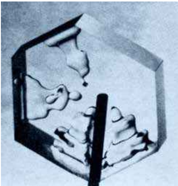
Figure 6.40: A “negative” snow crystal growing at -14^{\circ}\text{C} in a block of single-crystal ice, as a vacuum pump removes water vapor via a 0.45-mm-diameter capillary tube. The morphology of the void is determined from thermal diffusion effects together with a strong nucleation barrier in the sublimation kinetics. As with normal snow crystal growth, surface energy effects here are negligible compared to anisotropic sublimation kinetics. (Image from [1965Kni].)
