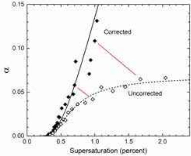
Figure 7.13: The basal growth data from Figure 7.12 converted to the basal attachment coefficient \alpha as a function of supersaturation. The open points show the uncorrected \alpha_{uncorrected} = v/v_{kin}\sigma_{\infty} plotted as a function of \sigma_{\infty} , while the filled points show the corrected \alpha = v/v_{kin}\sigma_{surf} plotted as a function of \sigma_{surf} . The red lines show how two individual points transformed from uncorrected to corrected.
