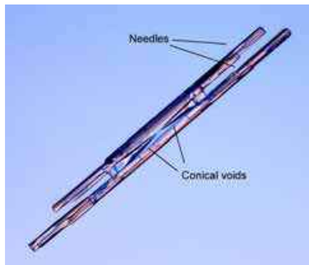
Figure 3.33: This crystal began as a solid column when it was small, but soon transformed into a hollow column, leaving behind central conical voids in the ice as it grew. Later, the corners of the basal edges sprouted branches, here taking the form of slender ice needles.
