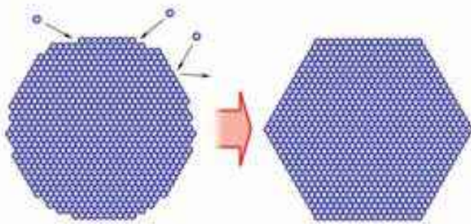
Figure 1.8: When water vapor molecules strike a molecularly rough ice surface, they tend to stick. But when they strike a molecularly smooth facet surface, they are less likely to stick. As the crystal grows, soon the rough areas fill in, leaving a fully faceted ice prism.
