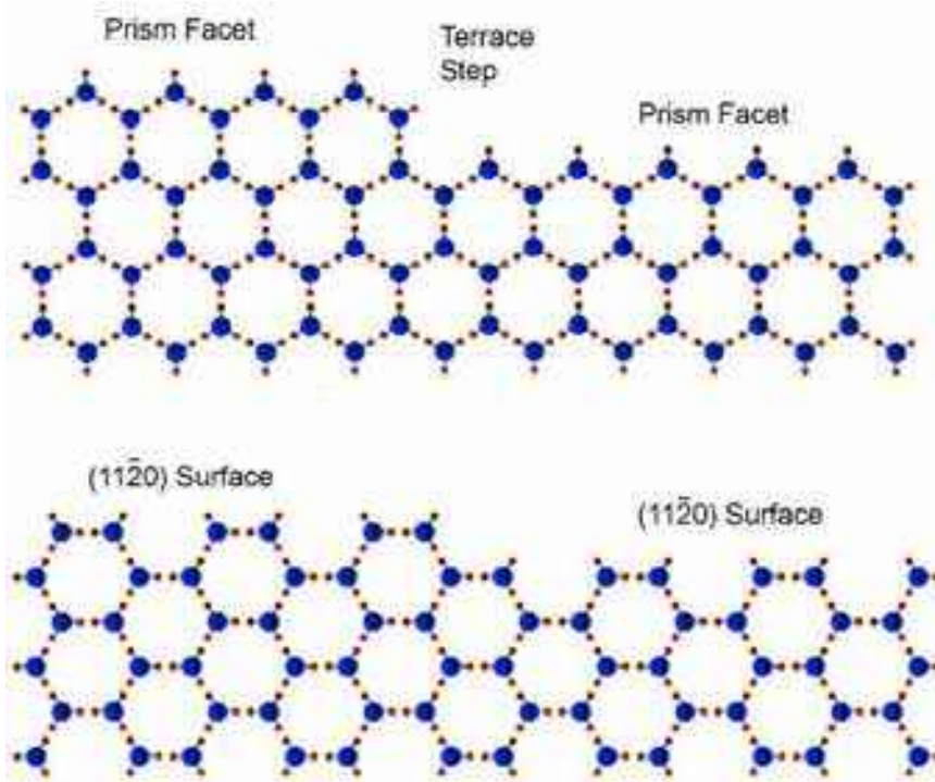
Figure 2.10 (left): Terrace steps on a prism \{1\bar{0}10\} facet and a \{11\bar{2}0\} surface, as seen looking along the [0001] direction. Note that the prism step is more distinct, and admolecules would likely bind much more strongly at a terrace step than on the prism facet. In contrast, the \{11\bar{2}0\} step is less distinct, and binding at the step edge is likely not much stronger than elsewhere on the surface. The larger terrace step in the top sketch suggests stronger faceting on the prism surface, as is observed.
