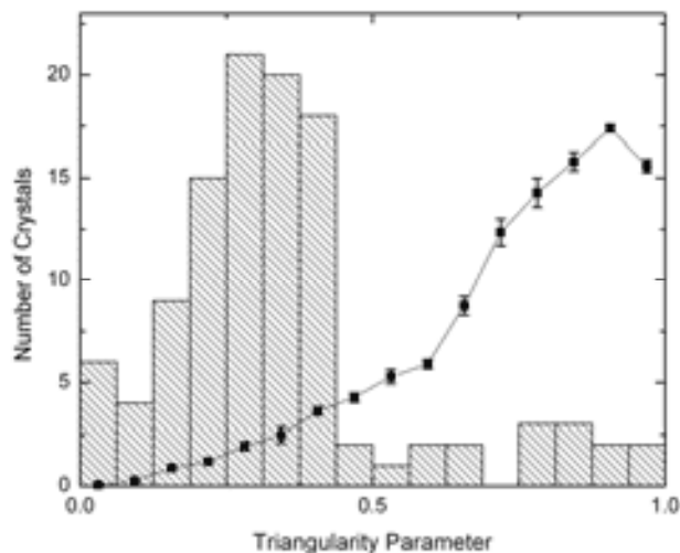
Figure 3.61: The distribution of measured values of the triangularity parameter T for a sample of plate-like crystals with H < 0.33 grown at -10 C. The line shows a Monte-Carlo model that assumes random growth perturbations of a hexagonal plate, again for crystals with H < 0.33 [2009Lib4]. These data indicate that truncated triangular plates are far more common than other non-hexagonal simple plates.
