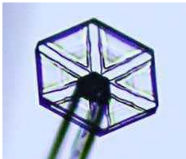
Figure 3.39: A laboratory snow crystal growing on an e-needle with (T, \sigma) = (-16^\circ\text{C}, 16\%) . Under these constant conditions, the hollow regions grew as roughly triangular segments separated by solid ice spokes.
