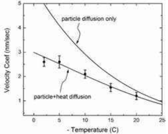
Figure 3.20: Measurements of the radial growth of thin ice needles, together with an analytical model that included only particle diffusion (top line), plus a similar model that included both particle and heat diffusion (lower line) [2016Lib]. The plotted velocity coefficient is equal to the cylinder growth rate at a fixed far-away supersaturation and a fixed cylinder radius of five microns, as described in [2016Lib]. The measurements show good agreement with the particle+heat diffusion model, confirming the temperature-dependent reduction in growth rate caused by latent heating.
