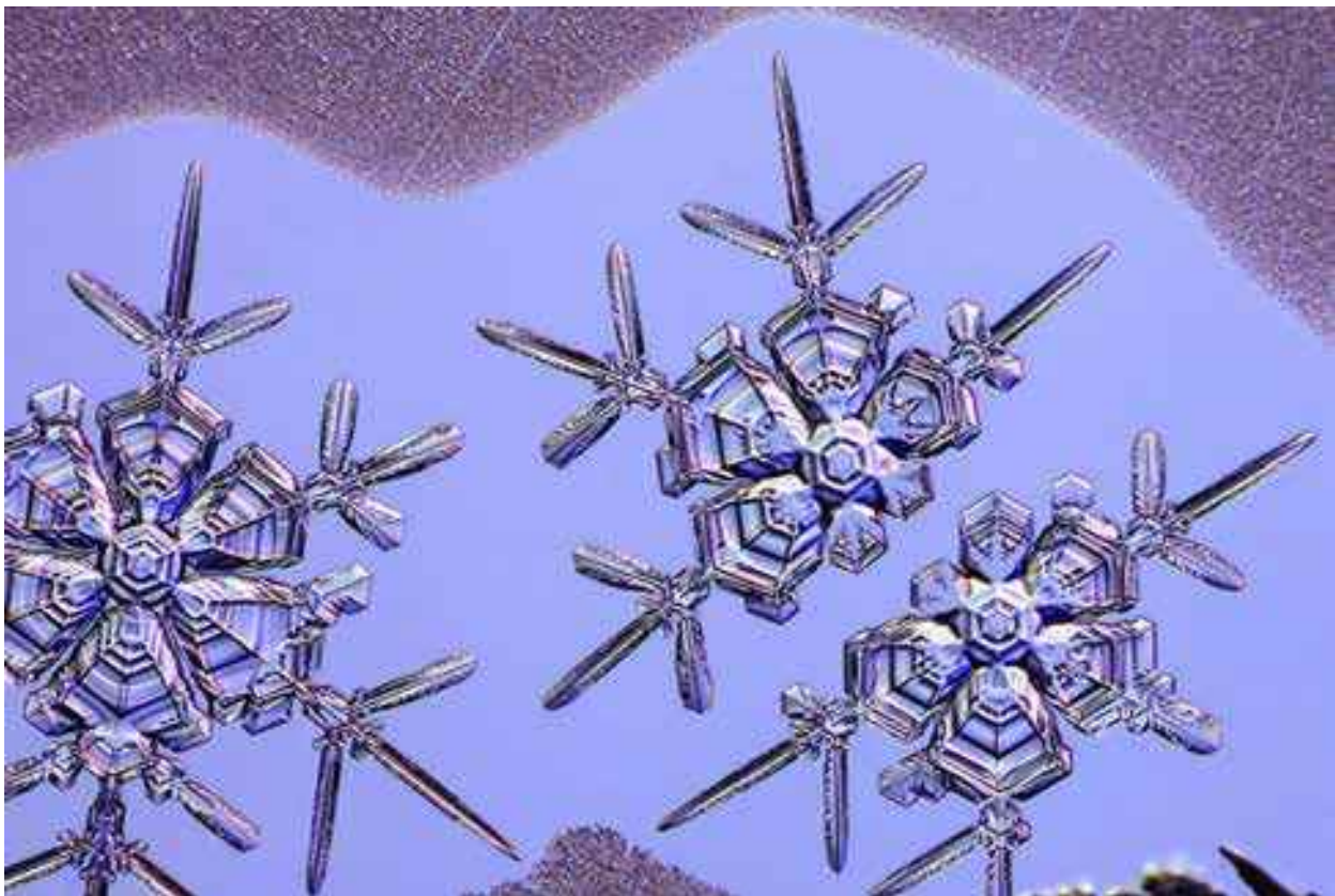
Figure 9.42: (Above and facing page) Asymmetry all around. When two or more PoP snow crystals grow in close proximity, they compete for the supply of water vapor in their vicinity, which can lead to quite a variety of odd asymmetrical crystals. For most of these photos, I focused my attention on an isolated crystal at the center of the camera's field of view, which grew with good symmetry. When finished with that crystal, I then looked outside the original field to see what else looked interesting.
