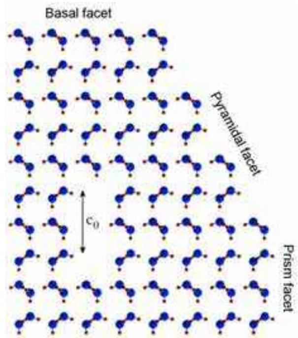
Figure 2.8: A projection of the ice Ih lattice looking along the [11\bar{2}0] direction, showing the basal, prism, and pyramidal facets. The angle between the prism and pyramidal facets is \tan^{-1}(\sqrt{3}a_0/2c_0) = 28.0 degrees. (The 31.5-degree angle seen in Figure 2.6 is from looking along the [\bar{1}010] direction, which is not parallel to a pyramidal facet.)
