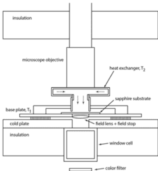
Figure 9.4: (Left) An expanded schematic view of the PoP growth region shown in Figure 9.3. In operation, saturated air at temperature T_2 blows gently down onto the substrate with its growing PoP crystal at temperature T_1 < T_2 . Not shown is a white-light LED lamp placed underneath the color filter in this sketch.
