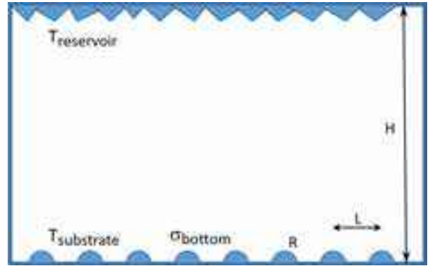
Figure 3.21: Analytic solutions of the diffusion equation can be quite useful for estimating the supersaturation in an experimental ice growth chamber, such as in this example. Even if there is only a low density of ice crystals on the bottom of the chamber, the supersaturation there can be reduced to surprisingly low levels.
