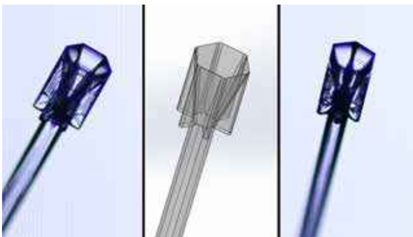
Figure 3.47: Cups with Fins. The photos on the left and right show two views of a cup-shaped snow crystal growing on the end of a slender ice column. The 3D drawing (center) illustrates the main structural features, including six plate-like “fins” that are related to snow crystal ridges. The laboratory crystals were grown on an e-needle (see Chapter 8) near -7^{\circ}\text{C} . [SolidWorks drawings by Ryan Potter.]
