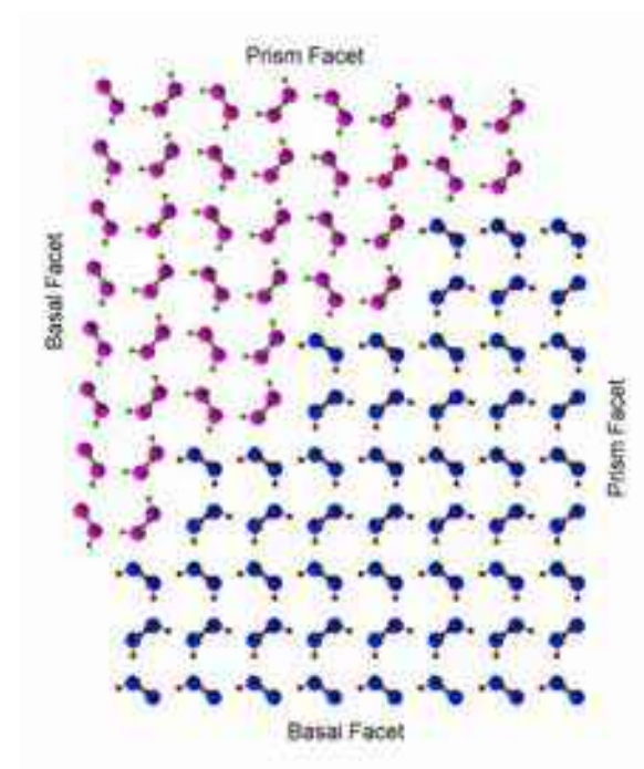
Figure 2.32: Crossed Plates Variant I. A possible lattice model for Variant-I crossed-plate twinning. This is a contact twin where the theoretical angle between basal facets is 2 \tan^{-1}(c_0/\sqrt{3}a_0) = 86.5 degrees.
