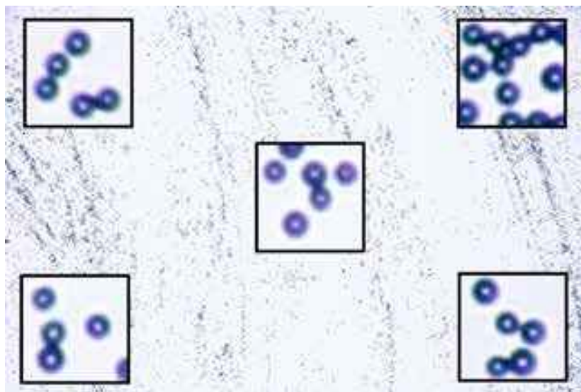
Figure 9.6: The background image here shows a dusting of 10- \mu\text{m} -diameter glass beads spread over the sapphire substrate, for testing image quality across the 56x37 mm field of view. Sub-images near the center and four corners were magnified to gauge image quality. The sharpness in the corners of the frame was noticeably improved in this image by using focus stacking of five images.
