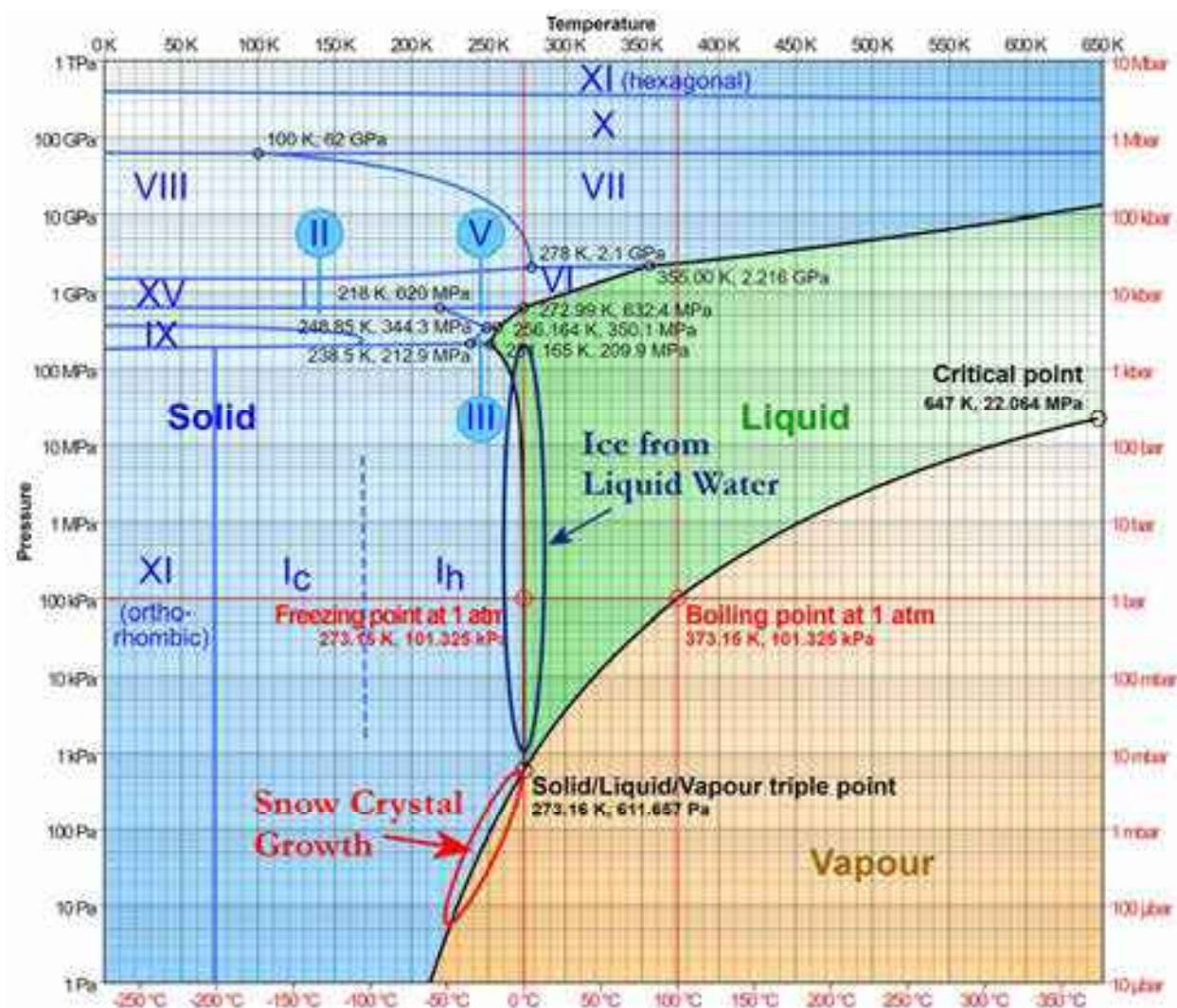
Figure 12.1: The phase diagram of water as a function of temperature and pressure. Ice growth occurs near the liquid/solid phase boundary (blue oval) while snow crystal growth occurs near the vapor/solid boundary (red oval). The high-pressure portion of the liquid/solid boundary is difficult to access experimentally, so nearly all observations of ice growth from liquid water have taken place near one atmosphere. Image adapted from https://en.wikipedia.org/wiki/Ice .
