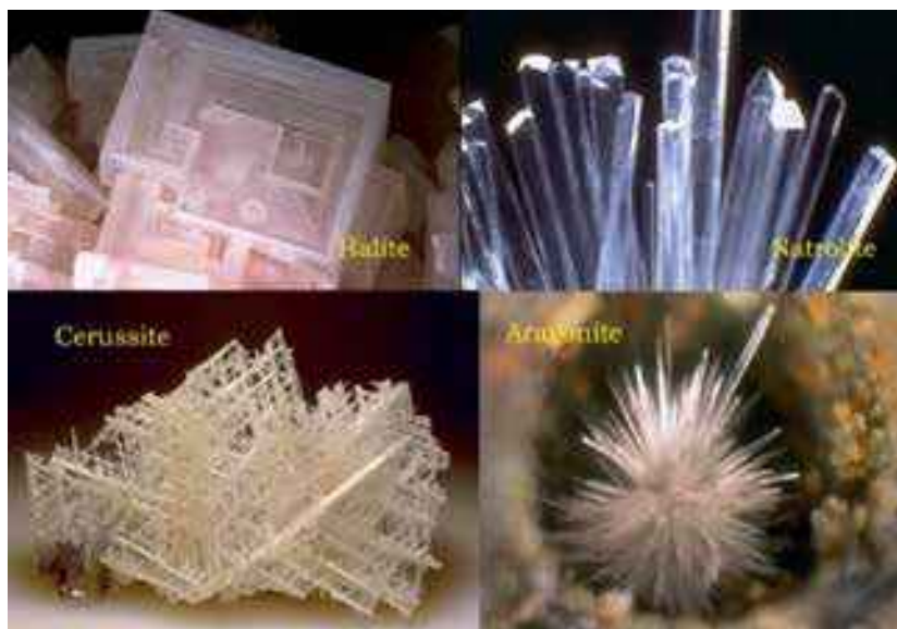
Figure 1.20: Many mineral crystals grow into faceted morphologies under the right conditions, as seen in these examples. The lattice structure determines the overall symmetry of these crystalline forms, but the attachment kinetics is largely responsible for the appearance of faceted surfaces.
