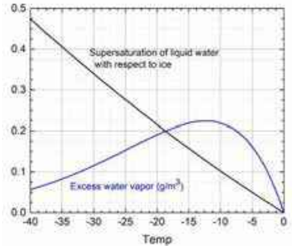
Figure 2.14: The supersaturation of supercooled water with respect to ice, given by \sigma_{water}(T) = [c_{water}(T) - c_{sat}(T)]/c_{sat}(T) . This is also plotted as the “excess” water vapor, equal to [c_{water}(T) - c_{sat}(T)]m_{water} .
