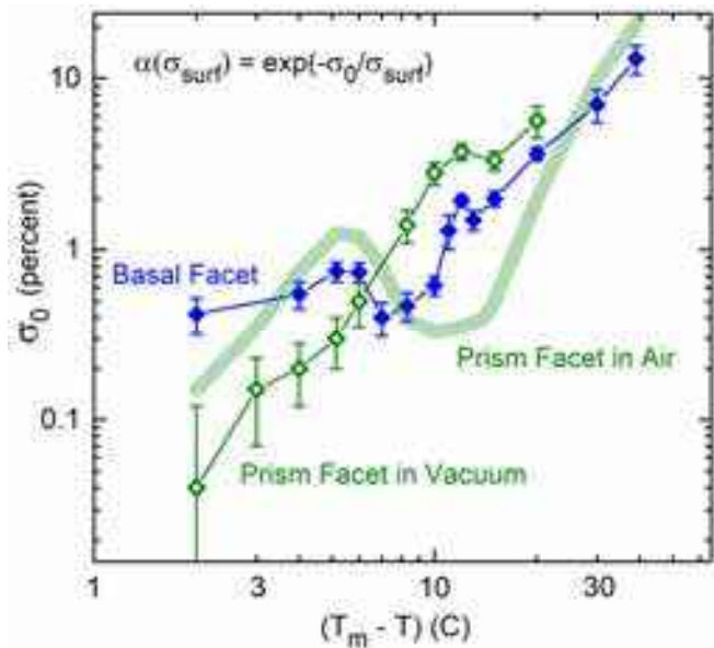
Figure 7.25: A comprehensive model of the ice attachment kinetics in both air and near vacuum. This model assumes that the \alpha_{basal}(\sigma_{surf}) (given by the blue data) are independent of air pressure. The green data points then give \alpha_{prism}(\sigma_{surf}) at low pressure, while the thick green line shows \alpha_{prism}(\sigma_{surf}) in air at one atmospheric pressure. The physical origin of the large change in \alpha_{prism}(\sigma_{surf}) with air pressure is discussed in Chapter 4.
