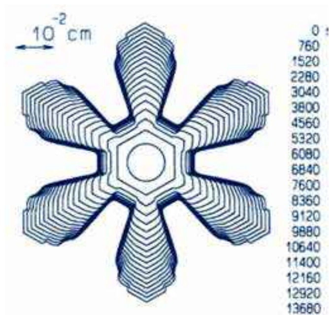
Figure 5.3: This numerical model by Yokoyama and Kuroda [1990Yok] exhibits an initial transition from a round seed crystal to a faceted plate, followed by the formation of six primary branches. Unlike earlier investigations, these authors created the first detailed physical model of the specific phenomenon of snow crystal growth from water vapor.
