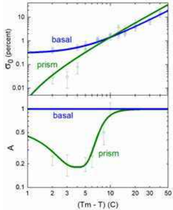
Figure 4.5: The smooth curves in these graphs show best-estimate CAK model functions \sigma_0(T) and A(T) on large basal and prism facets as a function of temperature, where T_m = 0 C is the ice melting point. The respective attachment coefficients are then given by \alpha(\sigma_{surf}) = A \exp(-\sigma_0/\sigma_{surf}) . The underlying experimental data and measurement techniques used to obtain these curves are described in Chapter 7. Because these curves parameterize the large-facet attachment kinetics over a broad range of growth conditions, they provide the foundation for the CAK model of the snow crystal attachment kinetics.
