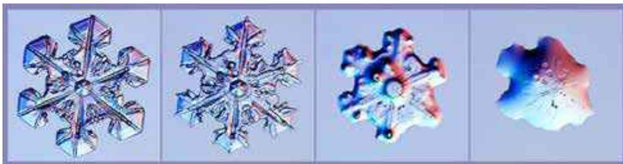
Figure 11.7: This series of photos shows a snow crystal melting, with just 27 seconds elapsed between the first and last image. The temperature was just below 0 C during this series, illustrating how challenging it can be to photograph snow crystals at such warm temperatures.
