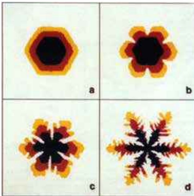
Figure 5.2: A progression from faceted prism growth (a) to dendritic growth (d) in a two-dimensional DLA model [1988Xia]. This work was the first to demonstrate a morphological transition of this nature resulting from the competing processes of diffusion-limited growth and surface attachment kinetics.
