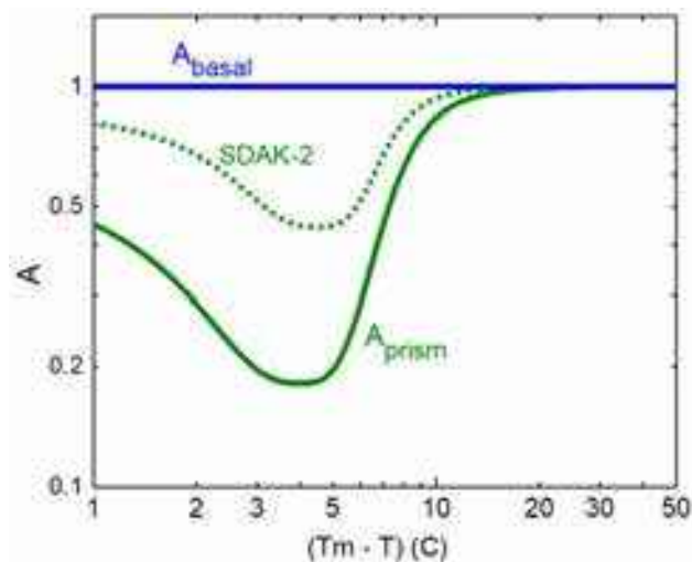
Figure 4.14: The SDAK-2 mechanism increases the value of A_{prism} on small prism facets at temperatures above -10 C, as approximated here by the dotted curve. This curve is expected to depend on supersaturation, such that A_{prism} \rightarrow 1 at especially high \sigma_{surf} . The solid curves are reproduced from Figure 4.5. This change in A_{prism} mainly affects the growth of sharp-tipped dendritic structures, which are often observed in high-supersaturation experiments.
