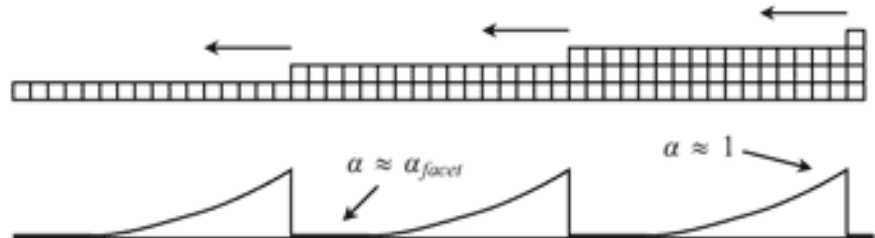
Figure 5.20: (below) On a low-angle vicinal surface, molecules can diffuse along a faceted surface to reach kink sites where they readily attach. Thus \alpha \approx \alpha_{facet} far from a kink site, while \alpha \approx 1 within one surface-diffusion length from a kink site. Here we have assumed a high Ehrlich–Schwoebel barrier that prevents diffusion over the tops of terrace steps.
