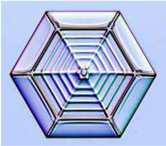
Figure 3.51: While growing this POP snow crystal, I periodically reduced and then increased the supersaturation, yielding the inner “spider-web” structure of ribs and ridges. After that, I added an extra-thick rib and then let the thin plate grow out unencumbered. Hexagonal rib patterns like these are typically associated with changes in external growth conditions.
