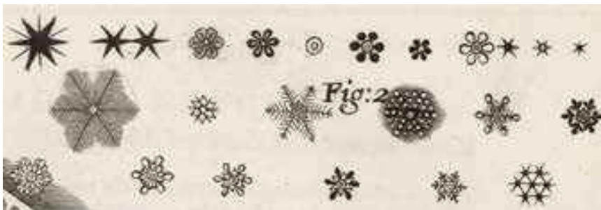
Figure 1.15: Robert Hooke sketched these observations of snowflakes 1665, enabled by his newly invented microscope [1665Hoo].
