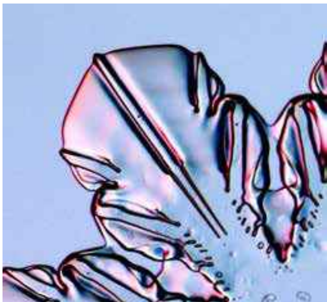
Figure 3.45: This photo shows a partially sublimated sectorial snow crystal that exhibits a pair of “grooves” flanking the central ridge. Similar features can be found in many snow crystals, although usually they are not as distinctive as in this example.
