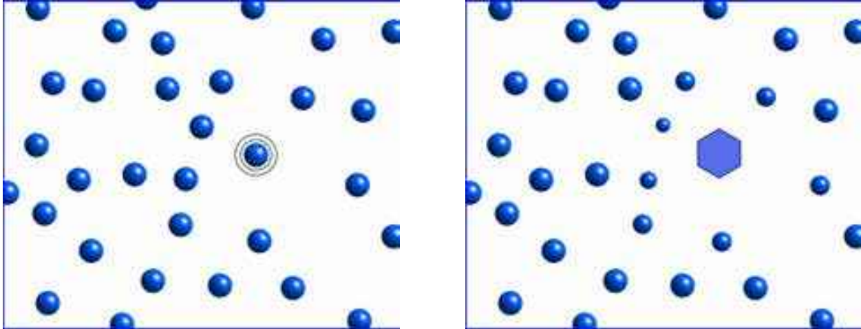
Figure 1.5: A snowflake is born when a liquid cloud droplet freezes into ice (first sketch). The ice particle initially grows into a faceted prism (second sketch), as the growth is limited by anisotropic attachment kinetics on the ice surface. After the crystal grows larger, the diffusion of water molecules through the air causes branches to sprout from the six corners of the prism (third sketch). The growing crystal removes water vapor from the air, which is replenished by the evaporation of nearby water droplets (fourth sketch). About 100,000 cloud droplets evaporate to provide enough material to make one large stellar snow crystal. The flake continues growing inside the cloud until it becomes so heavy that it falls to earth.
