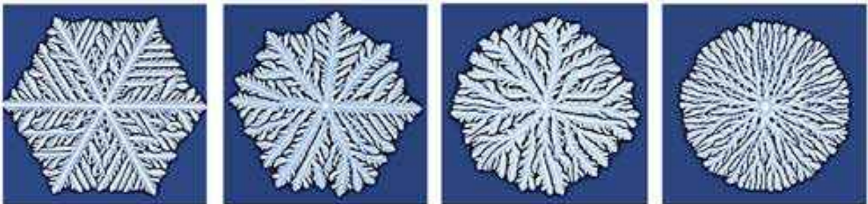
Figure 3.26: In crystal growth, some kind of surface anisotropy, usually in the attachment kinetics or surface energy, is necessary to prevent tip splitting and create stable free-dendrite growth (far left). For perfectly isotropic systems, seaweed-like structures emerge (far right). This numerical simulation shows a morphological transition between these two states, in this case when the underlying anisotropy possesses six-fold symmetry. (Image from [2006Gra1].)
