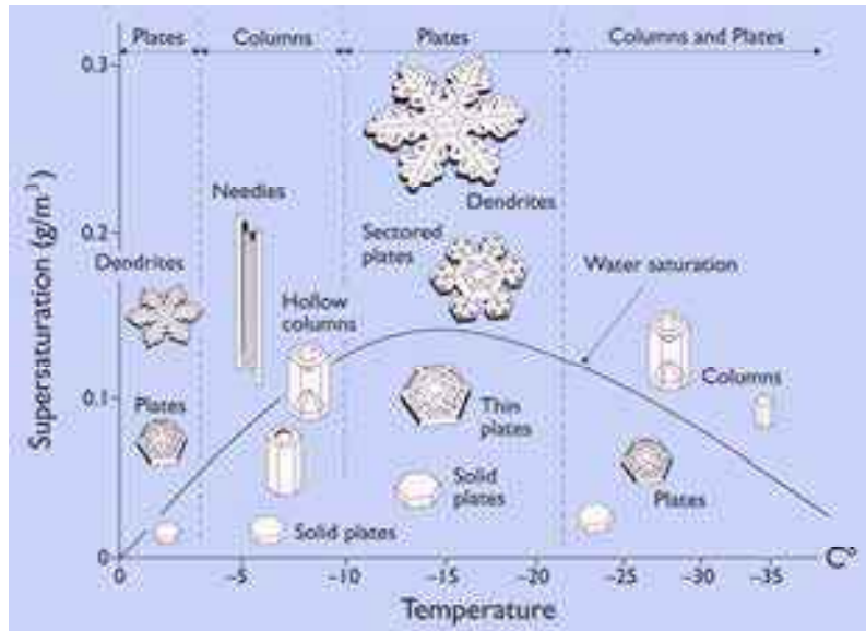
Figure 1.12: The Nakaya diagram illustrates the morphologies of snow crystals that develop at different temperatures and supersaturations. The water saturation line shows the supersaturation that is typically found in a dense winter cloud made of liquid water droplets.
