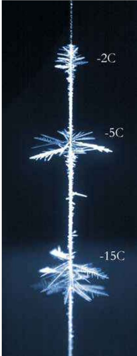
Figure 6.29: A string of snow crystals growing at high supersaturation in a diffusion chamber like that shown in Figure 6.27. The fastest-growing dendritic crystals cluster at -2^{\circ}\text{C} , -5^{\circ}\text{C} , and -15^{\circ}\text{C} . At other temperatures, the crystals tend to be blocky in form with slower growth rates.
