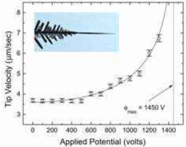
Figure 8.6. Experimental measurements (data points) showing a gradual increase in the tip growth velocity of an ice dendrite at -15 C as the applied voltage was increased. The line through the data points comes from the theory contained in Equation 8.5, with A adjusted to fit the data. Note that the dendrite morphology continued to exhibit sidebranching as the voltage was initially increased. Once a threshold voltage was exceeded, however, normal dendrite growth gave way to the formation of an electric needle. The inset image shows a similar run in which the normal dendrite growth transformed into a fast-growing a-axis e-needle above threshold. From [1998Lib].
