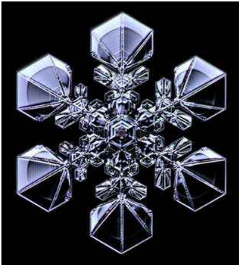
Figure 9.11: (Left) An image of a PoP snow crystal using dark-field illumination. In the absence of any ice, no light enters the microscope objective, so the background is dark. The crystal appears bright because the ice refracts some light from oblique angles toward the objective. In this case, the central light was blocked using a slightly off-center opaque spot in place of the color filter in Figure 9.4, giving an asymmetry in the overall illumination of the crystal.
