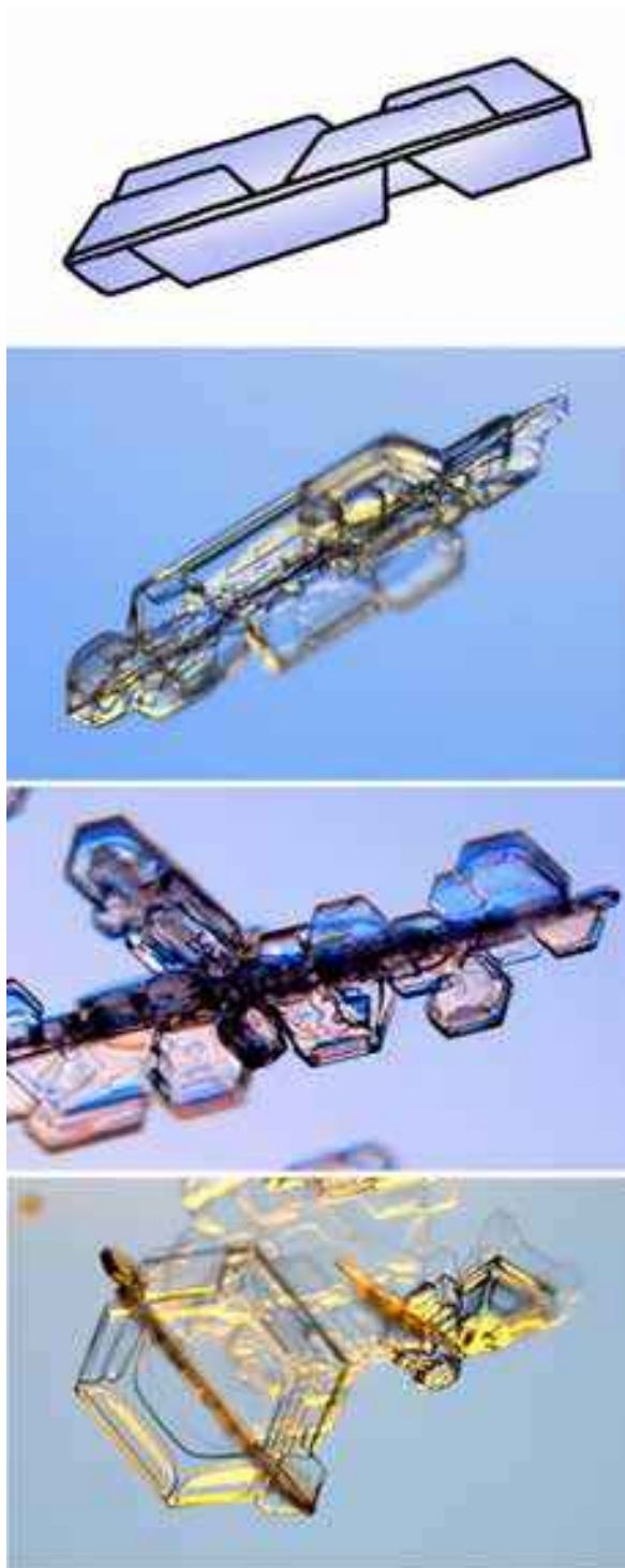
Figure 2.31: Crossed Plates Variant I. These photos show examples of natural twin-plate crystals, along with a sketch of their overall structure. Note that one prism facet edge is parallel to the intersection axis of the twinned crystals. Top, bottom images by Patricia Rasmussen [2003Lib2].
