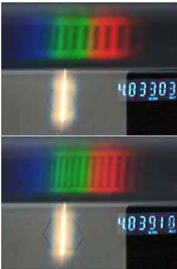
Figure 7.8: (Left) Two still images from a video showing the growth of a test crystal. The top parts of both images show interferometer fringes in true colors, while the bottom parts of the images show a direct image of the crystal including illumination from the slit. The numerical section in the images show a voltage from which \Delta T can be determined. The upper image was taken near the beginning of the growth cycle. The lower image shows the same crystal after it had grown larger and thicker. The bright slit light is periodically blocked to provide a better direct image of the crystal.
