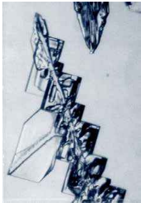
Figure 2.30: Arrowhead Twins Variant III. Walter Tape photographed this sharply faceted example of an arrowhead twin near the South Pole [2006Tap]. A careful measurement of the crystal (by KGL) yielded an apex angle of 88.5 \pm 0.5 degrees, in good agreement with the model shown in Figure 2.29.
