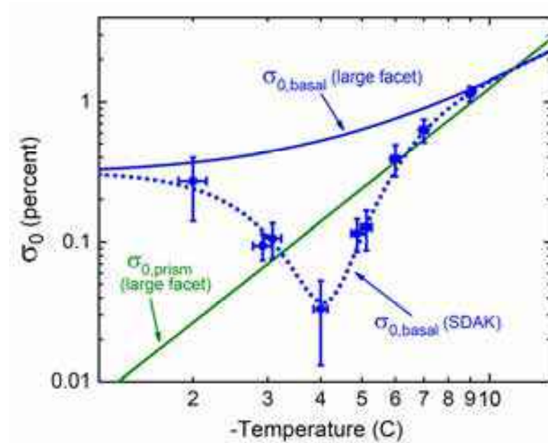
Figure 4.27: Measurements of the basal SDAK parameter \sigma_{0,basal,SDAK} as a function of temperature, revealing a substantial “SDAK dip” centered near -4 C [2020Lib2]. For comparison, the solid lines show the CAK model parameters \sigma_{0,basal} and \sigma_{0,prism} for broad-facet growth.
