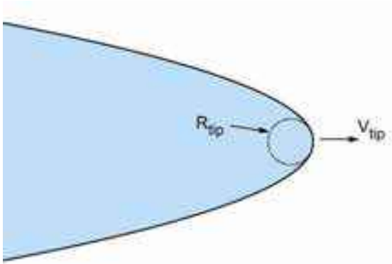
Figure 3.22: The Ivantsov solution to the diffusion equation describes a crystalline paraboloid of revolution with a constant parabolic shape and tip radius R_{tip} that grows forward with a constant velocity v_{tip} . If viewed from a frame of reference that moves in the growth direction with velocity v_{tip} , the system would appear completely static.
