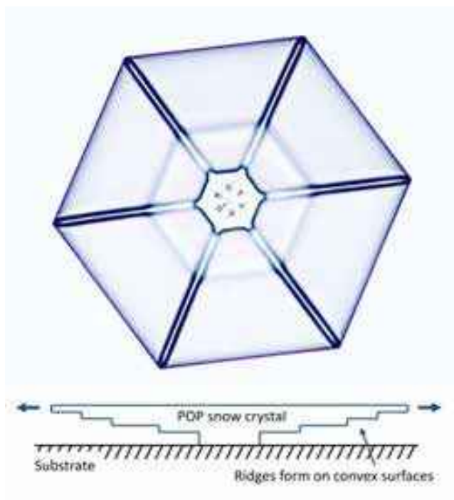
Figure 3.41: A small Plate-on-Pedestal (POP) snow crystal exhibiting simple ridges that originate at the six faceted corners as the plate grows outward. As shown in the accompanying sketch, the top basal surface of this crystal is essentially flat and unfeatured, while the ridges and other visible structural features exist on the convex lower surface of the crystal.
