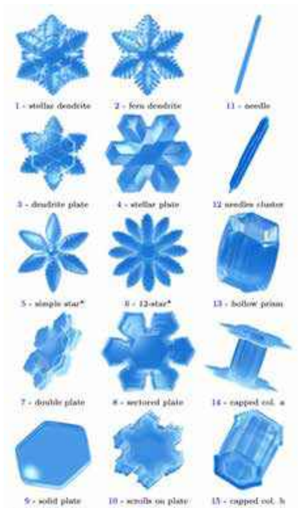
Figure 5.7: Additional 3D phase-field models of several well-known snow crystal morphologies, from [2017Dem1].
