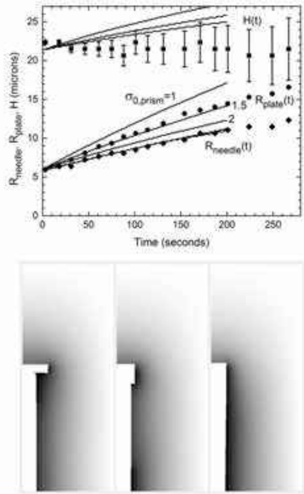
Figure 8.27. Measurements of the plate radius, needle radius, and axial growth as a function of time, from the data shown in Figure 8.26. Lines through the data are from numerical models of the growing crystals, and the lower images show computer-generated cross sections of the three model crystals shown in the upper graph. From [2015Lib2].
