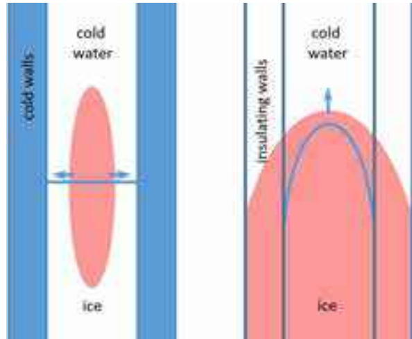
Figure 12.17: A possible model to explain the orientation of ice growth in constrained channels, here a small-diameter capillary tube. In the left sketch, the tube conducts heat well and is cold. In the right sketch, the tube walls are insulating. Red shows areas of concentrated heating from latent heat deposition for the two cases. The arrows show the maximum temperature gradients at the growing ice surfaces.
