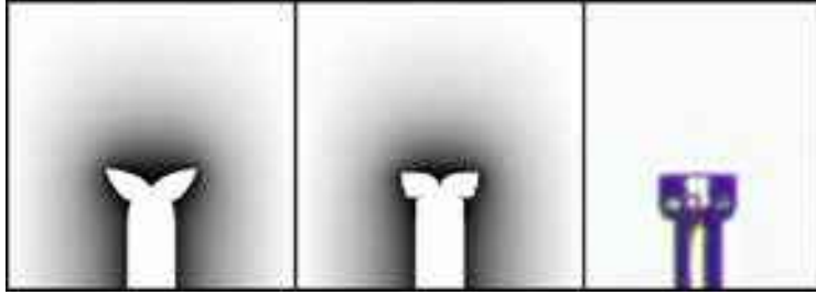
Figure 5.25: The image on the right shows a blocky prism forming on the end of an electric ice needle near -10\text{ }^{\circ}\text{C} [2015Lib1]. Other than a few minor surface markings, the block has a relatively simple morphology with essentially no basal hollowing. The image on the left shows an attempt to model the blocky growth using a simple facet-kink CA model. With reasonable model adjustments, it was not possible to eliminate the substantial basal hollowing. The center image shows another attempt using a fast-surface-diffusion approximation, yielding an improved morphology with less basal hollowing. The CA models could not produce a sensible model with no basal hollowing, however, so perhaps some additional physics is needed in the model.
