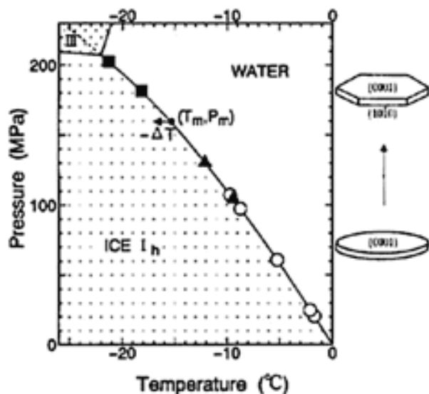
Figure 12.7: The growth form of ice in water at low supercooling changes from thin disks (open circles) to faceted hexagonal plates (solid squares) with position on the ice/water coexistence line. The transition likely arises from a change in the prism attachment kinetics with temperature/pressure, specifically the terrace step energy on prism facets.
