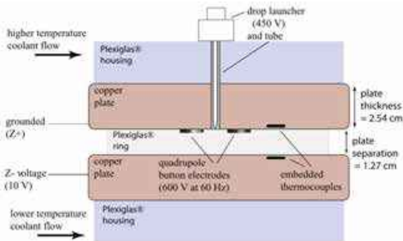
Figure 6.37: (Right) In this electrodynamic trap [2016Har], a trapping quadrupole electric field oscillating at 60 Hz is delivered via a set of “button” electrodes, while a constant vertical electric field balances gravity. The parallel-plate diffusion-chamber geometry allows for precise modeling of the supersaturation at the position of a trapped ice crystal.
