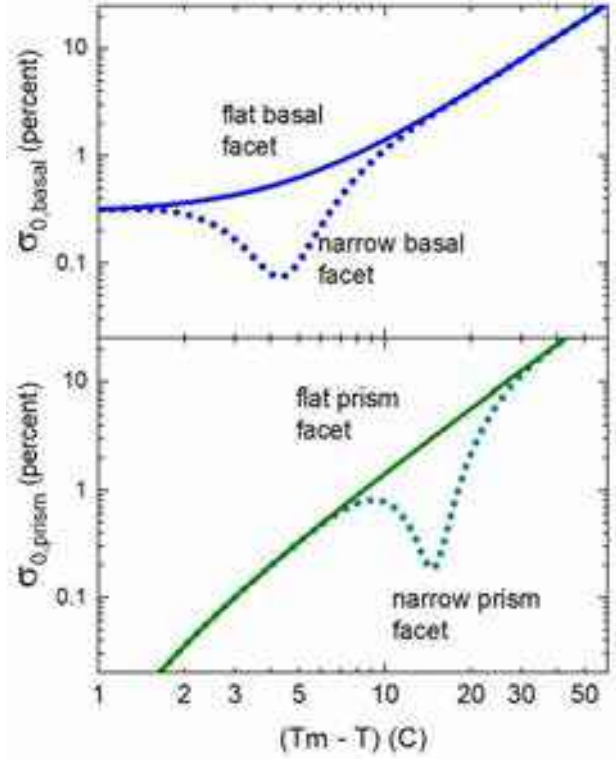
Figure 4.12: The solid lines in these two graphs are reproduced from Figure 4.5, again illustrating the CAK terrace-nucleation model for the attachment kinetics on large basal and prism facets. The dotted lines show the “SDAK dips” described in the text. Near -5 C, the narrow basal facets on hollow columns exhibit a much reduced effective \sigma_{0,basal} , explaining the rapid growth of these features. Near -15 C, narrow prism facets exhibit a similarly low effective \sigma_{0,prism} , explaining the growth of thin plates at that temperature.
