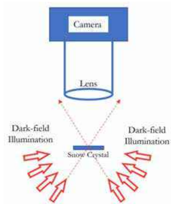
Figure 11.22: Dark-field Illumination. This variation of back illumination uses only light that does not enter the lens in the absence of a snow crystal. If not deflected, the light rays shown in the sketch all pass outside the lens. A snow crystal will refract some of those rays, however, sending them into the lens. The result is a bright snow crystal on a dark background, as shown in DFI#1.
