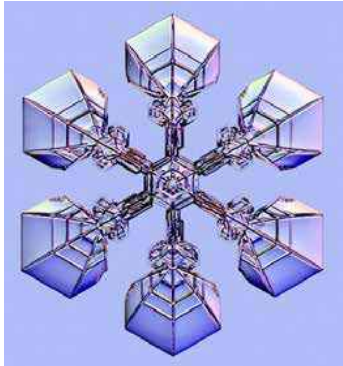
Figure 3.52: This POP snow crystal exhibits broad, plate-like extensions growing on the ends of narrow branches. Here again, the two prominent sets of ribs in the plates did not appear spontaneously but were induced by twice lowering the supersaturation to form a rib, then increasing it back again to resume the thin-plate growth.
