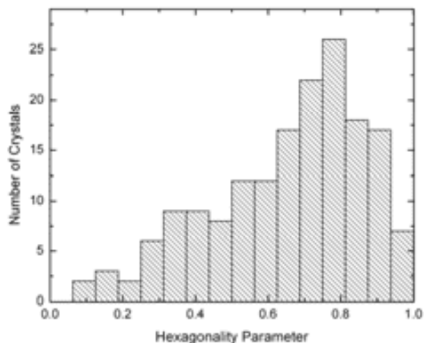
Figure 3.60: The distribution of measured values of the hexagonality parameter H for an unbiased sample of small plate-like crystals grown at -10 C. These data show that most plates are visually hexagonal in shape, but near-perfect hexagons are rare.
