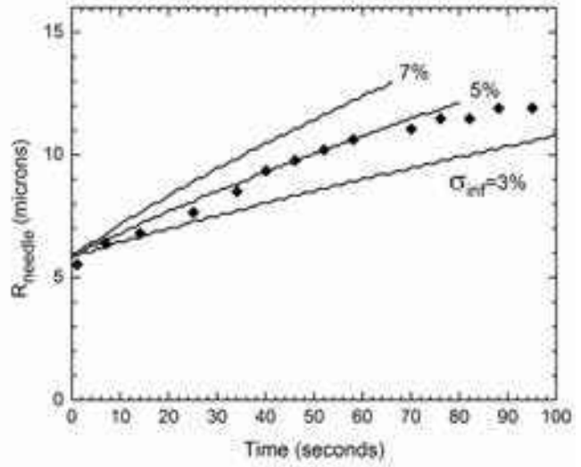
Figure 8.23. The needle growth data from Figure 8.22 along with several models using different values of \sigma_{far} . As long as \alpha_{diffcyl} \ll \alpha_{prism} (which is true in most circumstances), then the modeled R_{needle}(t) is essentially independent of \alpha_{prism} , while being approximately proportional to \sigma_{far} , as seen in this graph. Thus, the measured R_{needle}(t) allows one to determine \sigma_{far} with quite good accuracy, even when \alpha_{prism} is not well known. This result is somewhat counter-intuitive, but it follows directly from the analytical theory of the diffusion-limited growth of ice cylinders discussed in Chapter 3.
