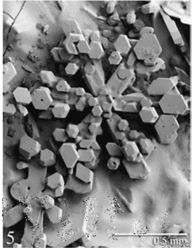
Figure 6.16: An electron micrograph of a stellar snow crystal covered with numerous small hexagonal prisms. Note that the facets of the small prisms all align with the underlying stellar prisms, indicating epitaxial growth [2003Erb].
