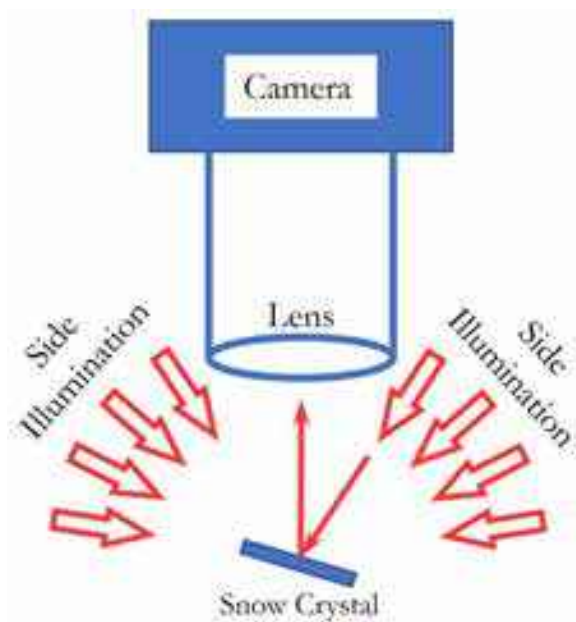
Figure 11.17: Specular Reflection. In this variation of side illumination, a plate-like snow crystal is tilted so the flat face of the crystal reflects light into the camera lens. With this arrangement, thin plates appear much brighter than with the face-on side illumination method shown in Figure 11.16.
