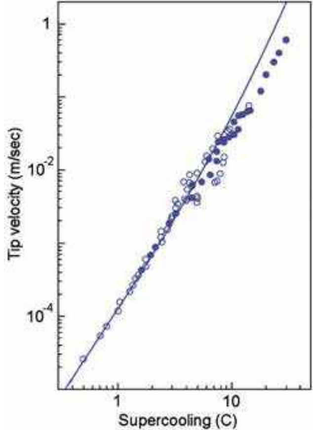
Figure 3.25: Measurements of the free dendrite tip velocity for ice growing from liquid water as a function of the far-away supercooling. The line shows a calculation from solvability theory. (Figure adapted from [2005Shi], with additional context given in [2017Lib].)
