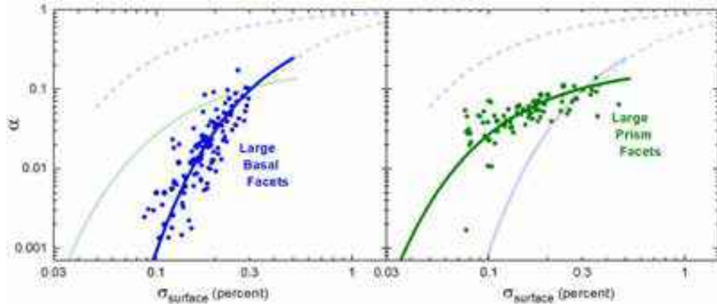
Figure 4.18: Data points in these two graphs show measurements of \alpha_{basal}(\sigma_{surf}) and \alpha_{prism}(\sigma_{surf}) at -5 C in a low-pressure environment. Lines in both graphs are from the CAK model for -5 C, while nonessential curves have been faded in the different panels. These observations reveal that platelike habits are the norm for simple ice prisms at -5 C, with thinner plates forming at lower supersaturations. These plots combine measurements from the VIG and VPG experiments described in Chapter 7.
