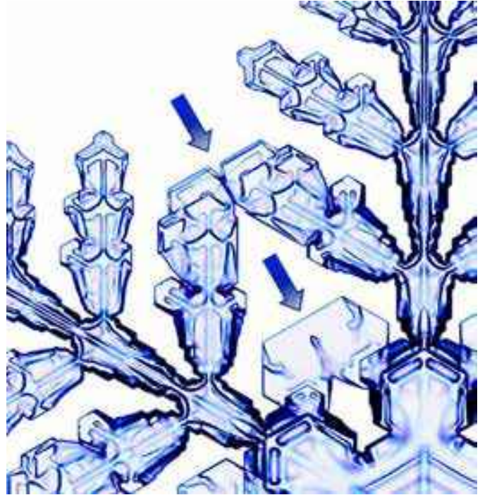
Figure 5.14: A laboratory-grown POP snow crystal with two instances of sidebranch mergers (arrow). The upper merger occurred relatively recently before the photo was taken, so the separate branch edges are still clearly seen. The lower merger is older, and the individual sidebranches have grown together into a single flat plate.
