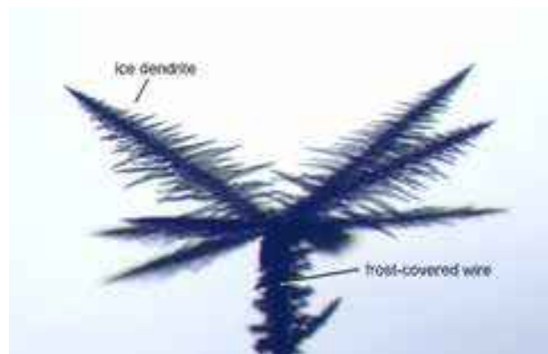
Figure 3.10: Several “fishbone” dendrites growing out from a frost-covered wire at a temperature of -5\text{ C} . Note the overall similarities between the different dendritic branches.
