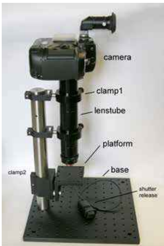
Figure 11.14: One possible rigid mounting system for snowflake photography, using the basic optical layout shown in Figure 11.9. Here the microscope objective is mounted on a threaded ring that moves the objective up and down by rotating the ring. A right-angle eyepiece is used to view the image through the DSLR camera. The base plate, vertical bar, clamps, and other mounting components are commercially available from Thorlabs and Edmund Optics.
