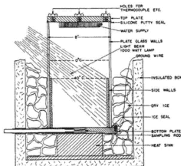
Figure 6.28: Perhaps the first snow-crystal diffusion chamber, cooled with dry ice [1952Sch].
