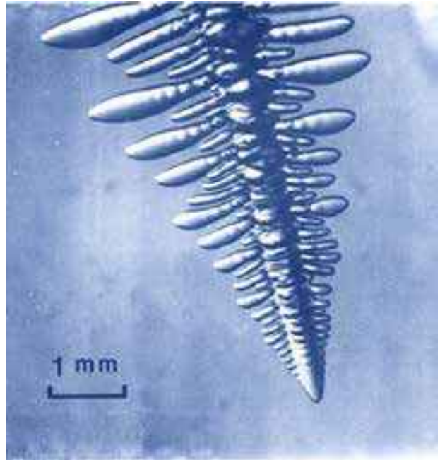
Figure 1.27: This photo shows a dendritic crystal of succinonitrile growing into a supercooled melt of the same material. Under constant conditions, the tip advances at a constant growth velocity while the radius of curvature of the tip remains constant [1981Hua].
