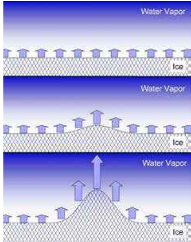
Figure 3.6: The diffusion-limited growth of an initially flat surface with \alpha \approx 1 (top sketch) is susceptible to the Mullins-Sekerka instability, also known as the branching instability. If a small bump appears on the surface (center), it will stick out farther into the supersaturated medium, so the top of the bump will grow slightly faster than the surrounding flat surface. This initiates a positive feedback effect, causing the bump to become larger, increasing its relative growth rate even more (bottom). This illustration assumes zero anisotropy in the attachment kinetics ( \alpha \approx 1 ) to eliminate the possibility of faceting and thus emphasize the Mullins-Sekerka instability.
