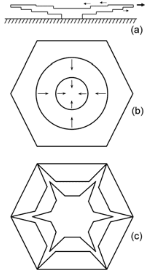
Figure 3.50: (a) The overall geometry of a POP crystal, as seen from the side. Steps represent molecular terraces on the basal surfaces. (b) Growth on the concave top surface yields nearly circular inward-propagating steps. Step bunching turns a series of one-molecule-high steps into a coarser series of macrosteps that can be seen using optical microscopy. (c) Faster step advancement near the hexagonal corners yields ridges on the lower convex surface.
