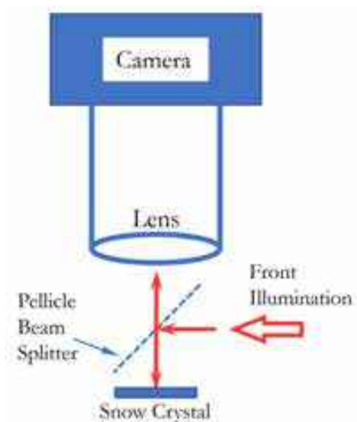
Figure 11.20: (Left) Front Illumination. This variation of specular-reflection illumination uses a pellicle beamsplitter to direct light onto a plate-like crystal. In contrast to Figure 11.17, the face-on crystal lies nicely in the image plane, avoiding depth-of-focus issues.
