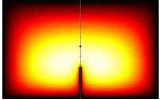
Figure 8.15. A finite-element diffusion model of the supersaturation field in DC2 at a fixed \Delta T . The supersaturation goes to zero (black) at the frost-covered walls and exhibits a broadly peaked maximum (yellow/white) below the chamber center. The black dot indicates the center of the chamber, which is the location of the growing e-needles. By running the model with different top and bottom temperatures, one can determine the supersaturation at the center of the chamber as a function of \Delta T .
