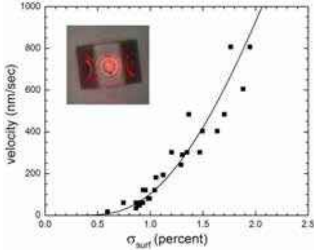
Figure 4.4: Ice-growth measurements (data points) are well described by a terrace nucleation model (curve) [2013Lib]. Chapter 7 describes these data in detail.
