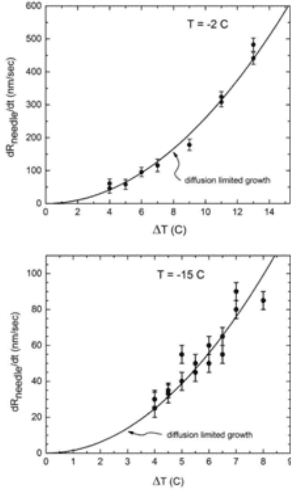
Figure 8.18. Example measurements at -2 C and -15 C showing the radial growth velocity of cylindrical ice needles when the needle radius was equal to 5\text{ }\mu\text{m} . The data are shown as a function of \Delta T = T_{\text{top}} - T_{\text{bottom}} in DC2, which is proportional to the supersaturation according to Equation 8.7. Fitting the data reduces it to a single parameter A(T) , with the growth velocity given by dR/dt = A(t)\Delta T^2 when the needle radius is equal to 5\text{ }\mu\text{m} [2016Lib].
