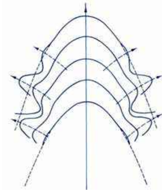
Figure 3.7: A schematic diagram showing the creation of dendritic sidebranches resulting from repeated application of the Mullins-Sekerka instability [1980Lan]. Random perturbations on the sides of the growing tip typically yield somewhat erratically placed sidebranches. However, there is often a characteristic length scale involved in the formation of these perturbations, resulting in a somewhat regular spacing between adjacent sidebranches.
