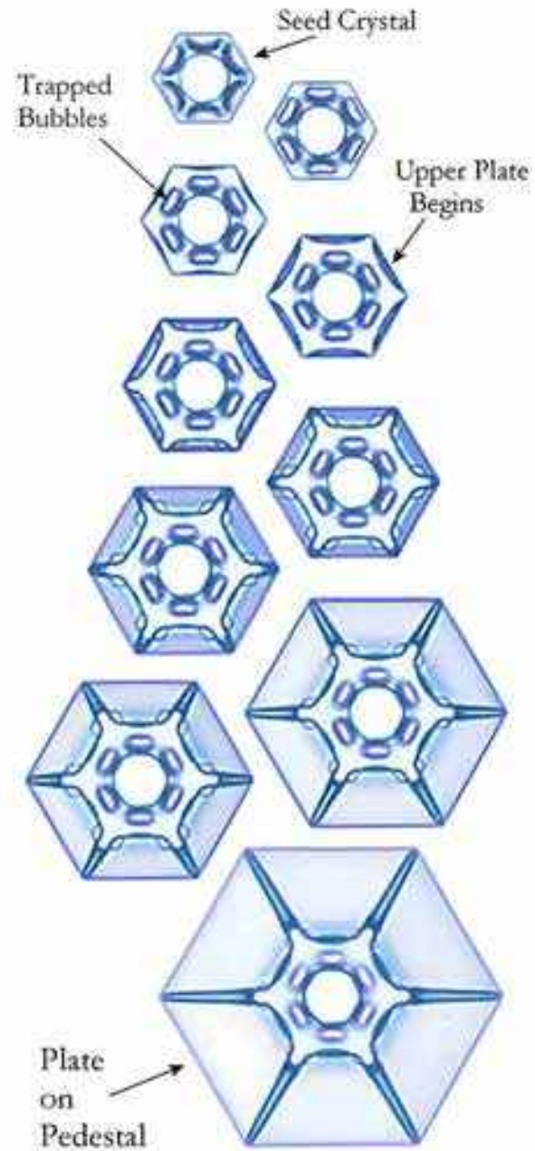
Figure 9.2: Multiple images showing the formation of a PoP snow crystal from a seed crystal, here growing from about 50\text{ }\mu\text{m} to 170\text{ }\mu\text{m} in diameter. The seed crystal exhibited some non-faceted structure, and its early growth trapped six small bubbles between the ice and the substrate surface. Once formed, these isolated bubbles did not evolve substantially as the upper plate formed. Note that the final thin, hexagonal plate is not touching the substrate, but is supported above it, as illustrated in Figure 9.1.
