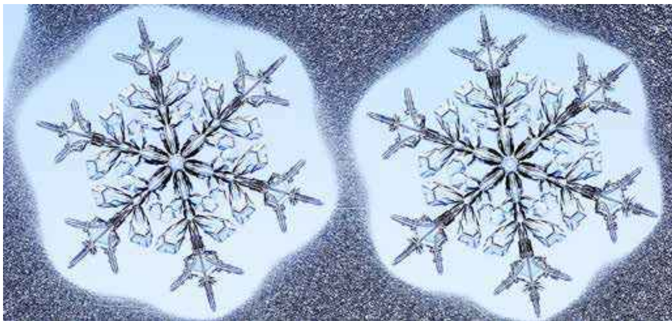
Figure 9.36: A pair of “identical-twin” snow crystals, grown side-by-side in the PoP apparatus.
