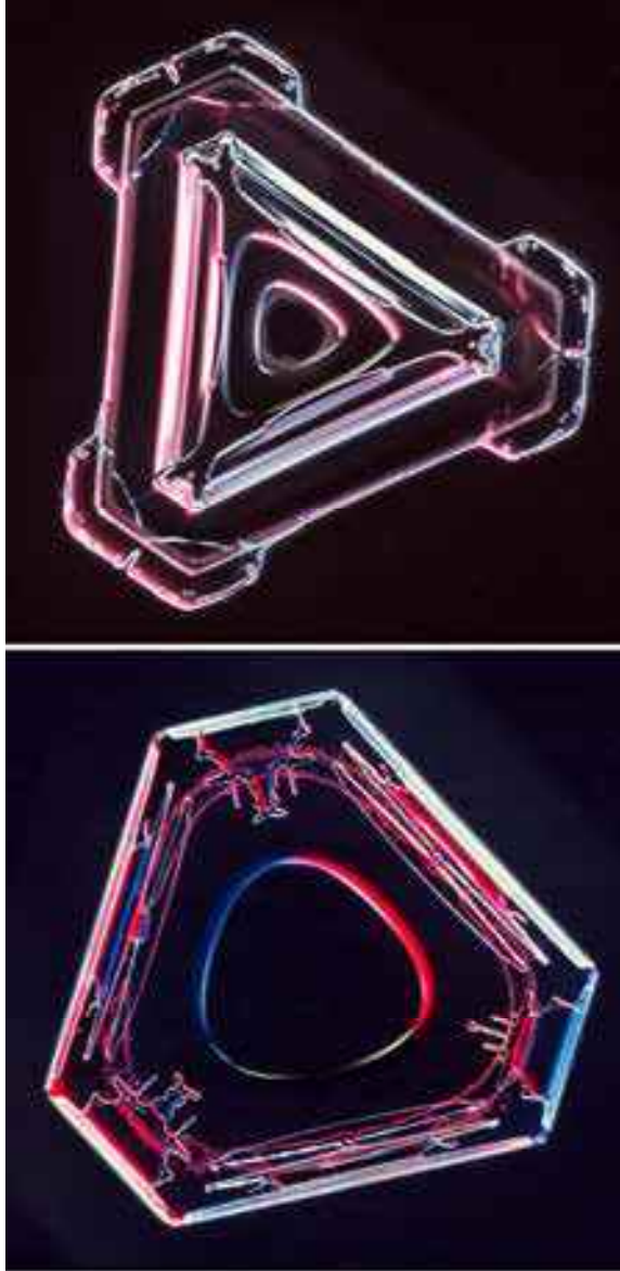
Figure 3.58: These natural snow crystals are shaped like small truncated triangular plates. They typically appear together with much larger numbers of normal hexagonal plates.
