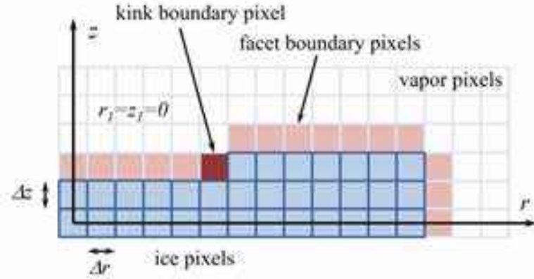
Figure 5.16: A pixel geometry for a 2D cylindrically symmetric cellular automaton model. Ice pixels are shown as blue while vapor pixels are white. The “facet” boundary pixels (adjacent to faceted ice surfaces) are pink, while this particular model includes a single red “kink” boundary pixel that touches two ice pixels. For convenience I often take \Delta r = \Delta z = \Delta x , which defines the generic pixel size \Delta x .
