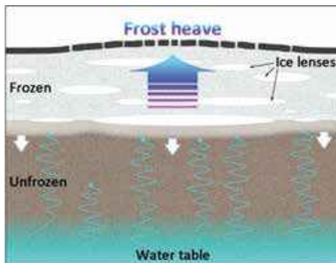
Figure 12.13: The phenomenon of frost heave is often responsible for pushing up road surfaces in cold weather, producing potholes in the process. Contrary to popular belief, the well-known expansion of water upon freezing does not produce frost heave. Segregation provides the dominant mechanism, as ice “lenses” push out porous soil particles, increasing the overall volume of the frozen layer relative to its previously unfrozen state. Image adapted from https://www.dmr.nd.gov/ndgs/documents/newsletter/2011Summer/FrostHeave.pdf
