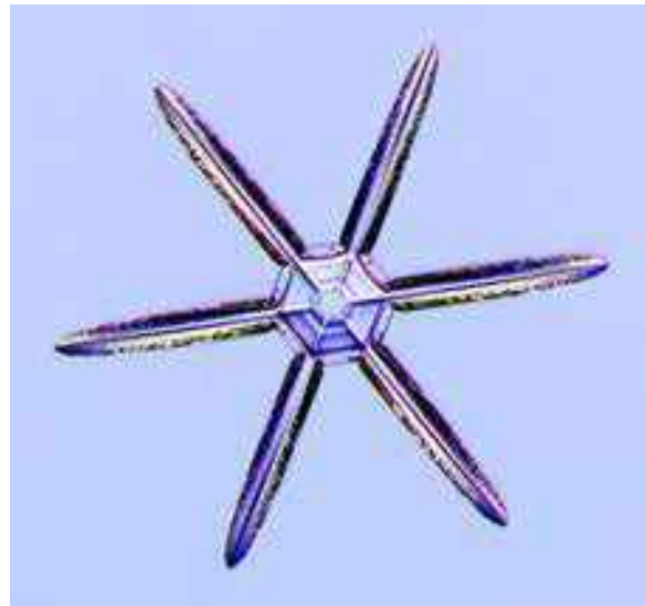
Figure 9.22: Narrow PoP branches can grow quite stably near -15 C, yielding a spiked star like this one. Dendritic structures will not form under constant growth conditions, however, because droplets condensing around the crystal will prevent the supersaturation from becoming high enough to drive spontaneous sidebranching.
