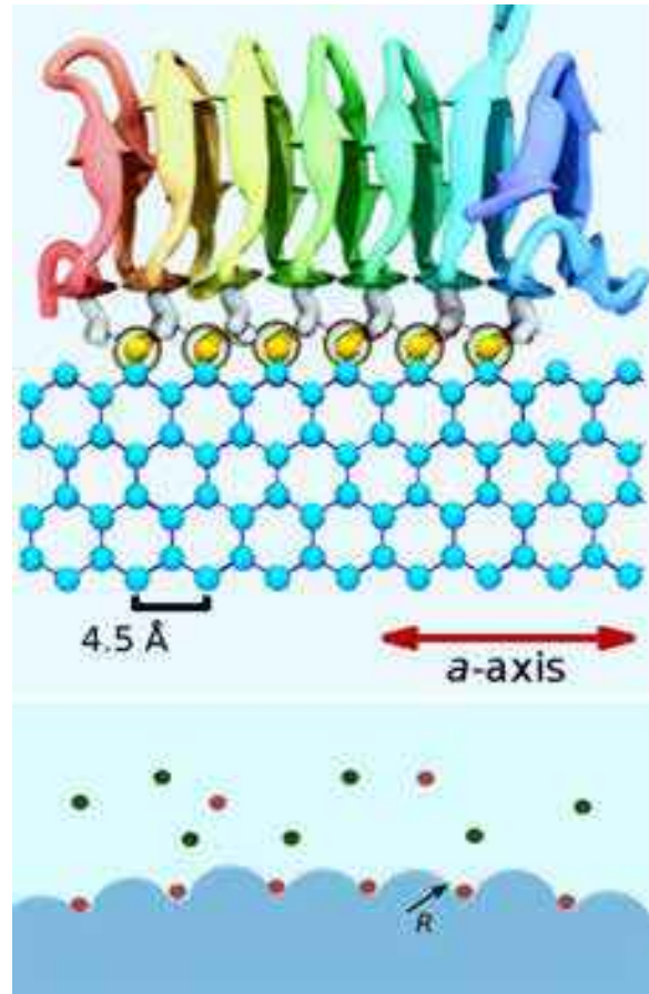
Figure 12.14: Top: An illustration of how an antifreeze protein might bind to an ice crystal surface. Bottom: Even a sparse density of growth inhibitors on an ice surface (red dots) can halt growth over the whole surface via the Gibbs-Thomson effect, as the induced surface curvature lowers the temperature needed for additional growth. Image adapted from [2015Kui].
