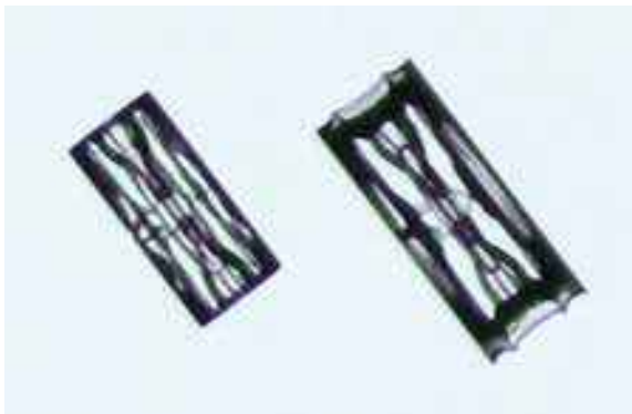
Figure 9.33: Sheath-like growth of a small columnar crystal observed in the PoP apparatus.
