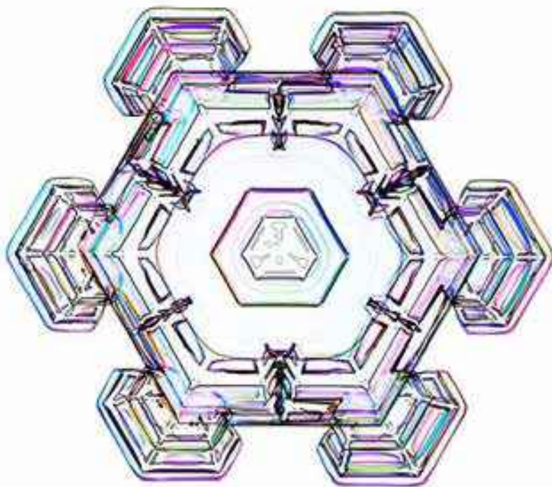
Figure 3.54: (Below) This natural snow crystal apparently experienced many variations in supersaturation that resulted in a complex set of rib-like surface features. Because the crystal tumbled through the atmosphere as it grew, the ribs likely formed on both basal surfaces, in contrast to the simpler ribs seen on POP crystals.
