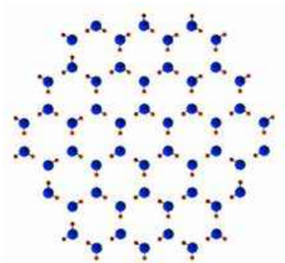
Figure 2.3: A 2D toy-model example of the Bernal–Fowler rules in ice Ih (although the full 3D rules do not visualize especially well in 2D). The basic idea sketched here is that there are many possible ways to orient the individual \text{H}_2\text{O} molecules in the crystal while keeping exactly one hydrogen atom between each adjacent pair of oxygen atoms, with each hydrogen forming one strong and one weak bond.
