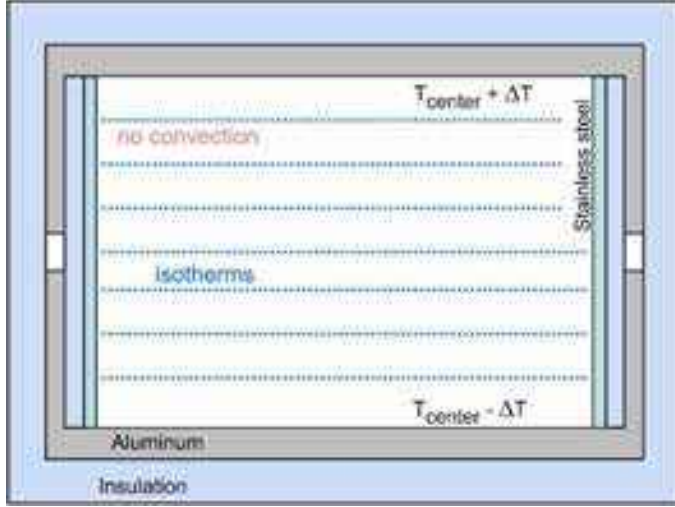
Figure 6.33: A “linear-gradient” diffusion chamber, designed using (moderately conducting) stainless-steel wall to produce a linear temperature profile. With this simpler thermal structure, it becomes possible to model the supersaturation within the chamber with a quite high accuracy.
