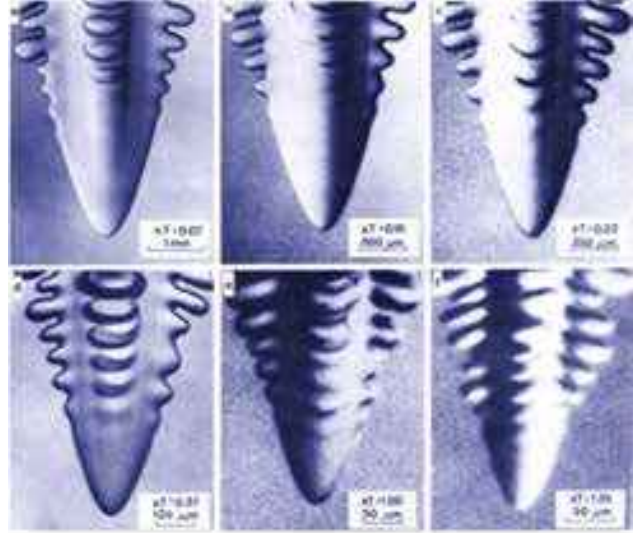
Figure 3.23: A series of photographs showing the tips of free dendrites growing during the solidification of liquid succinonitrile (a clear, waxy material that melts at 57 C). As the supercooling \Delta T of the liquid increases, R_{tip} decreases while v_{tip} increases, their product R_{tip}v_{tip} satisfying the Ivantsov relation for thermal diffusion. Meanwhile the overall growth behavior and dendrite tip morphology remains nearly independent of \Delta T . (Image from [1981Hua].)
