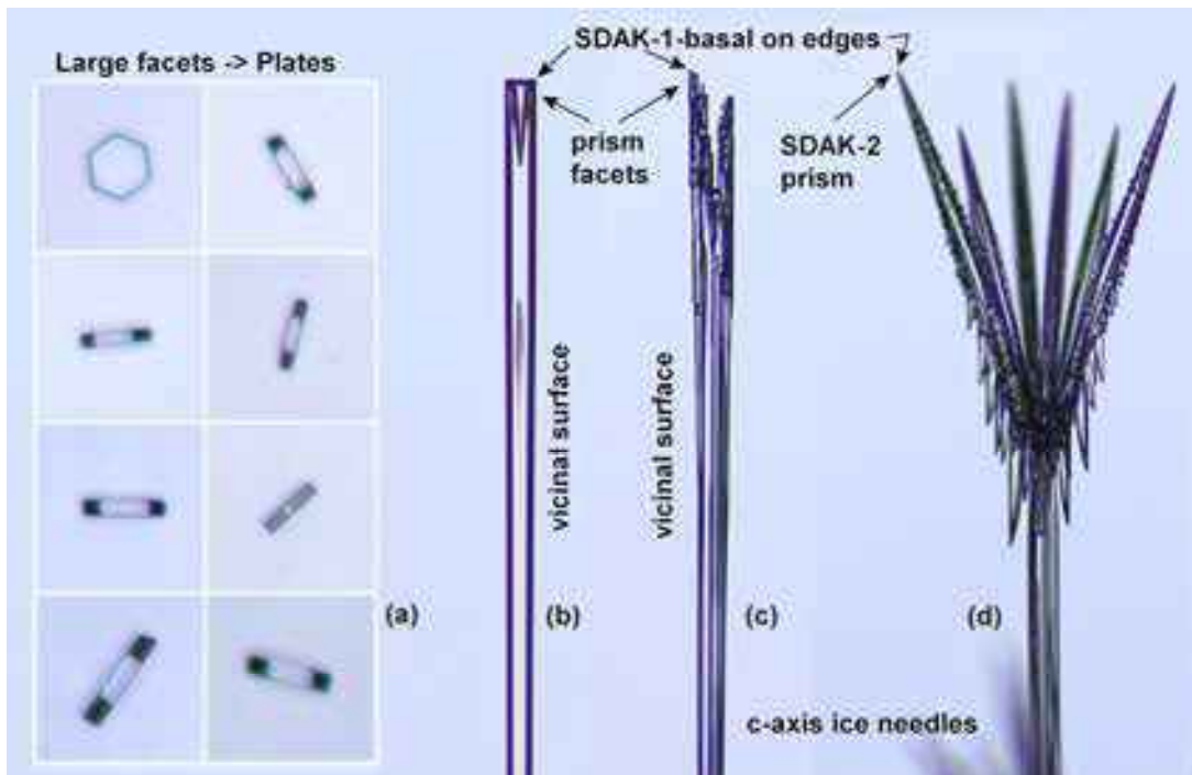
Figure 4.22. This photo collage illustrates several snow crystal growth behaviors at -5 C. (a) With simple prisms grown in vacuum, thick plates are the norm. (b) Starting with a c-axis needle in air (Chapter 8), the basal ESI from the SDAK-1 phenomenon brings about sharp basal edges and a hollow column. (c) At a higher supersaturation, the hollow column splits into a needle cluster. (d) At still higher growth rates, the SDAK-2 mechanism increases the prism kinetics, yielding dendritic structures where the opening angle increases with supersaturation. All four CAK branches in Figure 4.21 are needed to reproduce these different growth behaviors.
