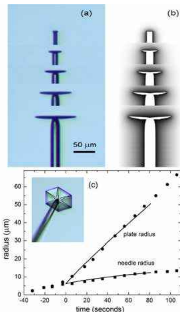
Figure 5.24: These figures illustrate a quantitative comparison a 2D CA model with experimental data [2008Lib, 2013Lib]. (a) A composite image made from five photographs shows the growth of a plate-like snow crystal on the end of an electric ice needle, viewed from the side. (b) A cylindrically symmetrical 2D CA model reproduces the observations, also showing the water-vapor diffusion field around the crystal. (c) A quantitative comparison of experimental data (points) and the computational model (lines) shows good agreement. The inset photo shows the crystal in (a) from a different angle.
