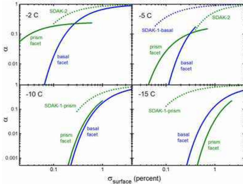
Figure 4.17: The inherent richness of the CAK model, and the attachment kinetics more generally, becomes apparent when displayed as constant-temperature \alpha(\sigma_{surf}) plots. The different “branches” represent different growth regimes identified by their corresponding physical effects. The graph shown for -5 C is particularly noteworthy, as it indicates that both platelike and columnar forms can appear at \sigma_{surf}=0.15\% , a feature that is supported by observations. Plots like these are especially useful for comparing with all different types of ice-growth experiments.
