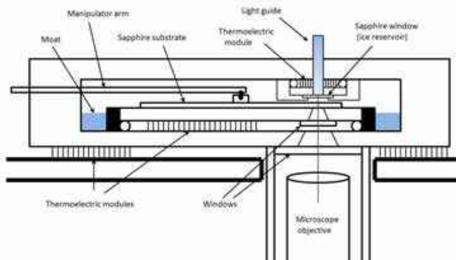
Figure 7.4: (Left) A schematic diagram of the dual-temperature chamber used in [2013Lib] to measure the growth of small ice crystal in near vacuum. Figure 7.5 shows a closer view of the ice-growth region.
