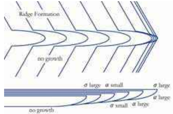
Figure 9.26: Diagrams illustrating the formation of a snow-crystal ridge. In the top sketch, the lines represent molecular terrace edges on the underside of the plate. Each terrace has an overall hexagonal shape, but the corners see a slightly higher supersaturation and are thus unstable to the usual branching instability. The lower sketch shows a side view of the ridge structure. As ice is added to the top surface and the plate edge, the ridge is left behind. Away from the edge, neither the ridge or the surrounding surface experiences any additional growth.
