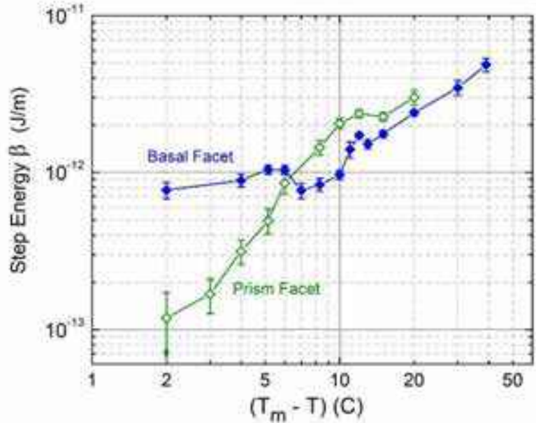
Figure 2.15: Measured ice/vapor terrace step energies (in near-vacuum conditions) for the basal and prism facets as a function of temperature [2013Lib].
