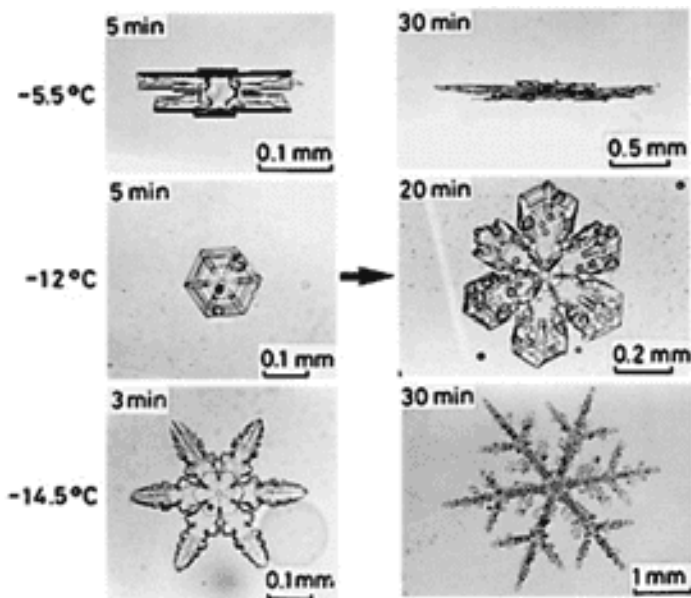
Figure 6.26: Example snow crystals grown in a laminar-flow chamber, from [1999Fuk].
