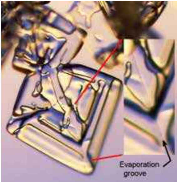
Figure 2.27: Arrowhead Twins Variant I. This photo shows a weak evaporation groove along the twin plane in an arrowhead crystal. The straightness and sharpness of this feature suggests its crystalline origin, in contrast to the other growth features in the crystal. Image by Patricia Rasmussen [2003Lib2].
