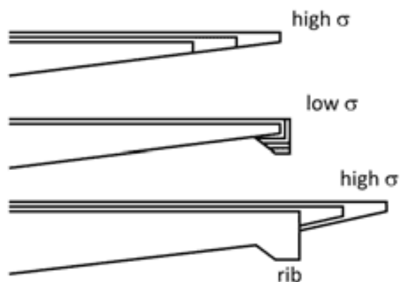
Figure 9.29: The above series of sketches shows a side view of the formation of a rib structure on a PoP snow crystal. The rib forms on the edge of the plate, but is subsequently left behind when the ESI brings about a thinner plate from the top edge of the ridge. Applying this sequence of supersaturation changes several times yielded the multi-rib pattern seen in Figure 9.28.
