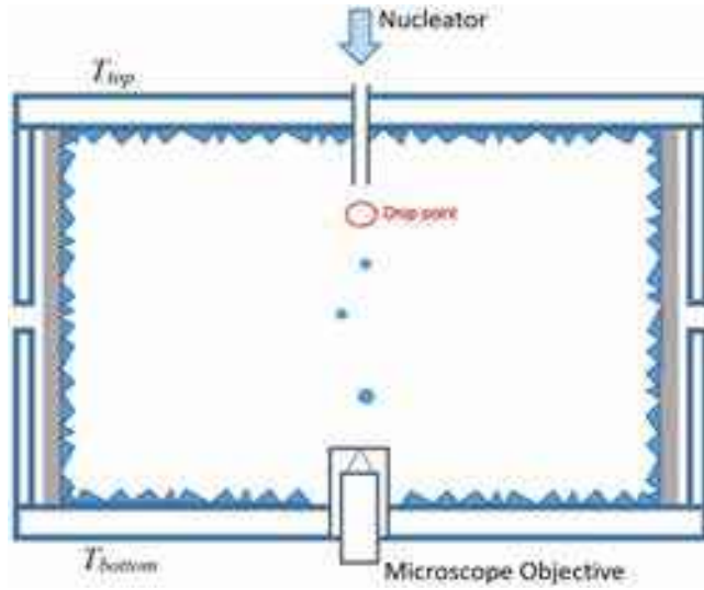
Figure 7.26: A linear-gradient free-fall growth chamber (see Chapter 6) for observing ice growth rates as a function of temperature, supersaturation, and background gas pressure. A nucleator carefully places crystals near the “drop point” shown, and from there they grow and slowly fall onto the substrate for observation. To date, even basic trends in snow-crystal growth morphologies as a function of background gas pressure have been characterized, presenting a sizable gap in our knowledge of the underlying attachment kinetics.
