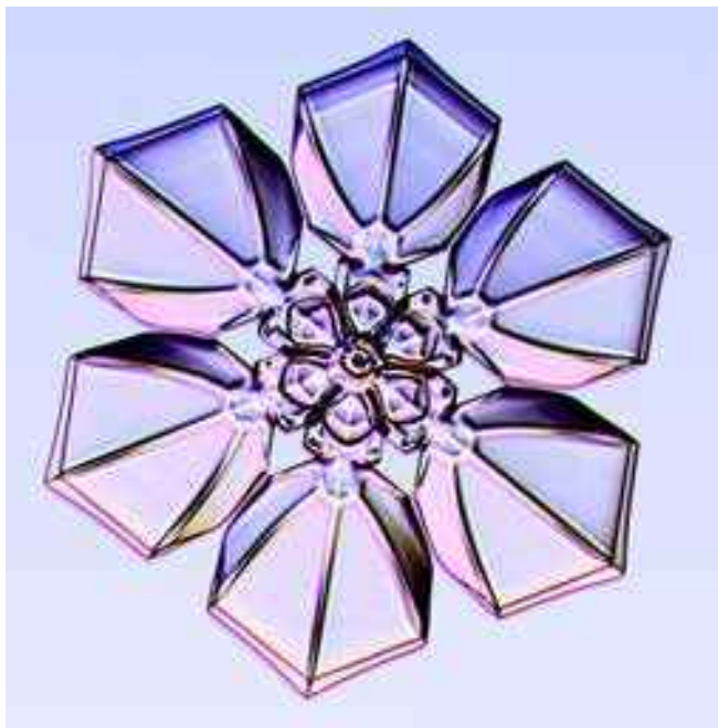
Figure 9.27: (Left) Sectored plate extensions. Curved ridges often form on broad-branched sectored plates, looking a bit like “duck’s feet” in this PoP example. Because ridge formation originates at the faceted corners of a plate, the ridges trace out the location of the corners as a function of time as the crystal developed.
