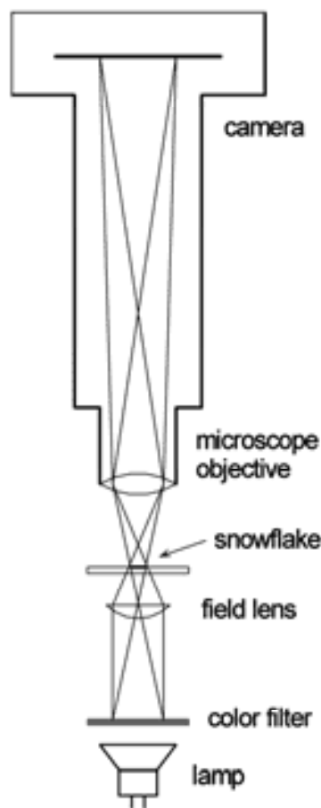
Figure 11.23: This diagram shows the optical layout used for Rheinberg illumination. In addition to the usual camera+lens, the lower field lens images a color filter onto the optical pupil at the microscope objective. This layout yields a uniform background even with a highly patterned color filter.
