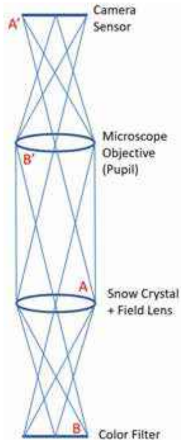
Figure 9.7: (Right) A simplified ray diagram of the optical layout shown in Figure 9.4. Note that the microscope objective images the snow crystal onto the camera sensor ( A \rightarrow A' ), while the field lens images the color filter onto a pupil within the microscope objective ( B \rightarrow B' ).
