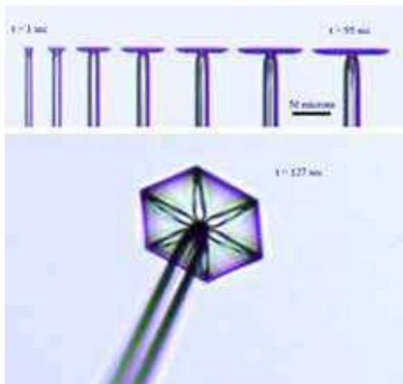
Figure 8.21. Observations of a thin plate-like snow crystal growing on the end of an ice needle, as seen from the side (top set of images) and from a more face-on direction (bottom). The crystal grew at a temperature of -15 C with a supersaturation at the center of DC2 of about 11 percent.
