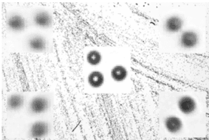
Figure 11.13: (Left) A photograph of a glass substrate sprinkled with 10- \mu\text{m} glass beads, imaged with a Mitutoyo Plan APO 5X objective. The total field of view is about 5x4 millimeters, and the inset images show magnified snippets of the main image taken from the center and the four corners. The focus was set to best image the center beads, which resulted in somewhat out-of-focus beads in the corners. Combining several images using focus stacking yielded a sharp focus across the entire image.
