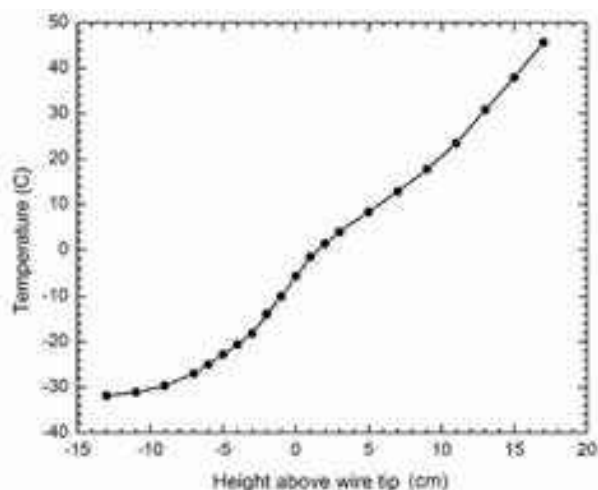
Figure 8.12. A measurement of the temperature profile along the central vertical axis in DC1. The parameters of the DC1 design, particularly the lengths of the upper and lower clam-shell walls, were adjusted to produce an especially high supersaturation and a temperature of -6 C at the location of the wire tip ( z = 0 in the graph). Note the especially steep dT/dz at this position.
