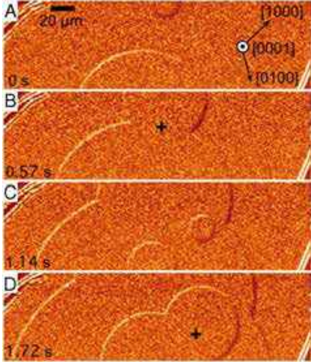
Figure 6.20: Photomicrographs of terrace steps on the basal face of an ice crystal that display the nucleation and growth of new terraces [2010Saz].
