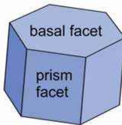
Figure 1.7: The most basic shape of a snow crystal is a hexagonal prism with two basal facets and six prism facets. This shape arises because of the underlying hexagonal structure of the ice crystal lattice, as described in Chapter 2.
