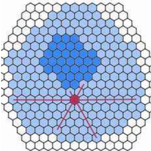
Figure 5.29: This diagram of several basal terraces shows a topmost “upper” basal terrace in dark blue, the next lowest terrace in light blue, and the terrace below that in white. The red cell illustrates a representative boundary pixel that lies atop the light-blue terrace. Counting the number of same-terrace boundary pixels in the six directions shown yields the L_i vector [-1, -2, +7, +5, +4, +7] .
