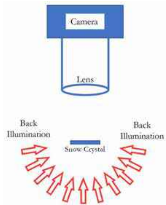
Figure 11.21: Back Illumination. With this method, a snow crystal is photographed using light transmitted through the clear ice. It requires placing the crystal on a transparent substrate, typically a glass microscope slide, and it is best implemented using a rigid mounting system. Many illumination effects can be achieved by modifying the direction, intensity, and color of the illumination.
