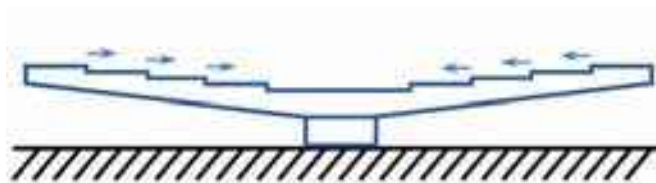
Figure 9.32: A sketch illustrating the side view of a (hypothetical) simple PoP crystal exhibiting inwardly propagating steps. Because water vapor is supplied from above, the plate grows outward and slowly upward, giving the upper basal surface a slightly concave morphology.
