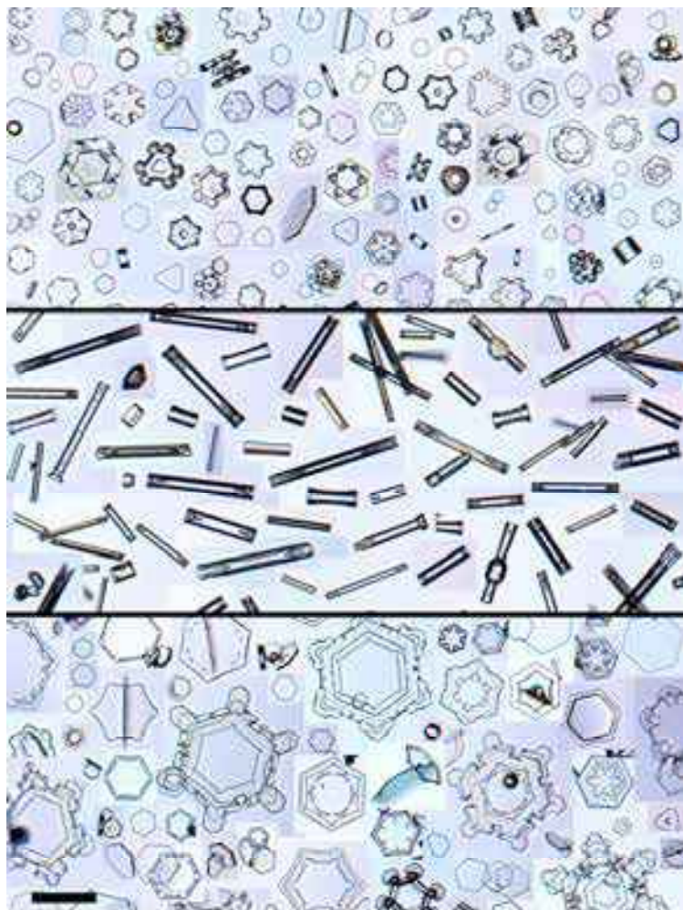
Figure 6.25: Examples of snow crystals grown in a free-fall convection chamber at temperatures of -2 C (top), -5 C (middle) and -15 C (bottom). The scale bar in the lower left corner of the image is 50 microns in length. The variation in crystal size and morphology at each temperature reflects inhomogeneities in temperature and supersaturation within the chamber. Overall, however, the morphologies agree with expectations from the snow-crystal morphology diagram.
