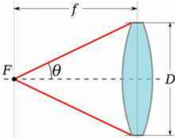
Figure 11.10: This sketch defines the focal length f , the lens aperture D , and the half-angle \theta for a simple microscope objective.
