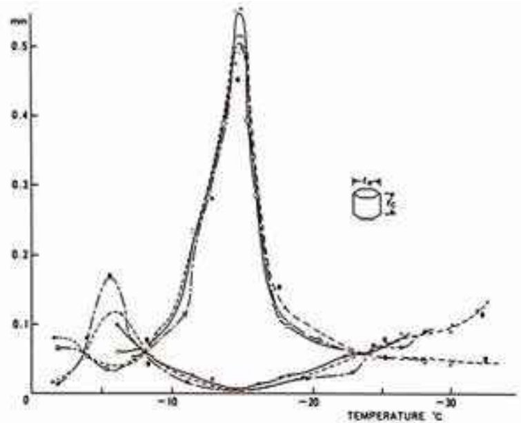
Figure 6.22: Measurements of the diameters and thicknesses of snow crystals after growing in air for 200 seconds in a free-fall cloud chamber [1987Kob]. Note that the variation in crystal aspect ratio as a function of temperature matches expectations from the snow crystal morphology diagram.
