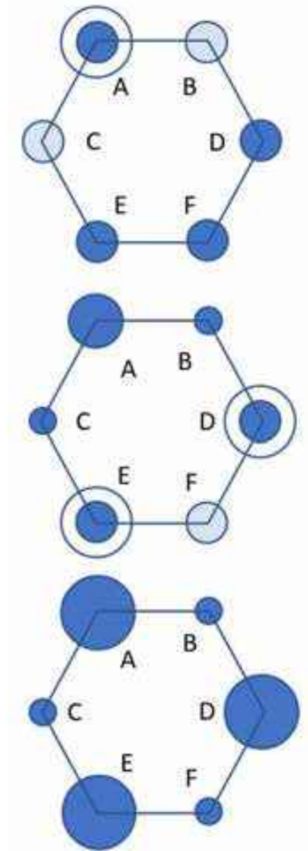
Figure 3.63: Trident Formation. (Top) If one of six primary branches (branch A) extending from a columnar crystal becomes a bit taller than the others, then the Mullins-Sekerka instability will enhance its growth, while its immediate neighbors (branches B and C) will be shielded. (Middle) As branch A grows taller and branches B and C are left behind, D and E will be more exposed to the supersaturated air and will thus grow faster, shielding branch F. (Bottom) In time, branches A, D, and E will dominate while B, C and F are strongly shielded, yielding a trident-shaped crystal.
