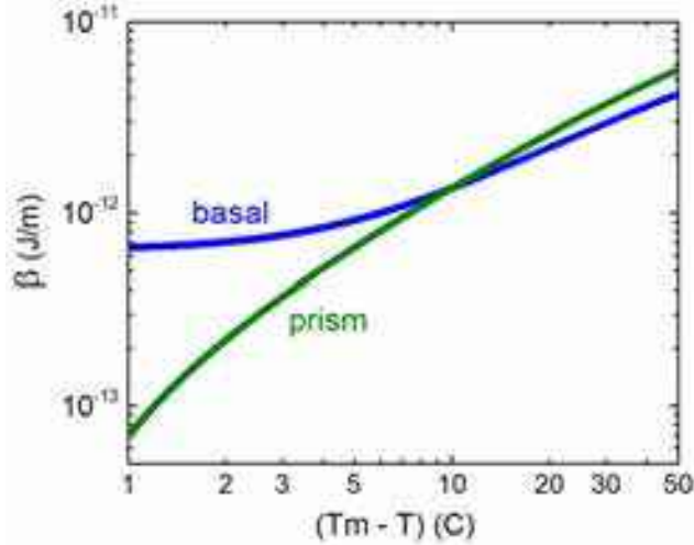
Figure 4.6: These curves show CAK model estimates for the step energies \beta(T) for large basal and prism facets as a function of temperature, extracted from \sigma_0(T) using Equation 4.5. While derived from dynamical growth measurements, these step energies represent fundamental equilibrium properties of the ice crystal surface.
