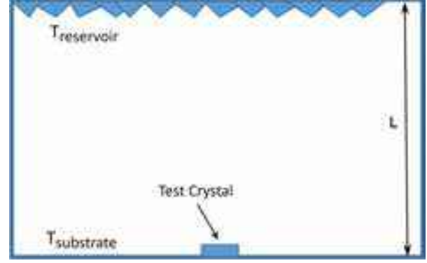
Figure 7.1: A schematic layout of a basic ice-growth experiment. The single test crystal being measured rests on an isothermal substrate at temperature T_{\text{substrate}} , and no other ice crystals are present on the substrate. Water vapor is supplied by a large collection of frost crystals on the top of the chamber at temperature T_{\text{reservoir}} . The walls are free of ice crystals and have a relatively low thermal conductivity.
