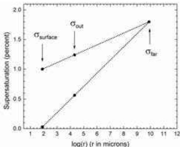
Figure 8.31. A simple analytical model showing the supersaturation field \sigma(r) surrounding an infinite cylinder. The bottom line assumes a fairly large \alpha_{vicinal} at the surface, while the top line assumes a much smaller \alpha_{prism} at the surface. Changing the value of the attachment coefficient has a large effect on the supersaturation near the crystal surface.
