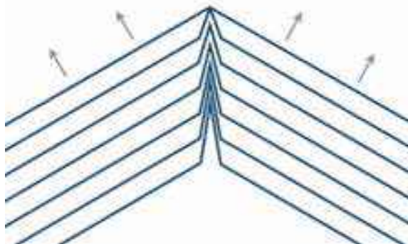
Figure 3.42: A sketch showing the development of a snow-crystal ridge on a convex basal surface. Lines represent molecular steps defining individual terraces. As the prism facet edges grow outward (arrows), diffusion enhances the growth of the terrace corners, leading to ridge formation. This terrace-branching model naturally explains why ridges are generally associated with convex basal surfaces.
