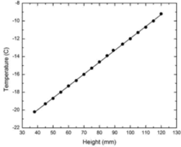
Figure 8.14. Measurements of the vertical temperature profile in DC2. Unlike in DC1, this temperature profile holds near the walls and throughout the interior of the chamber. As a result, there are no horizontal temperature gradients inside the chamber, so the air is stable against convection. This stability allows precise modeling of the supersaturation within the chamber.
