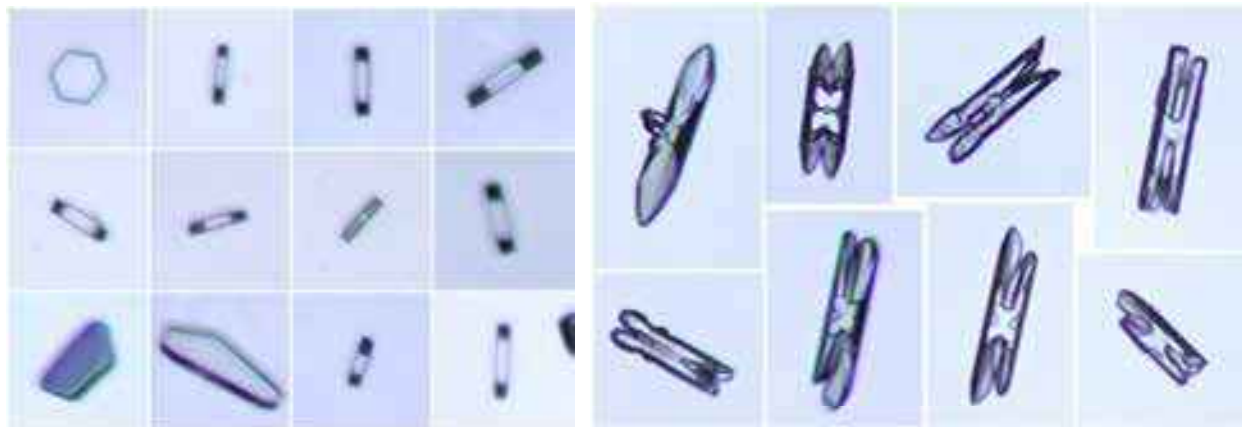
Figure 4.19: Left: A selection of thin platelike crystals growing at -5\text{ C} at low pressure in the VPG apparatus with \sigma_{surf} \approx 0.1 percent. These examples illustrate that quite thin plates can be grown at -5\text{ C} . Right: Several hollow columnar crystals grown in air at -5\text{ C} using the VPG apparatus. Although the overall morphologies are distorted by their intersection with the substrate, it appears that the Edge-Sharpening Instability is largely responsible for the formation of thin basal edges on these crystals.
