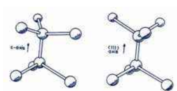
Figure 2.4: The essential lattice difference between hexagonal ice Ih (left) and cubic ice Ic (right) is a twist in some of the bonds, specifically those between the basal layers in ice Ih. Here the balls and sticks represent oxygen and hydrogen atoms, respectively.
