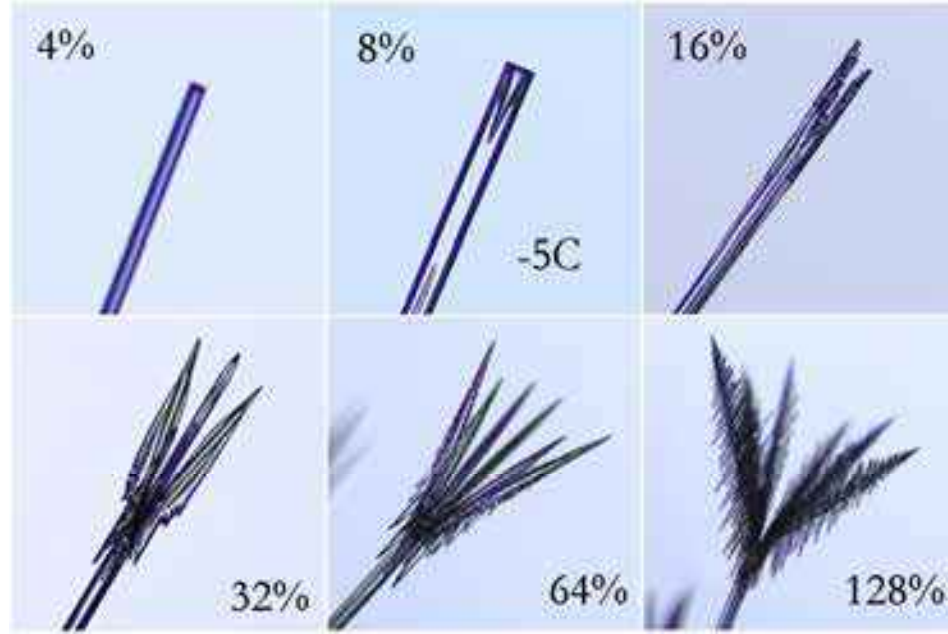
Figure 4.20: Several examples of crystals growing at -5 C in air on the ends of “electric” ice needles (Chapter 8). Each image is labeled with the supersaturation \sigma_\infty far from the needle tip. At 4%, the initial needle thickens to form a solid column with slight basal hollowing, while hollow-column growth develops quickly at 8%. At 16%, a hollow column has split to form needle clusters. At 32%, trident structures are common (Chapter 3). At 64% and 128%, fishbone dendrites (Chapter 3) exhibit rapid growth.
