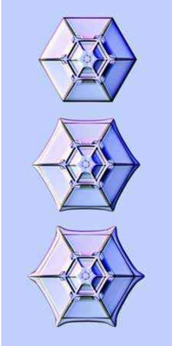
Figure 3.5: This series of photographs shows branches sprouting from the six corners of a hexagonal snow crystal when the applied supersaturation was increased. Branching like this becomes more likely when a hexagonal crystal is large and/or its growth rate is fast.
