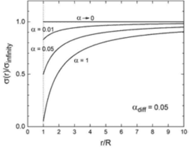
Figure 3.19: The solution to the diffusion equation for the growth of a spherical snow crystal with \alpha_{diff}=0.05 . When \alpha \rightarrow 0 , the growth is kinetics limited and \sigma_{surf} \approx \sigma_{\infty} . Then as \alpha increases, the growth becomes more diffusion limited and \sigma_{surf} decreases.
