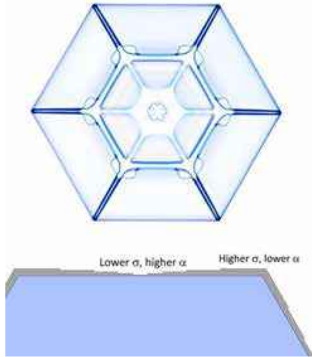
Figure 3.4: The prism facets on this POP snow crystal (top photo) look straight, but they must be slightly concave at the molecular scale (bottom sketch). The hexagonal corners stick out farther into the humid air, so \sigma is slightly higher at the corners than at the facet centers. At the same time, the density of molecular terrace steps is higher nearer the facet centers, making \alpha slightly higher there (the surface lines in the sketch represent molecular layers). Because the growth rate is proportional to \alpha\sigma , the entire facet surface grows upward at a constant rate, maintaining its flat appearance.
