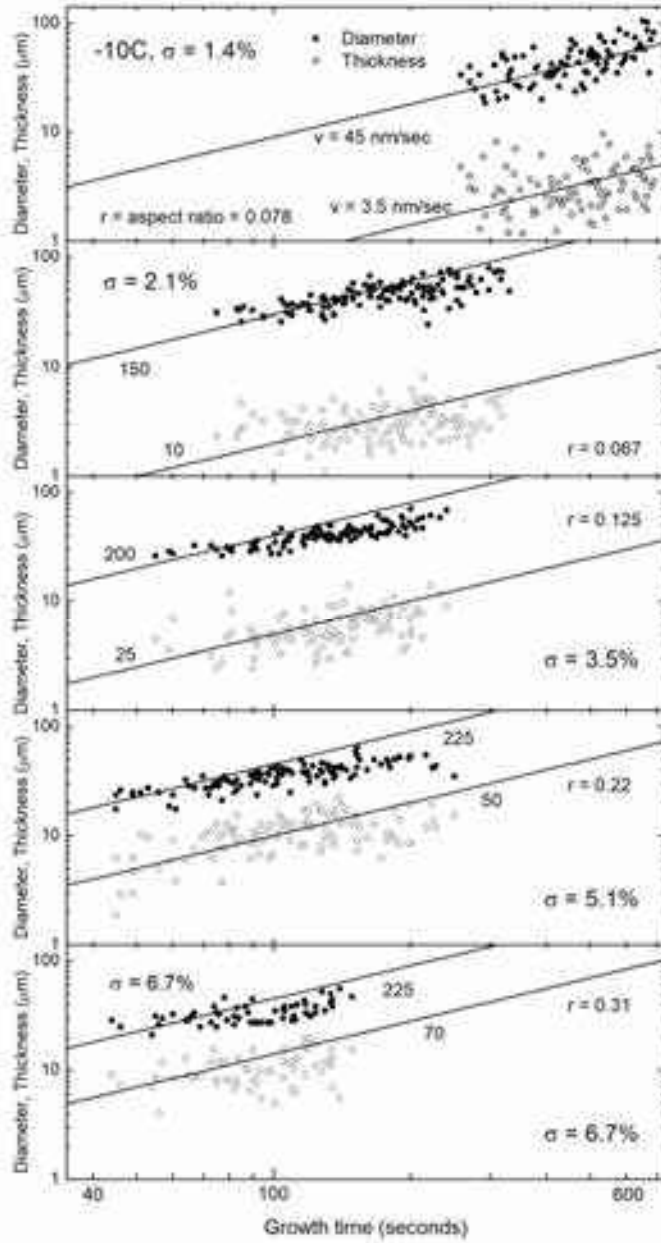
Figure 7.23: Free-fall growth data at -10 C from [2009Lib], showing crystal sizes as a function of fall times for several different supersaturations (here \sigma = \sigma_\infty , which is generally not equal to \sigma_{surf} ). Each pair of points (diameter and thickness) represent one observed crystal. Lines show constant-velocity trajectories, and the aspect ratio is the ratio of these velocities. Note that the aspect ratio tends toward unity with increasing supersaturation.
