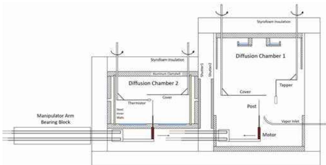
Figure 8.10. A dual diffusion chamber apparatus for observing snow crystal growth on electric ice needles. Diffusion Chamber 1 (DC1, on the right) provides the necessary conditions for creating c-axis electric needles easily and quickly. The needles are then transported to Diffusion Chamber 2 (DC2, on the left), which provides a well-controlled environment that can achieve a broad range of temperatures and supersaturation levels. The inside height of DC2 is 10 centimeters [2014Lib].
