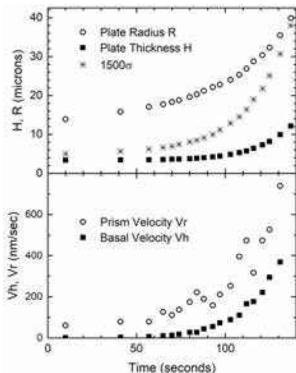
Figure 7.11: (Top) A typical growth sequence for a single thin-plate crystal at -12\text{ C} , like the one shown in Figure 7.8. As the supersaturation is slowly increased by increasing \Delta T , the plate thickness H is measured using white-light interferometry while the plate “radius” R (here defined as half the distance between opposing prism facets) is measured from direct imaging. Note R > H , indicating a thin, plate-like crystal. (Bottom) Growth velocities of the basal and prism facets derived from the size data above. The higher accuracy of the interferometric measurements yields a lower noise in the basal radius and velocity data.
