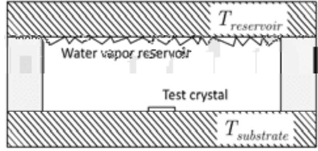
Figure 6.9: This dual-temperature chamber contains a layer of ice that acts as a water-vapor reservoir along with an ice test crystal to be measured. Both the reservoir and test-crystal surfaces are carefully temperature regulated. The supersaturation around a small test crystal is easily calculated from the two temperatures, going to zero when there is no temperature difference between the top and bottom surfaces.
