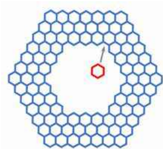
Figure 3.36: A diagram of the end of a fictitious nanoscopic hollow columnar snow crystal, with hexagons representing molecular cells in the ice lattice. While a nucleation barrier prevents growth of the outer faceted surfaces, there is no nucleation barrier on the inner surfaces because molecules can always attach at interior corners (red hexagon).
