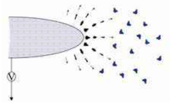
Figure 8.5. When a high voltage is applied to an ice needle, strong electric fields (arrows) are concentrated at the tip. As described in the text, these fields decrease the equilibrium water-vapor pressure near the tip, increasing its growth rate. This produces a positive feedback effect: faster growth yields a sharper tip, which increases the electric fields near the tip surface, making the growth faster still. The result is a runaway growth instability that produces a slender, fast-growing e-needle.
