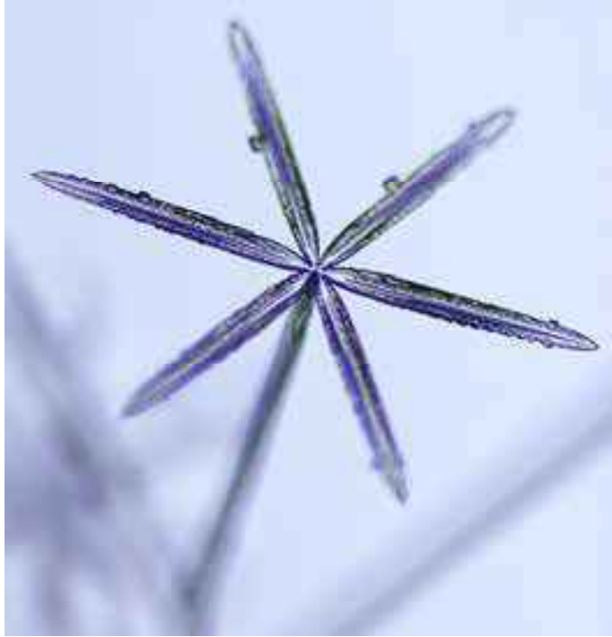
Figure 3.30: Simple stars present a case where large-scale morphology is directed by an unusual characteristic of anisotropic attachment kinetics. Rounding near the branch tips indicates \alpha_{prism} \approx 1 on the outermost prism surfaces, but faceting on the branch sides indicates \alpha_{prism} < 1 on those prism surfaces. This difference explains why sidebranching is suppressed on this crystal. The Edge-Sharpener Instability (see Chapter 3) may be present at the branch tips, although high-fidelity 3D numerical simulations will likely be needed to fully understand this seemingly simple morphology.
