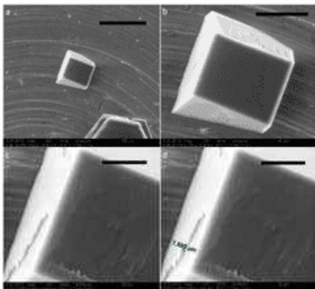
Figure 6.18: Several ESEM images of a simple prismatic ice crystal that reveal fine surface structures, such as the 1.6 \mu\text{m} step seen in the lower right image. The black scale bars are 100, 40, 20, and 20 \mu\text{m} long (adapted from [2014Mag]).
