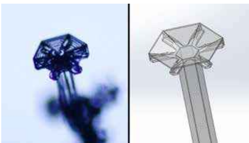
Figure 3.48: I-Beams. The photo on the left shows a snow crystal growing on an e-needle near (T, \sigma) = (-9^{\circ}\text{C}, 16\%) , and its overall structure is illustrated in the drawing on the right. Here the plate has an intermediate cone angle, yielding short fin-ridges that subsequently developed plate-like extensions, giving an overall “I-beam” ridge structure. This morphology is remarkably robust on e-needles, occurring over a broad range of growth conditions (see Chapter 8). [SolidWorks drawings by Ryan Potter.]
