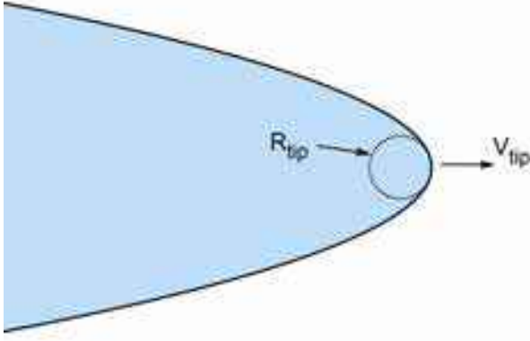
Figure 12.10: The Ivantsov solution to the diffusion equation describes a crystalline paraboloid of revolution with an unchanging parabolic shape and a constant tip radius R_{tip} , the entire structure growing forward with a constant tip velocity v_{tip} . If viewed from a frame of reference that moves in the growth direction with velocity v_{tip} , the system would appear completely static.
