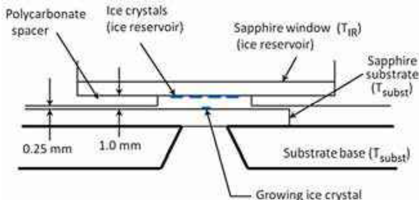
Figure 7.5: (Left) A close-up view of the ice-growth region of the apparatus in Figure 7.4, showing the ice reservoir and test crystal. Note the similarities to the ideal growth-chamber geometry shown in Figure 7.1.
