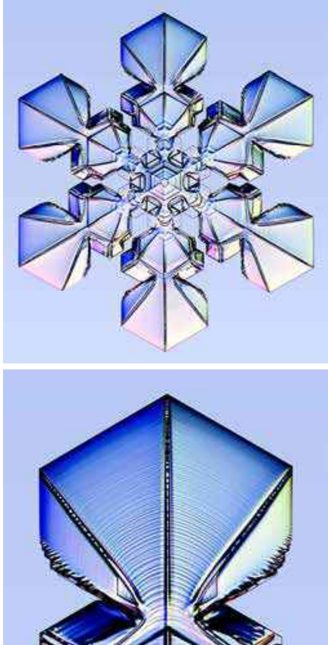
Figure 3.49: The upper photo shows a large laboratory-grown POP snow crystal, while the lower photo shows a close-up of a single sectored-plate branch. Molecular steps on the top basal surface nucleate near the outer edge of the crystal and subsequently grow toward the center. The molecular steps bunch together to produce a series of inward-propagating ring-like features. Near-constant growth conditions are required to produce such a uniform set of growth rings.
