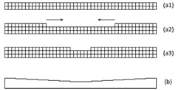
Figure 5.21: The growth of shallow concave basal surface is difficult to reproduce with good accuracy in a cellular-automata model. In the model (a1,a2,a3), a new terrace nucleates at the edges of the plate and then grows inward. In real life (b), there is a continuous series of terraces that nucleate at the plate edge and propagate inward.
