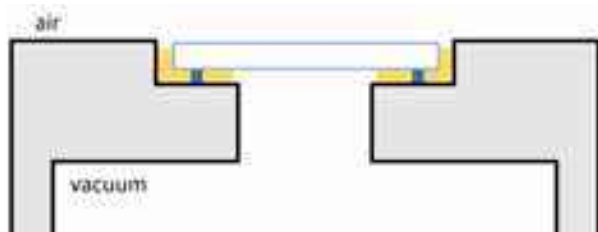
Figure 6.8: A simple and inexpensive, yet quite effective, design for attaching an optical-quality vacuum window to a vacuum flange. The large-area flat-against-flat adhesive seal (yellow) works well for preventing vacuum leaks. Spacers (blue) keep the adhesive layer thick, so it can flex during thermal cycling without losing adhesion.
