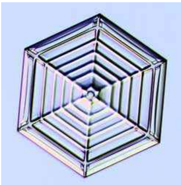
Figure 9.28: The “spider-web” pattern on this small PoP crystal was created by inducing a series of evenly spaced rib structures. Each hexagonal rib was created by lowering \sigma for about thirty seconds to thicken the plate edge, and then raising \sigma back up again to continue the thin-plate growth. Both ribs and ridges form on the undersides of PoP plates, as shown in Figure 9.29.
