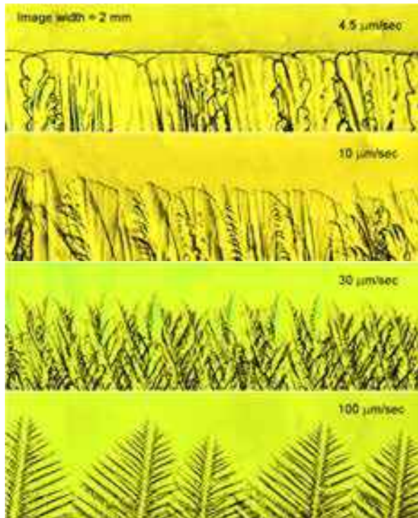
Figure 12.16: Several photographs of ice growing in water held between two closely spaced ( \sim 200\ \mu\text{m} ) plastic plates. The plates were pulled at constant velocities (shown) between hot and cold regions, creating a temperature gradient from top (warm) to cold (bottom) within each panel.
