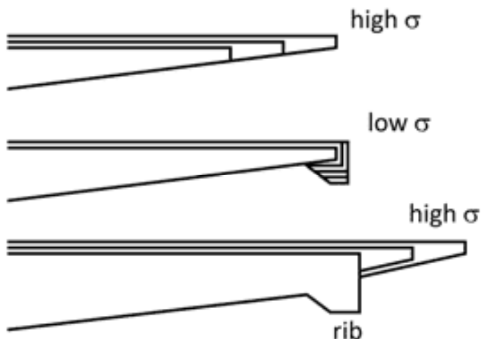
Figure 3.53: This series of sketches chronicles the formation of a snow-crystal rib on the underside of a POP snow crystal. When the supersaturation is high (top), thin-plate growth results. Upon lowering the supersaturation (middle), the crystal grows more slowly, and its edge develops a thick rim. Restoring high supersaturation (bottom), thin-plate growth commences from the upper edge of the rim, leaving a rib structure behind on the underside of the plate.
