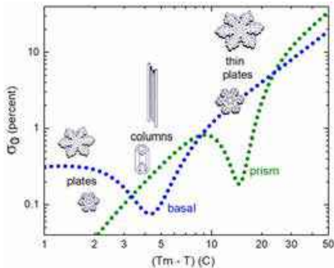
Figure 4.13: Plotting the SDAK curves from Figure 4.12 together, we can compare the basal and prism nucleation barriers as a function of temperature. A lower nucleation barrier (i.e., a lower \sigma_0 ) means faster attachment kinetics on the corresponding facet surface. This demonstrates that the CAK model exhibits the same transitions between platelike and columnar growth that are seen in the Nakaya diagram (Chapter 1). Beyond this qualitative agreement with morphologies, however, the CAK model also provides good quantitative agreement with many precision ice-growth measurements [2019Lib2, 2020Lib].
