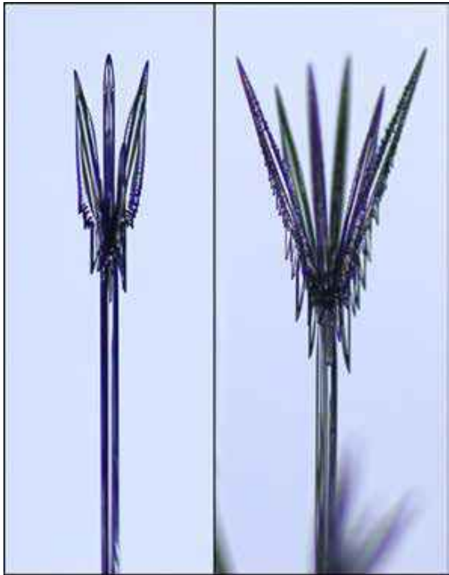
Figure 3.62: (Left) A “trident” snow crystal forming on the end of an ice e-needle (see Chapter 8) in air with (T, \sigma) = (-5\text{ C}, 32\%) . Starting from a hexagonal column, only three branches grew to a discernable length. (Right) A similar crystal growing with (T, \sigma) = (-5\text{ C}, 64\%) . In this case the opening angle between the branches is larger and all six grew out from the initial columnar crystal.
