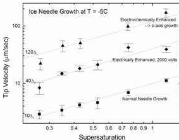
Figure 8.7. Experimental measurements (data points) showing the tip velocities for normal needle growth (lower points), e-needles growing along crystalline axes that are not the c-axis (middle points), and c-axis e-needles (upper points). The data were all taken at a temperature of -5 C, and in all cases the tip growth velocity is linearly proportional to the supersaturation, as predicted by solvability theory (see Chapter 3). Growth along the c-axis was stimulated using chemical vapor additives as described in this chapter. From [2002Lib].
