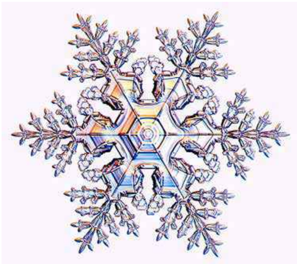
Figure 4.3. Facet-Dominated Growth. The attachment kinetics on any snow crystal can be divided into three classes of surfaces: top basal terraces described by \alpha_{basal} , top prism terraces described by \alpha_{prism} , and all other surfaces described by \alpha \approx \alpha_{rough} \approx 1 . The overall platelike structure of this crystal, as well as much of its dendritic branching, is determined by the first two surface classes. Thus, the attachment kinetics on the topmost facet terraces strongly influences the morphological development of the entire structure.
