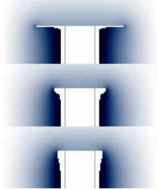
Figure 5.22: An illustration of the Gibbs-Thomson effect in a cylindrically symmetric CA model of a plate growing from the edge of a column [2013Lib1]. With zero surface energy (top), a one-pixel-thick ( 0.15 \mu\text{m} ) plate grows from the edge of the column, which is not a physically plausible solution. A Gibbs-Thomson length of d_{sv} = 0.3 \text{ nm} (middle) or d_{sv} = 1 \text{ nm} (bottom) suppresses the thin-plate growth. Vertical lines show the original seed crystal, while the supersaturation around the crystal is proportional to the image brightness.
