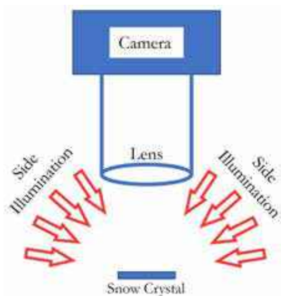
Figure 11.16: Side illumination. In this straightforward method, light shines in from the side to illuminate the snow crystal, and scattered light enters the lens and is focused onto the camera sensor.
