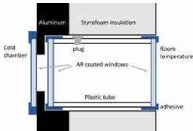
Figure 6.7: A sketch showing a viewport cell installed into the wall of a cold chamber. This design allows optical access while minimizing heat flow into the chamber and preventing condensation of water vapor from the room.
