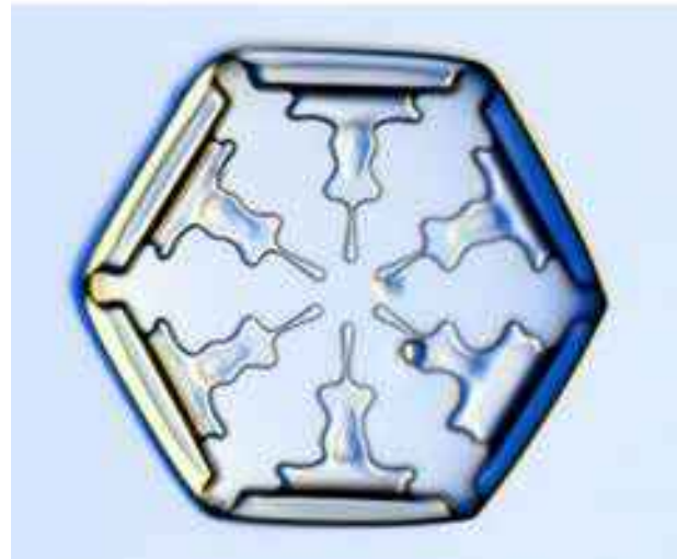
Figure 3.37: The essential geometry of a hollow-plate snow crystal (top) and a photograph of a natural snow crystal with deep hollows. Note that the six hollow regions are separated by solid ice at the hexagonal corners. The photo exhibits oddly shaped hollow regions reflecting the changing conditions that the crystal experienced during its growth.
