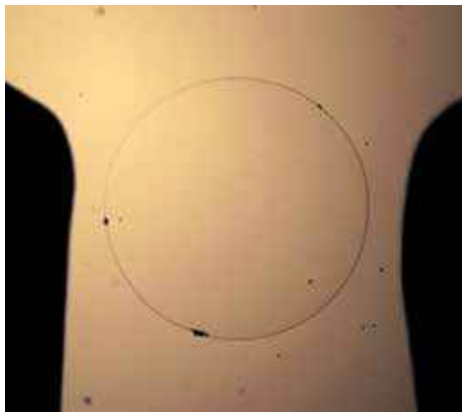
Figure 6.11: A 2-mm-diameter disk of ice grows outward on the surface of a thin film of slightly supercooled water covering a glass plate. (The dark regions are copper support arms glued to the glass.) The c-axis of the oriented ice crystal is aligned perpendicular to the glass surface.
