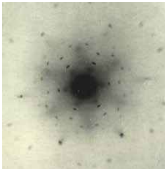
Figure 1.19: This X-ray diffraction pattern was made by a block of ice, used by William Barnes to derive the hexagonal lattice structure of the ice crystal [1929Bar].
