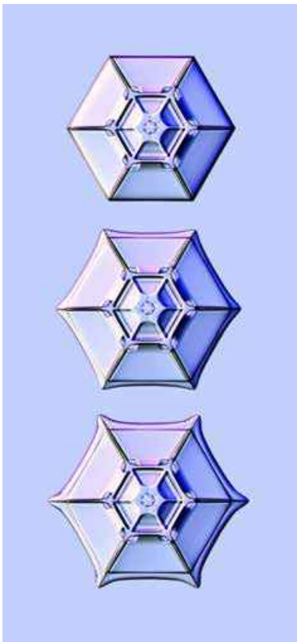
Figure 9.18: After growing a simple hexagonal PoP crystal at -12.5 C (top), the substrate temperature was reduced to -15 C to stimulate branching. At first the outer edge of the plate became thinner (middle), and then branches sprouted from the six corners of the hexagon (bottom). Note that the plate is supported above the substrate by the central ice pedestal, and the observed surface patterning is all contained on the underside of the plate. The top basal facet, in contrast, is essentially perfectly flat over the entire crystal.
