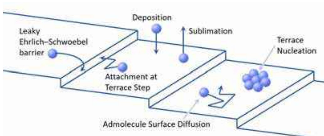
Figure 4.2: The attachment kinetics are governed by a variety of molecular processes occurring on the surface of a growing crystal, including those illustrated here.
