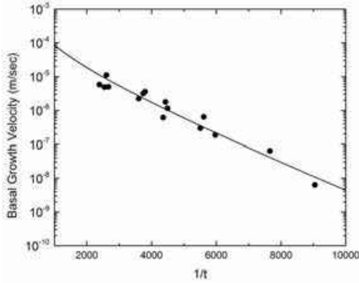
Figure 12.8: Measurements of the basal growth velocity for ice in liquid water as a function of the dimensionless undercooling t = (T_m - T_{surf})/T_{surf} . The line through the data shows a terrace-nucleation model with an ice/water basal step energy of \beta_{sl,basal} \approx 5.6 \times 10^{-13} J/m [1958Hil, 2014Lib, 2017Lib].
