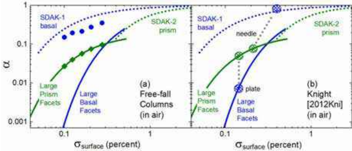
Figure 4.23: Additional snow-crystal growth data obtained at a fixed temperature of -5 C [2020Lib2]. (a) Data from a free-fall growth chamber, again analyzed using the witness-surface method. (b) A rough analysis of observations in [2012Kni] that demonstrated the simultaneous growth of platelike and needle structures at -5 C. The data can also be explained using the CAK model, albeit with substantial experimental uncertainties. Together with Figures 4.18 and 4.21, these data exhibit a remarkably diverse range of growth behaviors, and all can be reasonably well explained with the CAK model.
