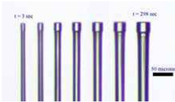
Figure 8.26. Observations of a blocky snow crystal growing on the end of an ice needle at a temperature of -15 C with a far-away supersaturation of about 4.6 percent.
