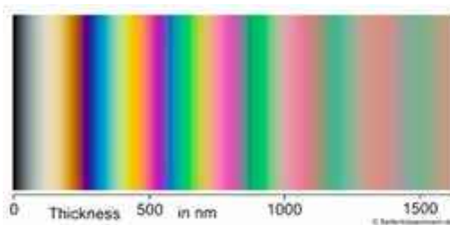
Figure 11.19: The calculated interference colors for white light reflecting off a thin soap film, as a function of the thickness of the film in nanometers. Factoring in the index of refraction, the thickness of an internal air cavity in ice is roughly 1.3 times larger than the soap-film thickness with the same interference color. The calculation will change somewhat depending on the camera color response and the spectrum of the light source. Image from soapbubble.fandom.com/wiki/Color_and_Film_Thickness .
