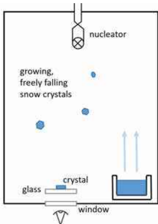
Figure 6.23: A free-fall convection chamber. The expansion nucleator near the top of the chamber (described in Figure 6.8) produces microscopic seed crystals that subsequently grow and slowly fall in the supersaturated air. After a few minutes of growth, the crystals fall to the bottom of the chamber, where some land on a glass substrate for observation.
