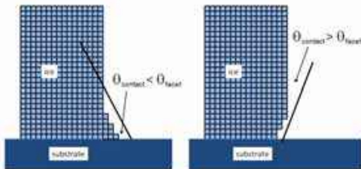
Figure 6.12: If the ice/substrate contact angle is less than the facet/substrate angle (left sketch), then new terraces will be nucleated at the ice/substrate contact line. With a larger contact angle (right sketch), new terrace nucleation can only occur on the free faceted surface, away from the contact region. The enhanced terrace nucleation in the first case can greatly increase the growth rates of facets contacting the substrate.
