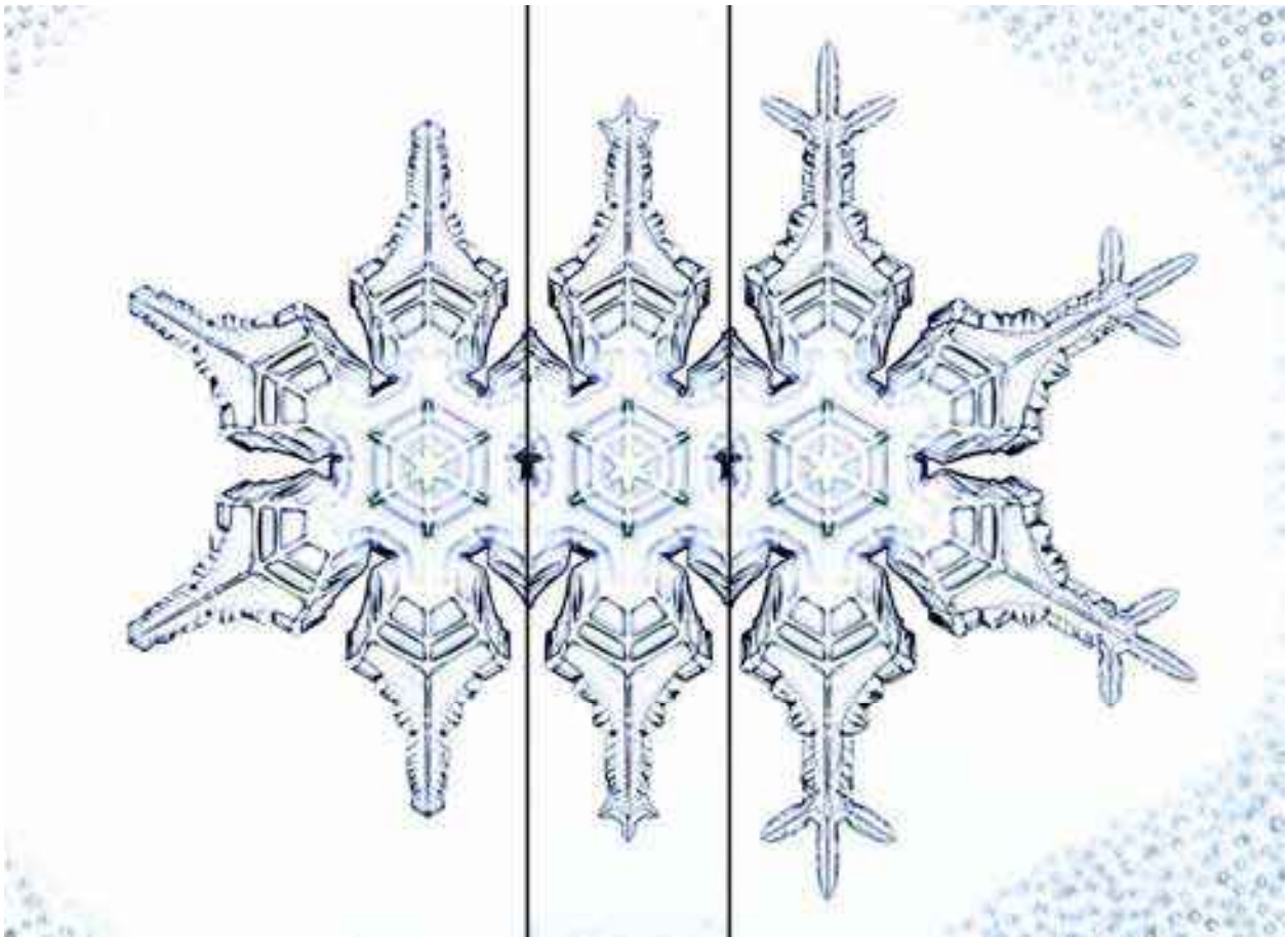
Figure 9.23: The process of induced sidebranching is illustrated in these three photos of a growing PoP snow crystal. After growing a set of six primary branches, the supersaturation was lowered so the branch tips became faceted (left photo). Once the three outermost facet corners were well developed, the supersaturation was abruptly increased, causing branches to sprout from these corners (center). Keeping the supersaturation high, the primary and side branches all continued to grow outward at about the same rate (right).
