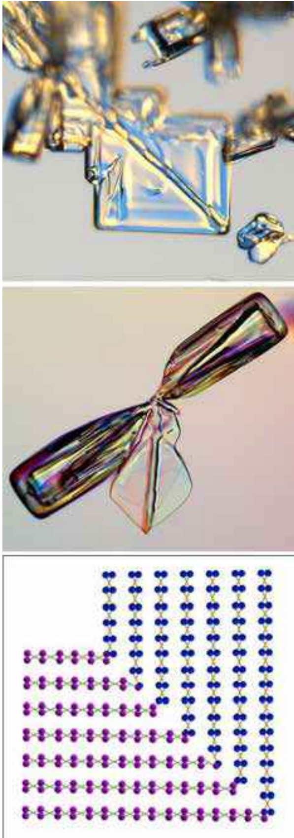
Figure 2.29: (Left) Arrowhead Twins Variant III. This variant of an arrowhead twin displays an apex angle that is close to 90 degrees, and the model structure shown in the sketch has a theoretical value of 2 \tan^{-1}(3c_0/5a_0) = 88.7 degrees. There are few quality photographic examples of this arrowhead variant, and no laboratory-grown specimens. Nevertheless, to the limits of what has been measured, this model is in good agreement with observations. Images by Patricia Rasmussen [2003Lib2].
