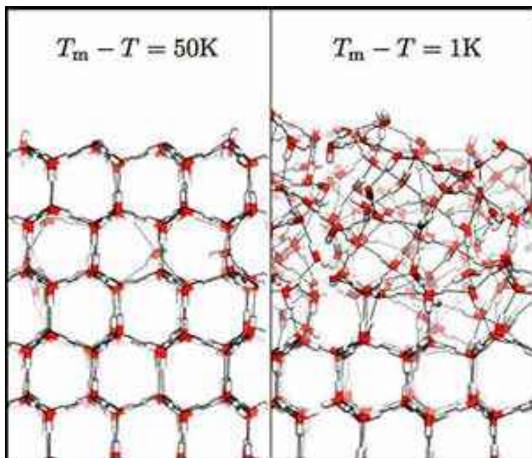
Figure 2.12: A molecular-dynamics simulation from [2014Lim] demonstrating surface premelting. At temperatures far below the melting point (left), the bulk lattice structure persists all the way up to the surface (here showing an edge-on view of a basal facet). Near the melting point, however, the top molecular layers lose their ordered structure, forming an amorphous premelted layer, also called a quasi-liquid layer (QLL).
