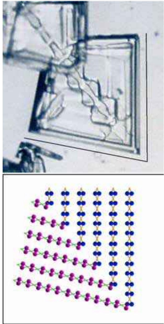
Figure 2.26: Arrowhead Twins Variant I.
