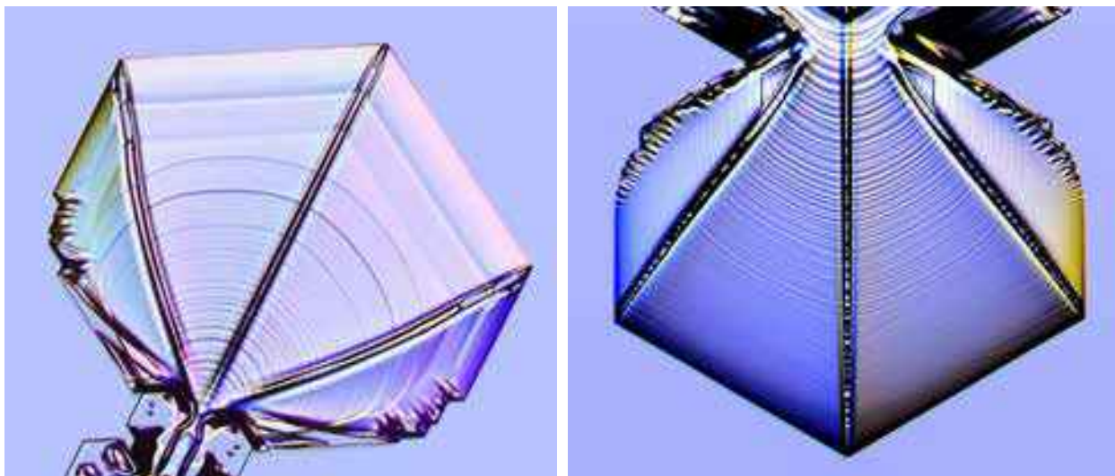
Figure 9.31: Large sectored-plate extensions on PoP snow crystals often exhibit concentric-ring patterns like those seen in these two examples. The rings propagate inward slowly as the plates grow, and they are located on the top basal surfaces, as sketched in Figure 9.32. Ridges and faint ribs can also be seen, and both these features are located on the lower plate surfaces.
