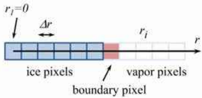
Figure 5.15: The radial layout of cells (a.k.a. pixels) for a one-dimensional spherical cellular-automaton model. At any given time, the model consists mainly of ice pixels (blue) and vapor pixels (white). The red “boundary” pixel is a vapor pixel that neighbors an ice pixel.
