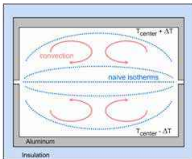
Figure 6.32: A “clam-shell” diffusion chamber designed to create a high supersaturation level at the center of the chamber. Unfortunately, the system is unstable to convection, making it quite difficult to accurately characterize the temperature and supersaturation within the chamber.
