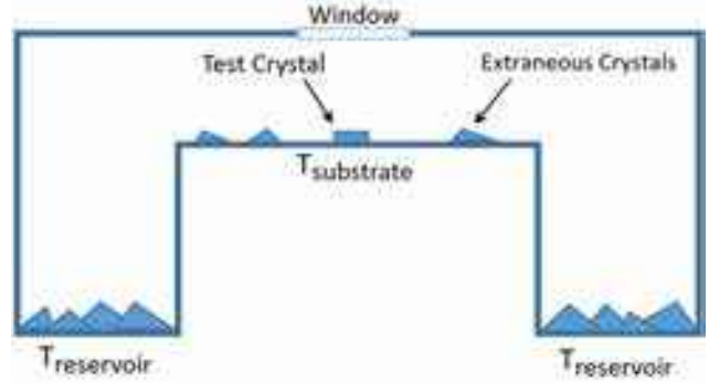
Figure 7.3: An example of a poor chamber design for making precision ice-growth measurements. The presence of extraneous ice crystals on the substrate, coupled with the ice reservoir being far from the test crystal (making L large in Equation 7.6), make it nearly impossible to determine the supersaturation near the test crystal with reasonable accuracy.
