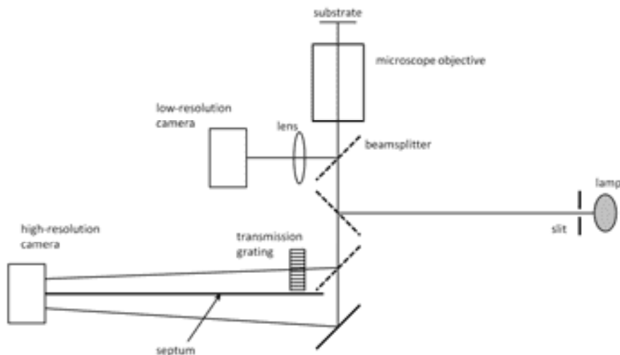
Figure 7.7: The optical layout for observing the growth of a test crystal. The substrate and microscope objective are the same as in Figure 7.4. As described in the text, the low-resolution camera is used for finding and positioning a test crystal, while the high-resolution camera records a direct image of the test crystal along with a broadband interferometer signal used to measure the crystal thickness.
