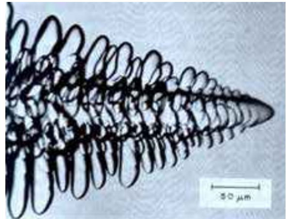
Figure 3.15: A free dendrite forming in succinonitrile from its melt [1976Gli]. This transparent material is often used as a metal analog in studies of solidification, as it forms dendritic structures that are typical for solidification from the melt when attachment kinetics is not an important factor.
