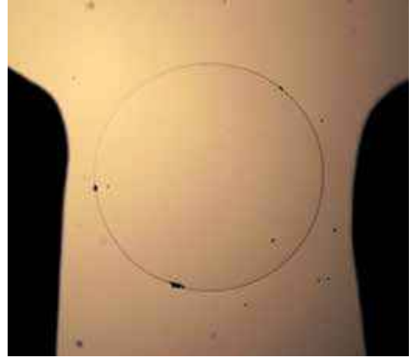
Figure 12.2: A 2-mm-diameter disk of ice grows outward on the surface of a thin film of slightly supercooled water covering a glass plate. (The dark regions are copper support arms glued to the glass.) The c-axis of the oriented ice crystal is aligned perpendicular to the glass surface. It appears that the close proximity of the cold support plate stabilizes the circular shape against dendritic branching.
