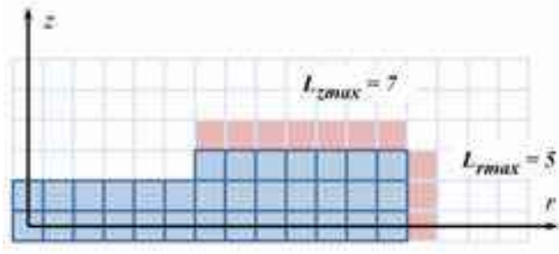
Figure 5.23: A CA model in which the “outer” basal and prism boundary pixels are shown in pink. These pixels represent upper terraces with no adjoining kinks sites, and the terrace widths can be used to roughly estimate the edge curvature for including the Gibbs-Thomson effect.
