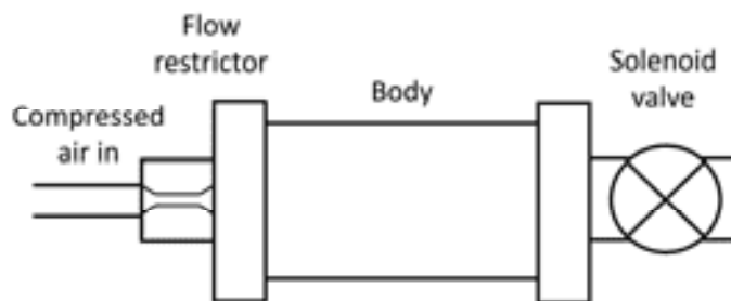
Figure 6.10: An expansion nucleator for creating small ice crystals, consisting of a 5-cm length of pipe (body) flanked by a narrow constriction and a solenoid valve. When the valve is pulsed opened, the rapid expansion of air reduces its temperature sufficiently to nucleate a number of minute ice crystals. The length of the body portion of the nucleator is about five centimeters.
