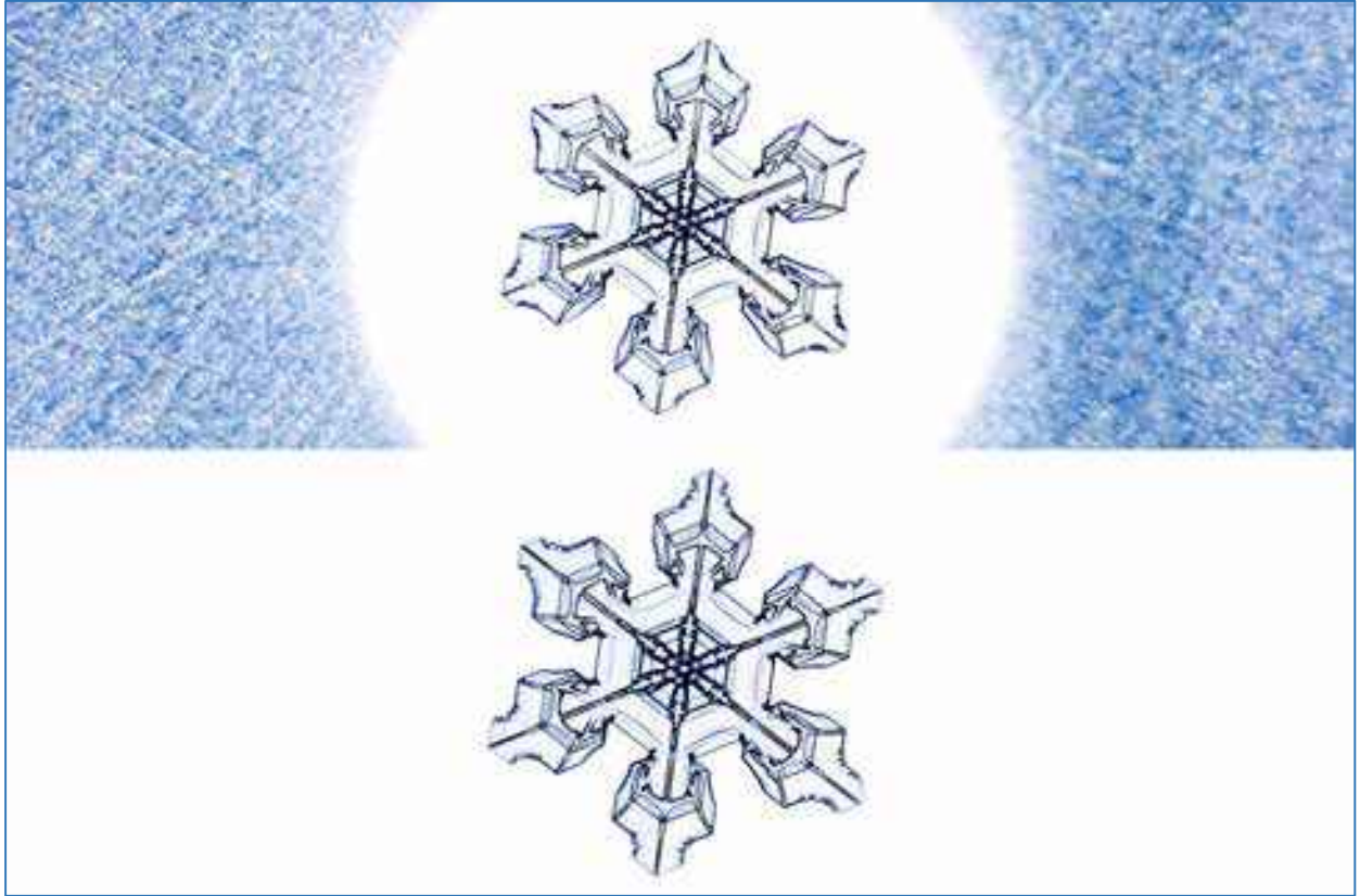
Figure 9.17: After growing the PoP crystal in the upper image, surrounded by a fog of water droplets, the supersaturation was reduced to a value 0 < \sigma < \sigma_{water} . Under these conditions, the water droplets soon evaporated away, while the crystal continued growing slowly, yielding the lower crystal surrounded by a clean substrate, free of droplets.
