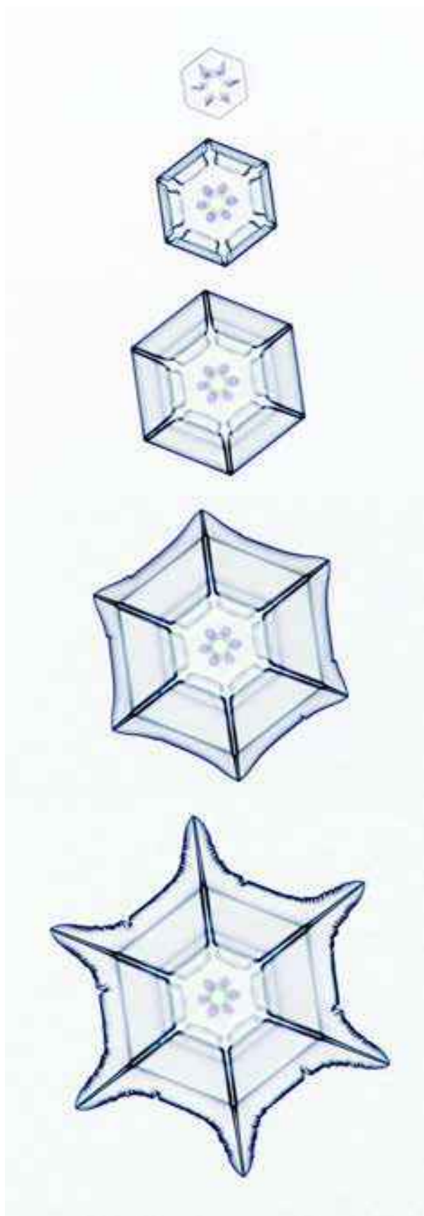
Figure 9.19: (Left) Another example of the onset of branching on a simple hexagonal plate, brought about by lowering the temperature to near -15 C and increasing the supersaturation. First the edge of the plate first grew thinner, then the prism facet started to become curved, and finally the branching instability kicked in. The small “petals” at the center of the crystal are bubbles trapped at the base of the pedestal, and again all of the surface structure is located on the underside of the plate, while the upper basal surface is almost perfectly flat.
