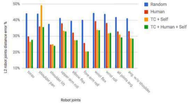
Fig. 16: L2 robot error break-down by robot joints . From left to right, we report errors for the 8 joints of the Fetch robot, followed by the joints average, followed by the joints average excluding the "shoulder pan" joint.
