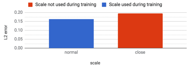
Fig. 20: Testing for scale invariance: while the error increases when decreasing the distance of the camera to the subject (about half way compared to training), it remains competitive and lower than the human-supervised baseline.
