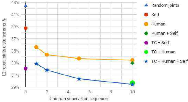
Fig. 13: Comparing types and amounts of supervision : Self-supervised imitation ("TC+self") outperforms human-supervised imitation ("Human").
