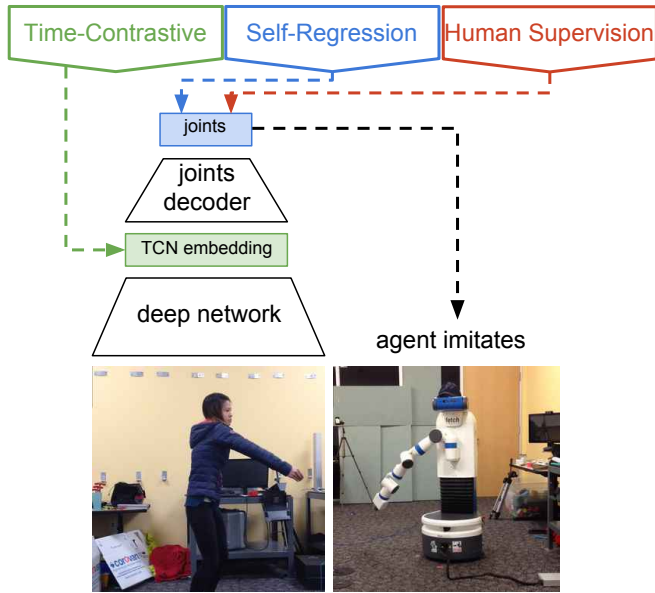
Fig. 8: TCN for self-supervised human pose imitation: architecture, training and imitation. The embedding is trained unsupervised with the time-contrastive loss, while the joints decoder can be trained with self-supervision, human supervision or both. Output joints can be used directly by the robot planner to perform the imitation. Human pose is never explicitly represented.
