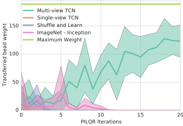
Fig. 12: Learning progress of the pouring task , using a single 3rd-person human demonstration that is different than the one shown in Fig. 6. This graph reports the weight in grams measured from the target recipient after each pouring action (maximum weight is 189g) along with the standard deviation of all 10 rollouts per iteration. The robot manages to successfully learn the pouring task using the multi-view TCN model after 20 iterations.
