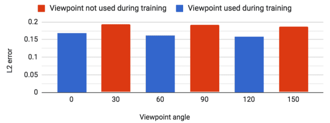
Fig. 19: Testing TC+Human+Self model for orientation invariance: while the error increases for viewpoints not seen during training ( 30^\circ , 90^\circ and 150^\circ ), it remains competitive.
