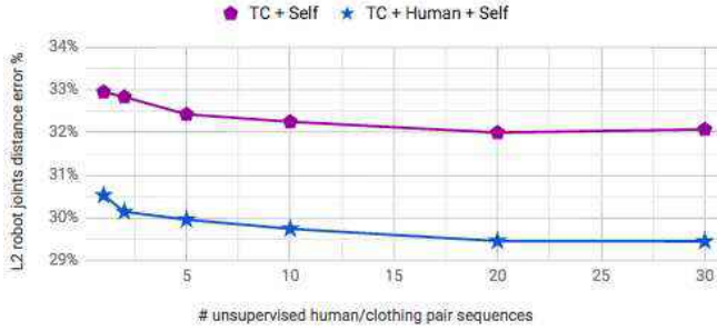
Fig. 15: Varying the amount of unsupervised data : increasing the number of unsupervised sequences decreases the imitation error for both models.
