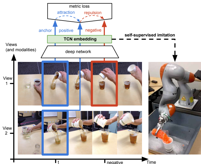
Fig. 1: Time-Contrastive Networks (TCN): Anchor and positive images taken from simultaneous viewpoints are encouraged to be close in the embedding space, while distant from negative images taken from a different time in the same sequence. The model trains itself by trying to answer the following questions simultaneously: What is common between the different-looking blue frames? What is different between the similar-looking red and blue frames? The resulting embedding can be used for self-supervised robotics in general, but can also naturally handle 3rd-person imitation.
