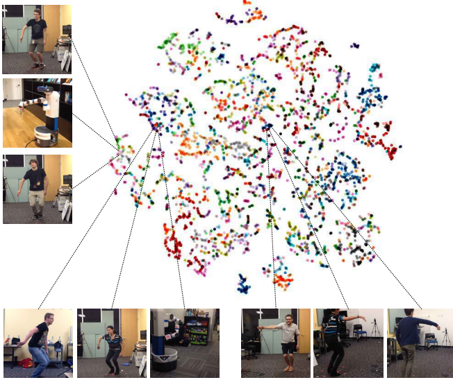
Fig. 14: t-SNE embedding colored by agent for model "TC+Self" . We show that images are locally coherent with respect to pose while being invariant to agent or viewpoint.
