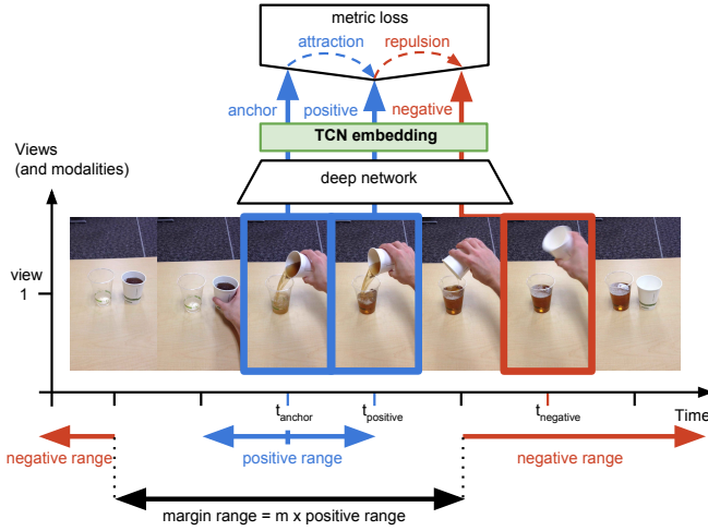
Fig. 3: Single-view TCN : positives are selected within a small window around anchors, while negatives are selected from distant timesteps in the same sequence.
