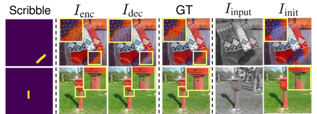
Figure 12: Qualitative comparisons of edge-enhancing network applied in encoder and decoder layers. I_{\text{enc}} and I_{\text{dec}} denote the enhanced results of the respective setting.
