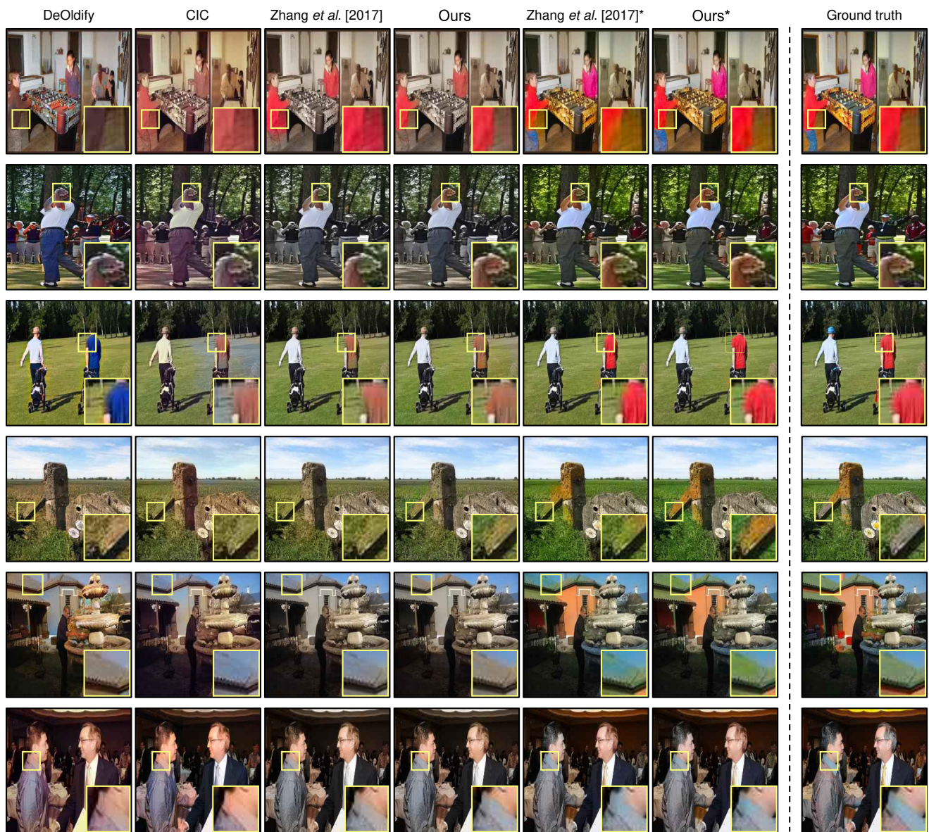
Figure 17: Qualitative comparisons between our model applied to Zhang et al. [6] and other baseline models.
