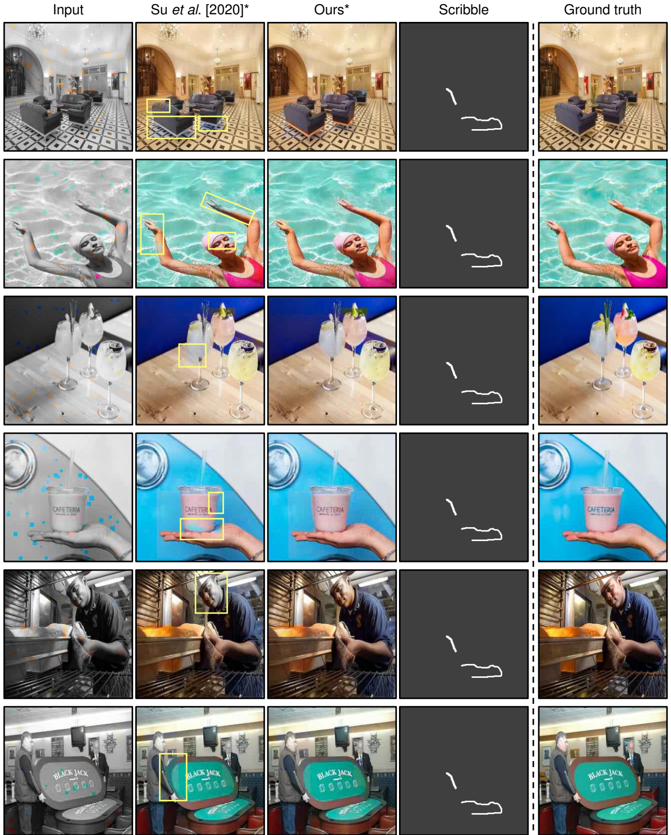
Figure 16: Qualitative results of edge-enhancement of our method applied to Su et al. [5]
