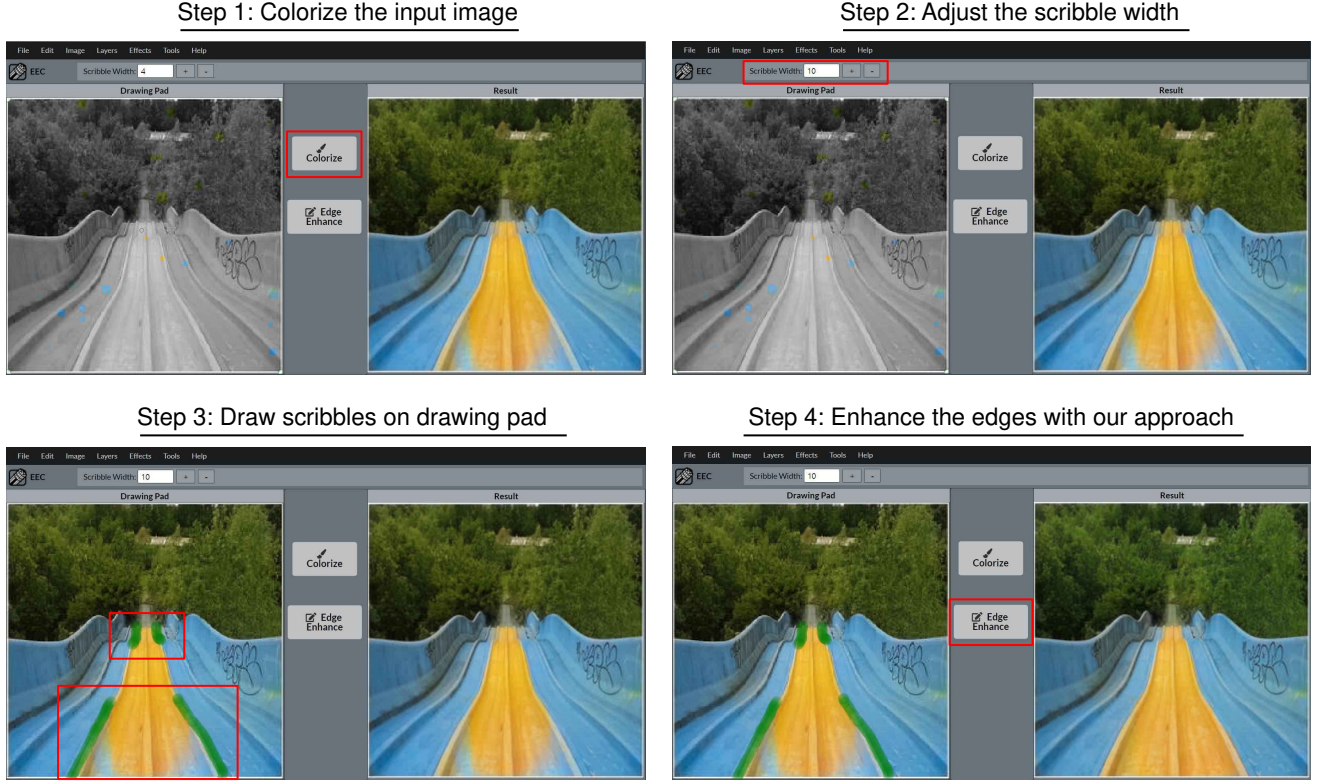
Figure 13: A step-by-step demonstration of an edge enhancement via our proposed user interface tool.
