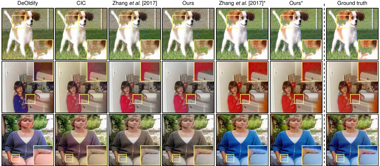
Figure 6: Qualitative comparisons between our model and baseline models. These images include color-bleeding in the same region for all baselines. Qualitative results show that our model successfully refinement this bleeding.
