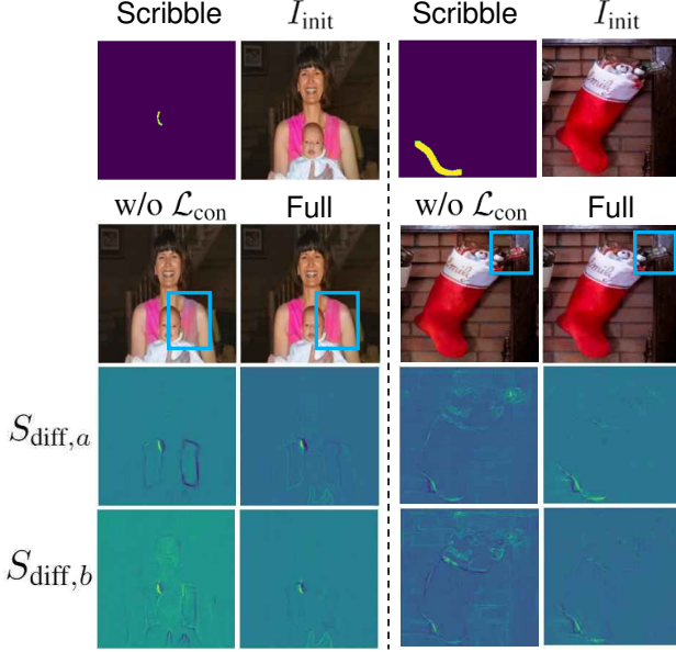
Figure 10: Qualitative comparisons between the generated outputs from our approach trained with and without \mathcal{L}_{\text{con}} in the training. The column denoted as w/o \mathcal{L}_{\text{con}} contains the results of our model without \mathcal{L}_{\text{con}} , and the column denoted as Full corresponds to the results of our model with all the proposed techniques, including \mathcal{L}_{\text{con}} .
