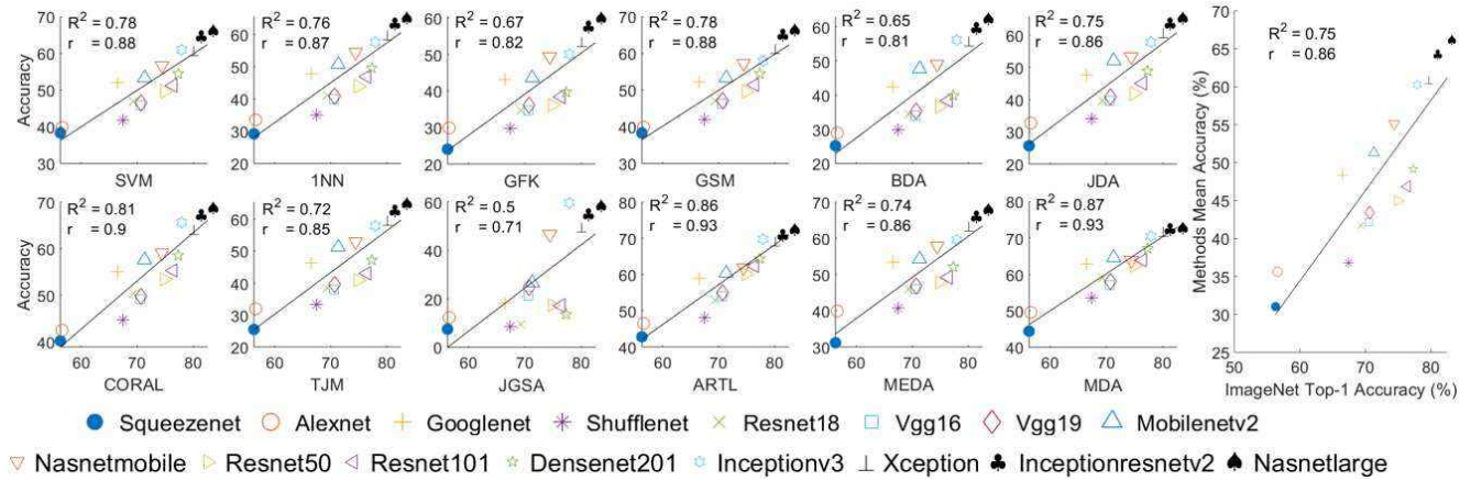
(c) Correlation and R^2 square value of Office-Home dataset
