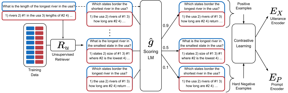
Figure 2: An overview of our approach for training EPR. Given a training example, we use an unsupervised retriever R_u to obtain a set of candidates. We then pass the candidates to a scoring LM and label the top- k and the bottom- k as positive and negative examples, respectively. Last, we use this training data to train a dense retriever.
