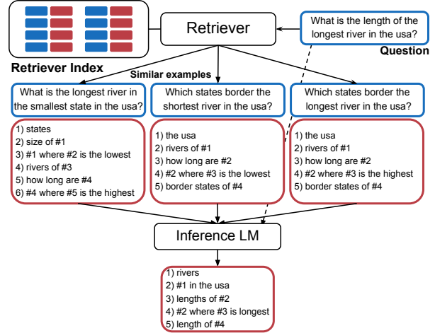
Figure 1: An overview of prompt retrieval: Given a question from BREAK, we retrieve similar training examples from an index of the training set. The question and training examples (the prompt) are passed to an inference LM that decodes the output.
