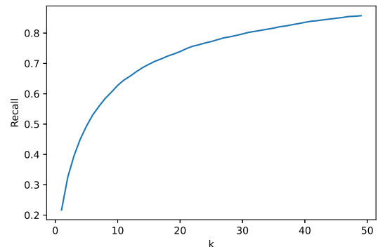
Figure 3: Recall@ k for EPR on BREAK, w.r.t labels given by the scoring LM. We compute Recall@ k by checking whether the top- k prompts retrieved include at least one example that was labeled as positive by the scoring LM.
