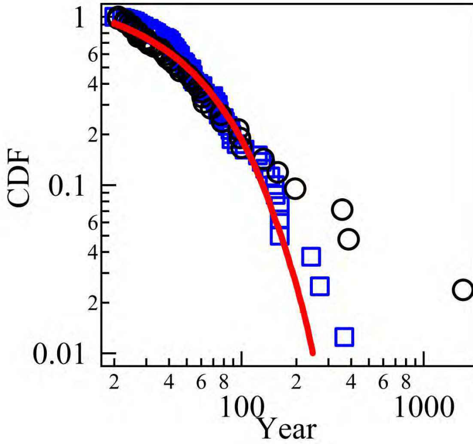
Fig. 5: Complementary cumulative distribution functions (ccdf) of the times-to-proof for open problems (rectangles), closed problems (circles) and an exponential distribution with rate 0.02 (continuous line), obtained by introducing a lower threshold equal to 20 years, i.e., by removing all times-to-proof smaller than 20 years.
