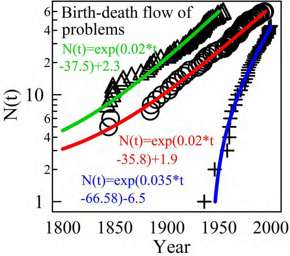
Fig. 2: Cumulative number of stated problems N_{closed}(t) that have found a solution (circles), cumulative number of stated problems N_{stated}(t) that are both closed and still open (triangles) and the cumulative number N_{solution}(t) of the solutions of the solved problems (crosses) from 1850 CE to 2000. The continuous lines correspond to the exponential growth models (8-10).
