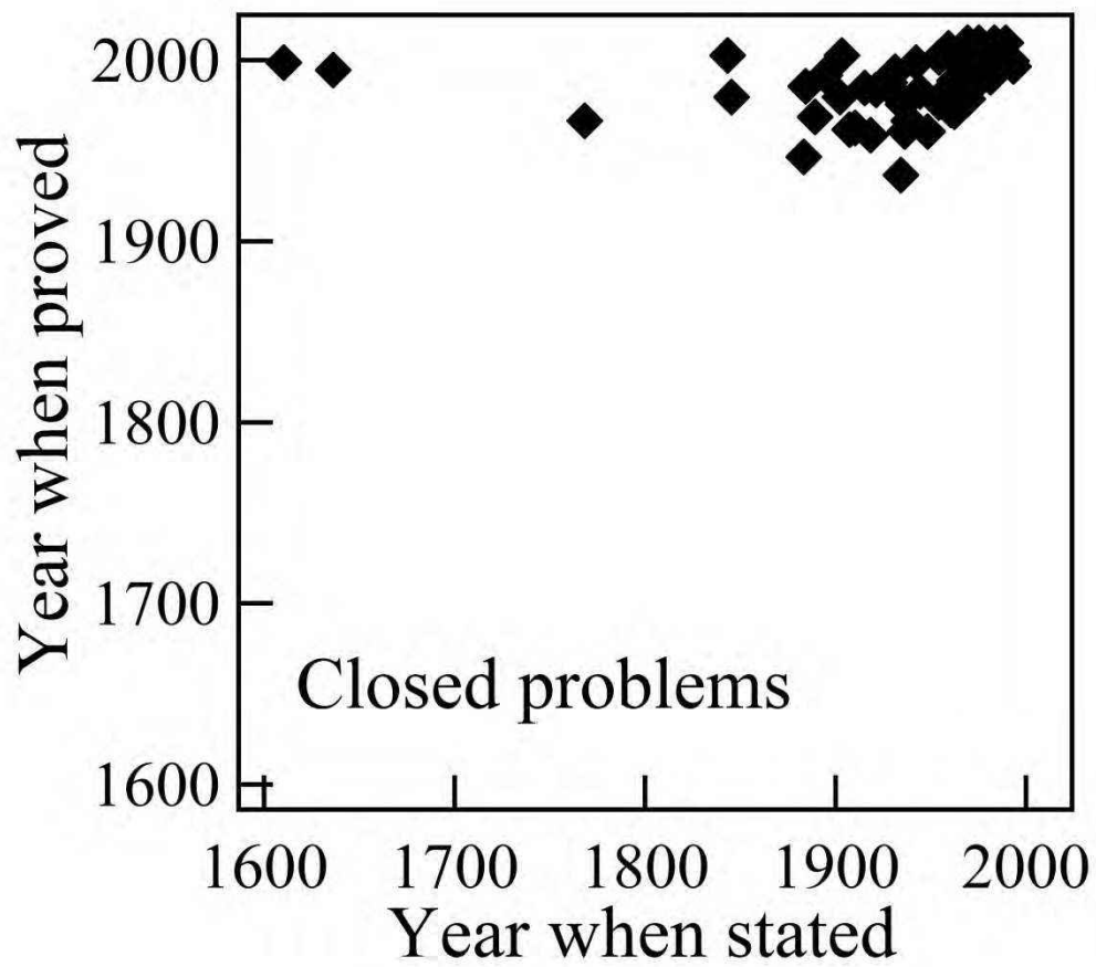
Fig. 1: Scatter plot showing when a mathematical problem was formed and when it was resolved for all 60 closed problems in our dataset, starting from the year 1600.
