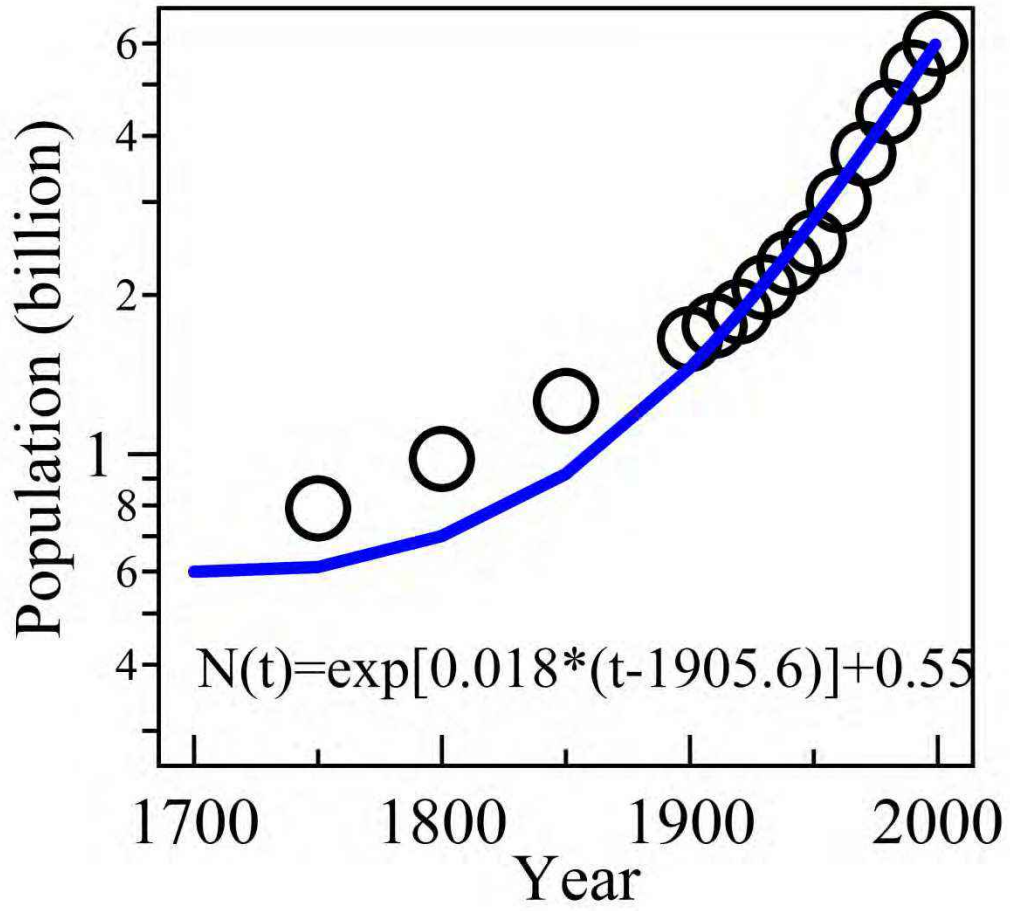
Fig. 3: Growth of the World population from 1750 to present (data retrieved from the United Nations website [6]), taken as the simplest proxy for the growth of the relevant population of mathematicians. This growth can be reasonably approximated by an exponential growth given by expression (11).
