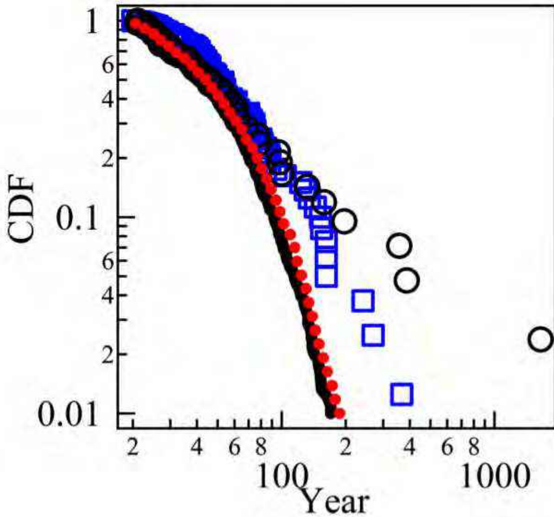
Fig .6: Comparison between the empirical cumulative distribution functions (ccdf) of the times-to-proof for open problems (rectangles), closed problems (circles) and the ccdf generated by the simple model presented in the text using an exponential distribution of the intrinsic time-to-proofs with rate \lambda = 0.01/\text{year} .
