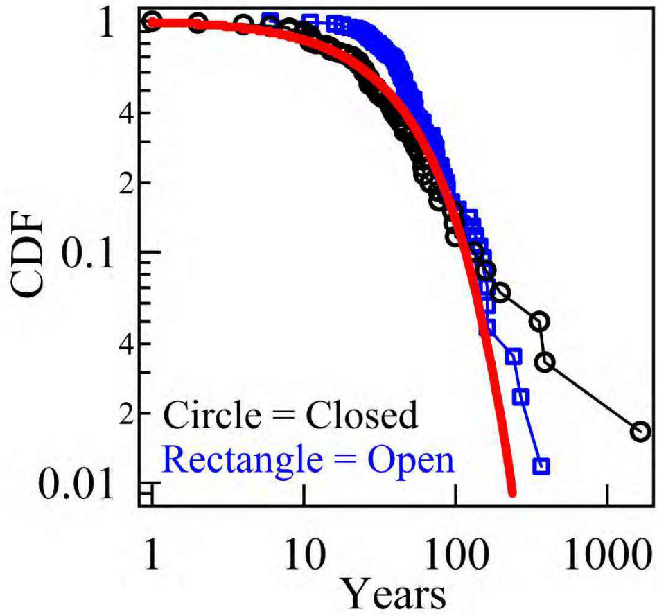
Fig. 4: Complementary cumulative distribution functions (ccdf) of the times-to-proof for open problems (rectangles), closed problems (circles) and an exponential distribution with rate 0.02 (continuous line).
