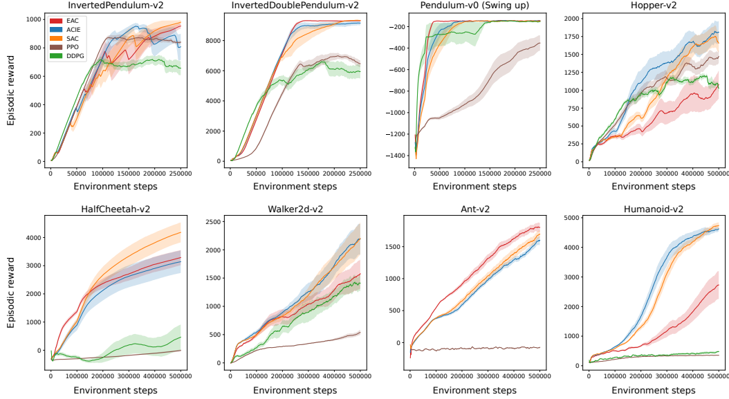
Figure 3: Raw Results of MuJoCo Experiments. The plots are similar to the plots from Figure 2, but report episodic rewards (averaged over the last 100 episodes) versus steps—not maximum episodic rewards seen so far as in [9]. For the pendulum tasks, the limits of the y-axes are preserved.
