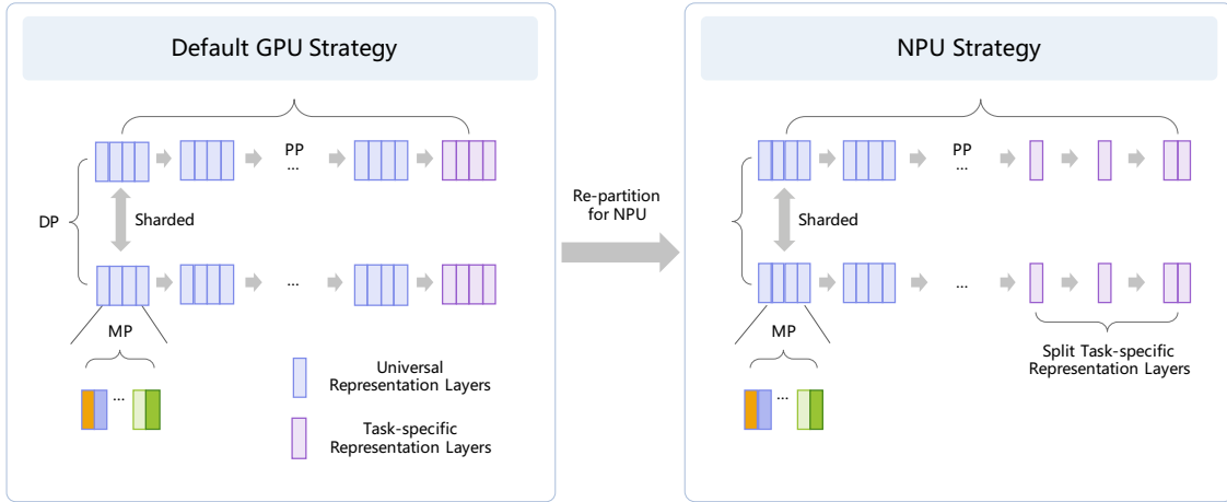
Figure 3: Resource-aware-partition.
