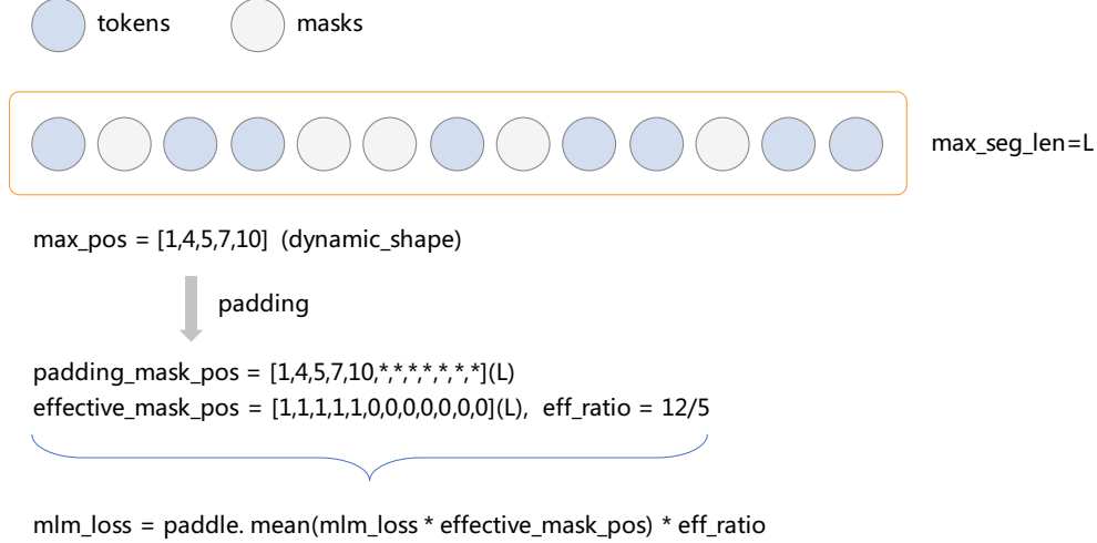
Figure 4: Convert dynamic shape to static shape.
