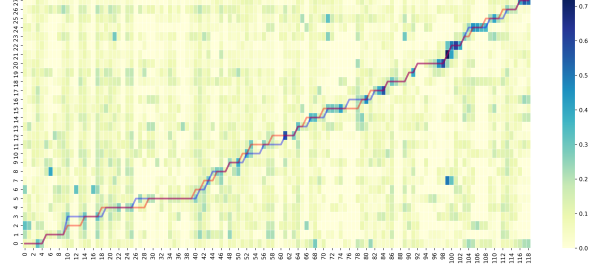
Figure 2: The Alignment of dialogues and narrative segments of a movie. X-axis and Y-axis are the ID of dialogue sessions and narrative segments, respectively. The variety of colors depicts the different similarity values between a dialogue session and a narrative segment. The blue line is the predicted alignment via normalized TF-IDF while the red line is the gold alignment.
