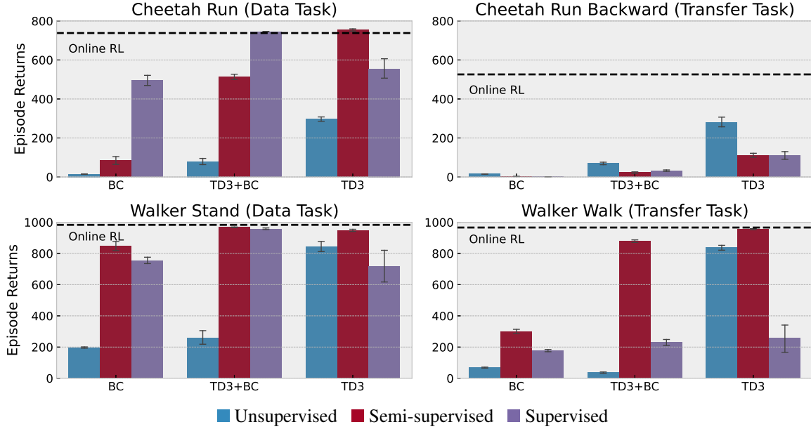
Figure 5. A comparison of three different data-collection strategies: unsupervised (intrinsic reward only), semi-supervised (intrinsic reward plus data task reward), and supervised (data task reward only). Data diversity is key to enable more aggressive trajectory stitching and task transfer.
