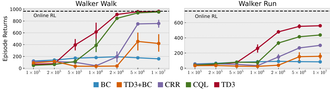
(a) Correlation between TD3 performance and the unsupervised data collection transition budget.
