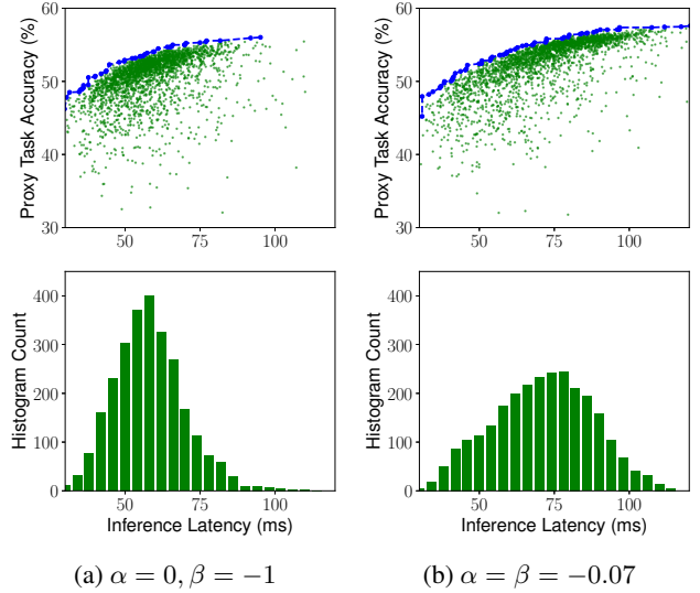
Figure 6: Multi-Objective Search Results based on equation 2 with (a) \alpha=0 , \beta=-1 ; and (b) \alpha=\beta=-0.07 . Target latency is T=75ms . Top figure shows the Pareto curve (blue line) for the 3000 sampled models (green dots); bottom figure shows the histogram of model latency.
