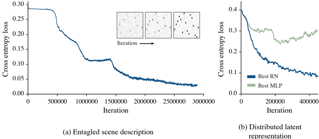
Figure 6: Inferring relational structure from entangled scenes. (a) A RN augmented with a linear layer U is able to reason about object relations from a scene description matrix that has been entangled with a random permutation matrix B . Examples of matrix UB (inset) during training (for a single example seed) illustrates that the linear layer learns to recover factorised object representations. (b) Distributed latent representations are inferred latent variables from VAE processing of image depictions of the scenes.
