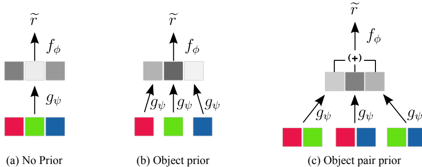
Figure 1: Model types. RNs are constructed to operate with an explicit prior on the input space (c). Features from all pairwise combinations of objects act as input to the same MLP, g_\psi .
