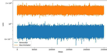
FIGURE 4. Training losses of the generator and the discriminator for TTUR based on Adam with constant learning rates \alpha^G = 10^{-10} and \alpha^D = 10^{-10} and batch size b = 2^6 versus number of steps for training DCGAN on the CIFAR-10 dataset (FID fluctuated between 290 and 330)
