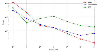
FIGURE 6. Number of steps for TTUR based on SGD, Momentum, and Adam versus batch size needed to train DCGAN on CIFAR-10. The number of steps N for TTUR based on Adam is a monotone decreasing function of b .
