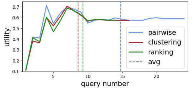
Figure 10: Utility: This graph shows the reached utility over time, according to the utility function we defined and described to the participants in words. All query types have similar performance. We can also see that the average number of answered queries in the pairwise setting is about 15, and 8-10 in the clustering/ranking scenario within the given minute.
