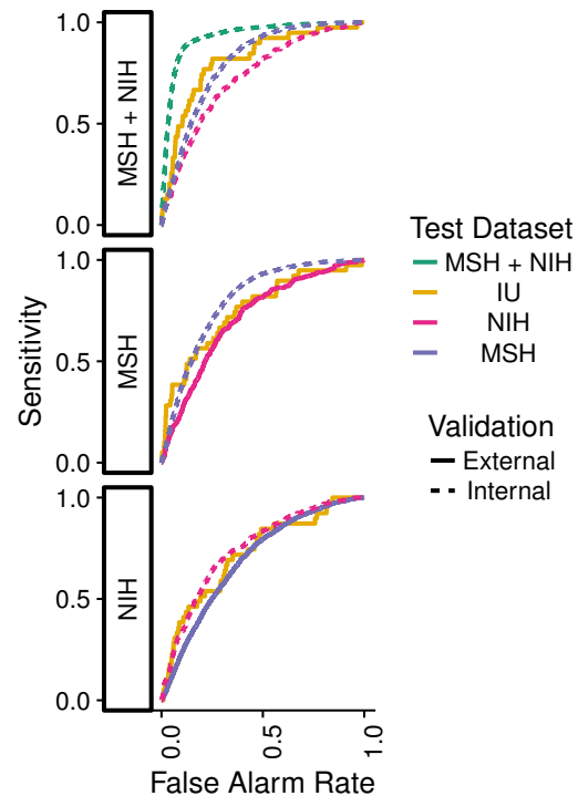
Fig 3. Pneumonia models evaluated on internal and external test sets. A model trained using both Mount Sinai and NIH data (MSH+NIH) had higher performance on the combined MSH+NIH test set than on either subset individually or on fully external Indiana (IU) data.
