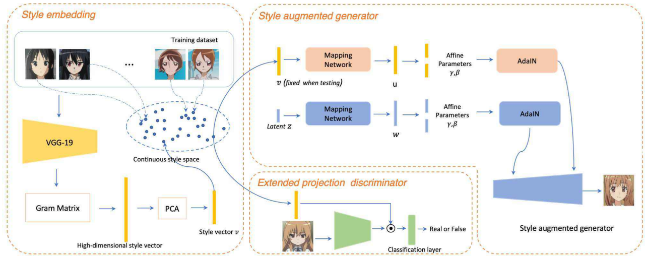
Figure 2: Overview of the proposed framework. First, all collected images are embedded in a continuous space by using Gram matrix (Gatys, Ecker, and Bethge 2016) and PCA. Spatial proximity of the embedded style vectors well reflects the visual style similarity of the original images. Style vector is sampled and passed through the mapping network. It is used as affine parameters to modulate the image generator’s AdaIN modules. A projection discriminator is used to take into account the style vector and supervise the generator. Combining these components we are able to precisely control the style of the generated images to match that of each single training example or to interpolate between them using their corresponding style vectors.
