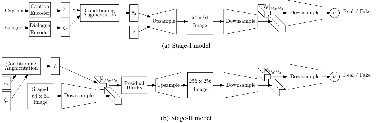
Figure 3. ChatPainter: (a) Stage-I of the model generates a 64 \times 64 image conditioned on a caption and the corresponding dialogue. (b) Stage-II of the model generates a 256 \times 256 image conditioned on Stage-I’s 64 \times 64 generated image and the caption and corresponding dialogue.
