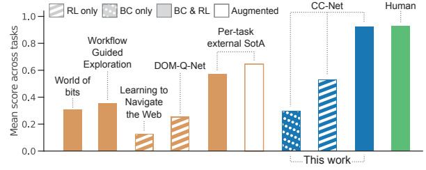
Figure 3 | Mean performance across MiniWob++ tasks. Shown are previously published MiniWob++ results (Gur et al., 2018; Jia et al., 2019; Liu et al., 2018; Shi et al., 2017), which each only report performance for a subset of tasks (for these results the performance on non-reported tasks is set to zero, all scores used are given in Appendix Table 3). In order to make a fair comparison, we combine the best external results for each task into aggregated external SotA scores, reporting those obtained both with and without additional augmentations (we filter the 16 out of 104 tasks without external scores from our corresponding results). Our agent, CC-Net, outperforms these results by a large margin, and matches mean human performance. We achieve this without using environment augmentations. Instead, we find that the combination of BC and RL is crucial to CC-Net performance; BC- and RL-only training are less effective.
