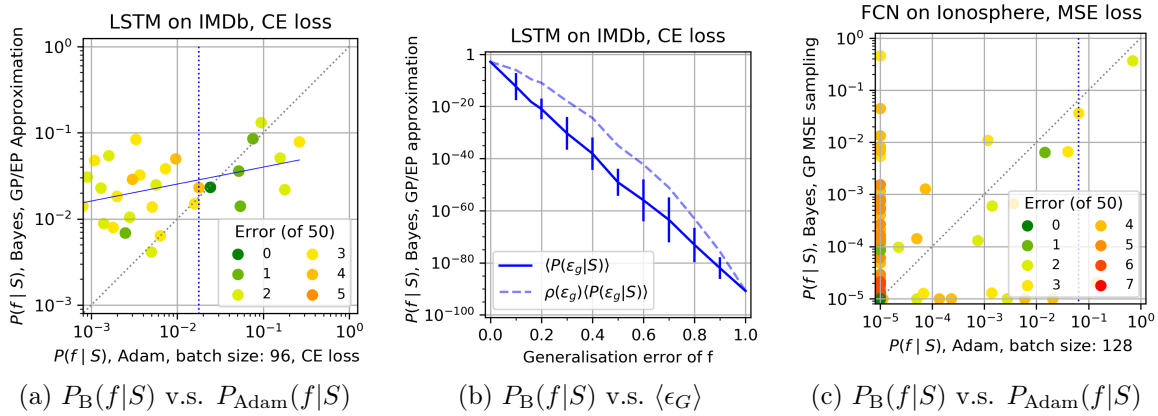
Figure 4: Comparing P_B(f|S) to P_{\text{Adam}}(f|S) for a LSTM on the IMDB movie review dataset, and an FCN on the ionosphere dataset. (a) P_B(f|S) v.s. P_{\text{Adam}}(f|S) for LSTM on IMDB dataset, ( \langle \epsilon_G \rangle = 4.28\% , 10^4 samples). Because of the computational cost of the problem, we used a training set size of 45000 and a test set of size 50. (b) P_B(f|S) v.s. \langle \epsilon_G \rangle for the LSTM on IMDB shows that the functions found by the Adam optimiser are in the small fraction of high P_B(f|S) probability/low error functions. (c) P_B(f|S) v.s. P_{\text{Adam}}(f|S) for an FCN with 3 hidden layers of width 256 on the Ionosphere dataset. Training set size is 301 and the test set size is 50. ( \langle \epsilon_G \rangle = 4.59\% for Adam, \langle \epsilon_G \rangle = 5.41\% for the GP). See Figures 14 and 15 for further results for these systems.
