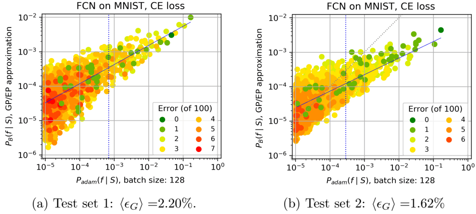
Figure 12: Comparing P_{\text{B}}(f|S) to P_{\text{AAdam}}(f|S) for an FCN on MNIST with CE loss for two different test sets [We use training/test set size 10,000/100 and batch size=128. Vertical dotted blue lines denote 90% probability boundary; solid blue lines are fit to guide the eye; dashed grey line is x = y .] (a) is the test set used throughout the paper and (b) is another test set (disjoint from both the first test set and the training set), chosen at random from MNIST. To first order the two look very similar, but to second order small differences can be seen, not just in the function probabilities, but also in the slope of P_{\text{B}}(f|S) v.s. P_{\text{AAdam}}(f|S) , which may be affected by the EP approximation used here. No normalisation was applied to this figure so it depicts the raw EP approximation (see Appendix A.2.2).
