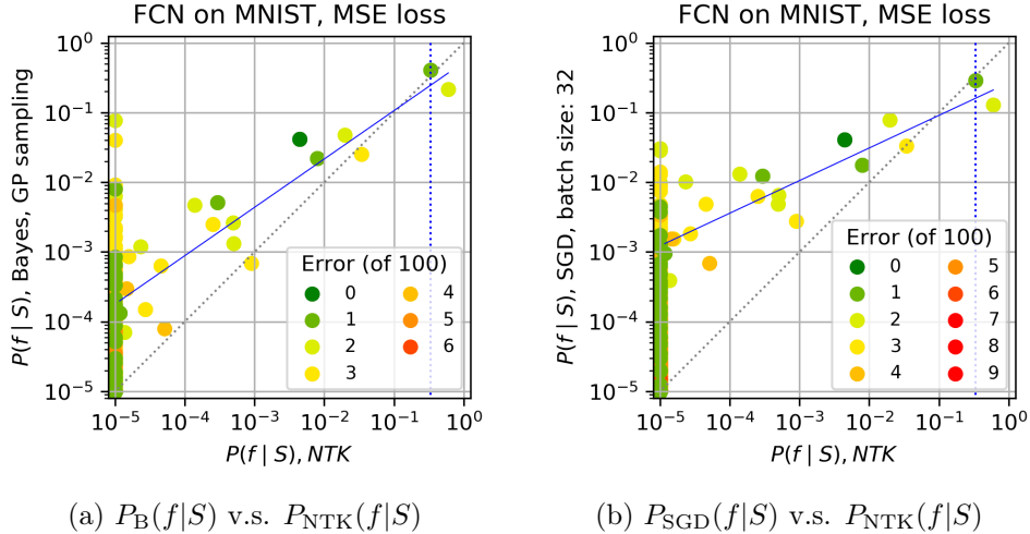
Figure 3: Comparing P_B(f|S) and P_{\text{SGD}}(f|S) to P_{\text{NTK}}(f|S) for an FCN on MNIST. [The functions to the right of the blue dotted lines make up 90% of the total probability. We did 10^7 samples for NTK and GP, and 10^6 for SGD]. In (a) we show the correlation between P_{\text{NTK}}(f|\mathcal{D}) and P_B(f|S) . Weighted by probability, 77.5% of functions found by sampling from the GP are found by NTK; all functions found by NTK are found by sampling from the GP. In (b), we show the correlation between the P_{\text{NTK}}(f|\mathcal{D}) and P_{\text{SGD}}(f|S) . Weighted by probability, 65.8% of functions found by SGD are found by NTK; all functions found by NTK are found by SGD. \langle \epsilon_G \rangle = 1.69\% (NTK), \langle \epsilon_G \rangle = 1.61\% (GP), \langle \epsilon_G \rangle = 1.88\% (SGD).
