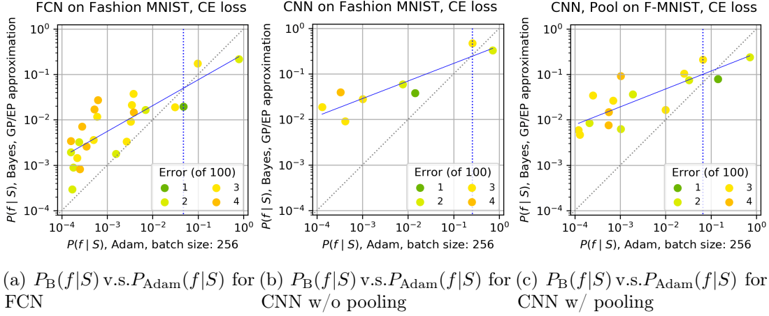
Figure 2: Comparing P_B(f|S) to P_{\text{Adam}}(f|S) for CNNs and the FCN on Fashion-MNIST [We use a training/test set size of 10,000/100; vertical dotted blue lines denote 90% probability boundary; dashed grey line is P_B(f|S) = P_{\text{OPT}}(f|S) .] (a) FCN on Fashion-MNIST; \langle \epsilon_G \rangle = 2.11\% for Adam with CE loss. (b) Vanilla CNN on Fashion-MNIST; \langle \epsilon_G \rangle = 2.25\% for Adam with CE loss. (c) CNN with max-pooling on Fashion-MNIST; \langle \epsilon_G \rangle = 1.96\% for Adam with CE loss. Note that when max-pooling is added, the probability of the lowest-error function increases notably for both P_{\text{Adam}}(f|S) and P_B(f|S) . There is a strong correlation between P_B(f|S) and P_{\text{SGD}}(f|S) in all three plots. See Figure 13 for related results, including P_B(f|S) vs \epsilon_G , a CNN with batch normalisation, and a CNN with MSE loss.
