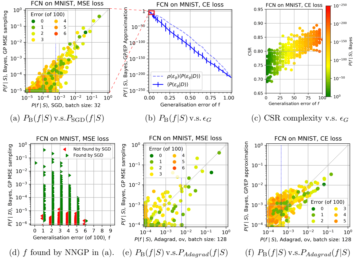
Figure 1: Comparing the Bayesian prediction P_B(f|S) to P_{OPT}(f|S) for SGD and Adagrad, for an FCN on MNIST [We use training/test set size of 10,000/100; For (a,e,f), the vertical dotted blue lines are drawn at the highest value of P_{OPT}(f|S) such that the sum of P_{OPT}(f|S) for all functions above the line is > 90\% (90% probability boundary); dashed grey line denotes P_B(f|S) = P_{OPT}(f|S) .]
