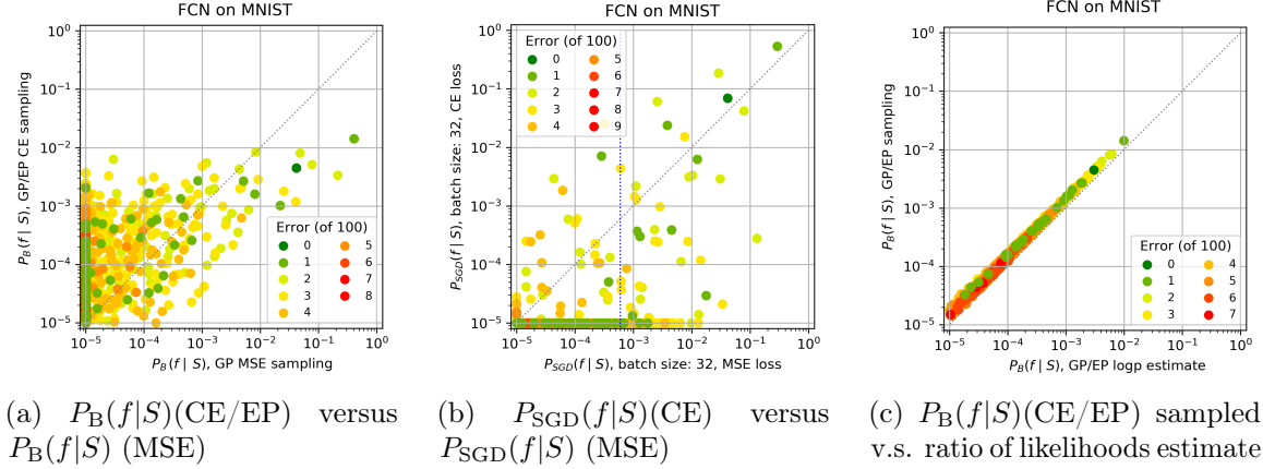
Figure 7: Comparing GP approximations with CE and MSE loss for FCN on MNIST In (a) we compare the behaviour of the GP approximations for P_{\text{B}}(f|S) with MSE loss to the GP/EP approximation with CE loss. We sampled from the GP MSE posterior, and the GP/EP CE posterior distribution 10^6 times. It is expected that the two measures should diverge somewhat due to details of the loss function on the training data. (b) compares P_{\text{SGD}}(f|S) with MSE loss and P_{\text{SGD}}(f|S) with CE loss. Functions with high P_{\text{SGD}}(f|S) are scattered around y = x . This implies that the loss function does not substantially affect P_{\text{SGD}}(f|S) on average. Note that in (a) the two methods correlate, but that 1) the GP-EP is systematically lower than the MSE, and 2) that the slope is below x = y . These two trends are, we believe, more general for the GP-EP approximation on CE loss. (c) Here we compare the GP/EP \log(p) approximation with GP/EP sampling. For this figure, we use only functions found by Adam in 10^6 samples, and compare probabilities found by the GP/EP \log(p) approximation to those found by GP/EP sampling. We use both methods in this paper, but as is clear from the above figure, there is not much difference between them for functions with high P_{\text{B}}(f|S) .
