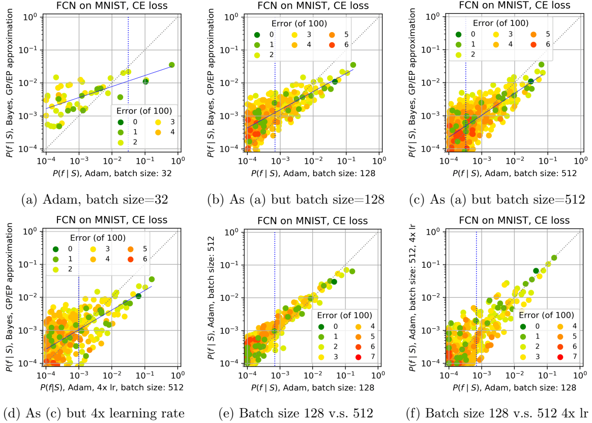
Figure 5: Effects of changing batch size and learning rate on P_B(f|S) and P_{\text{Adam}}(f|S) for FCN on MNIST with CE loss [We use training/test set size 10,000/100. Vertical dotted blue lines denote 90% probability boundary; dashed grey line is x = y .]
