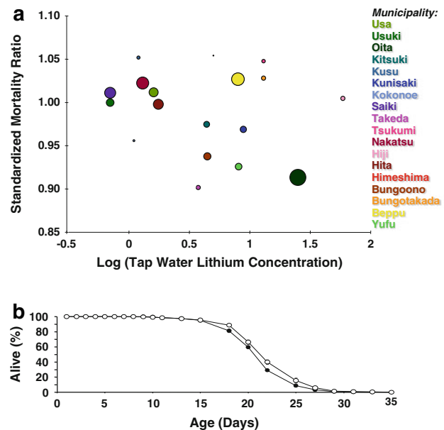
Fig. 1 Low-dose lithium exposure modulates mortality. a depicts data from 18 different Japanese municipalities which are named and color coded on the right-hand side . The numbers of inhabitants are reflected by the respective diameter of circles. The X-axis shows logarithmic median tap water lithium concentration, the Y-axis depicts the standardized mortality ratio, defined as number of observed deaths divided by the number of expected deaths. b depicts are mean values ( \pm SEM) of three separate experiments with approximately one hundred of C. elegans roundworms per experiment and condition. Black circles reflect control animals, open circles reflect animals that were continuously exposed to 10 \mu\text{M} lithium chloride
