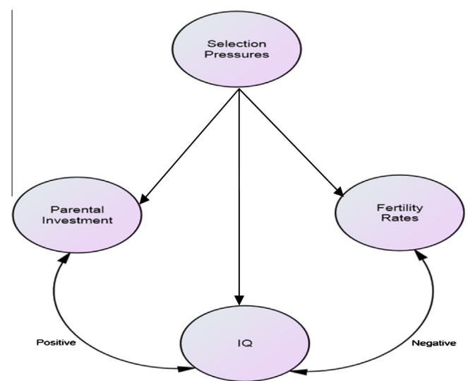
Fig. 1. Theoretical model.
