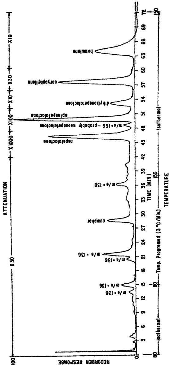
FIG. 2. GAS-LIQUID CHROMATOGRAPHIC ANALYSIS OF Nepeta cataria OIL. 0.05 \mu l OF THE OIL WAS USED. THE COLUMN WAS 45 M X 0.5 MM, APIEZON L-COATED AND KEPT AT 150°. THE HYDROGEN FLAME DETECTOR WAS KEPT AT 200°. THE HELIUM PRESSURE WAS KEPT AT 25 LB/IN 2 .
