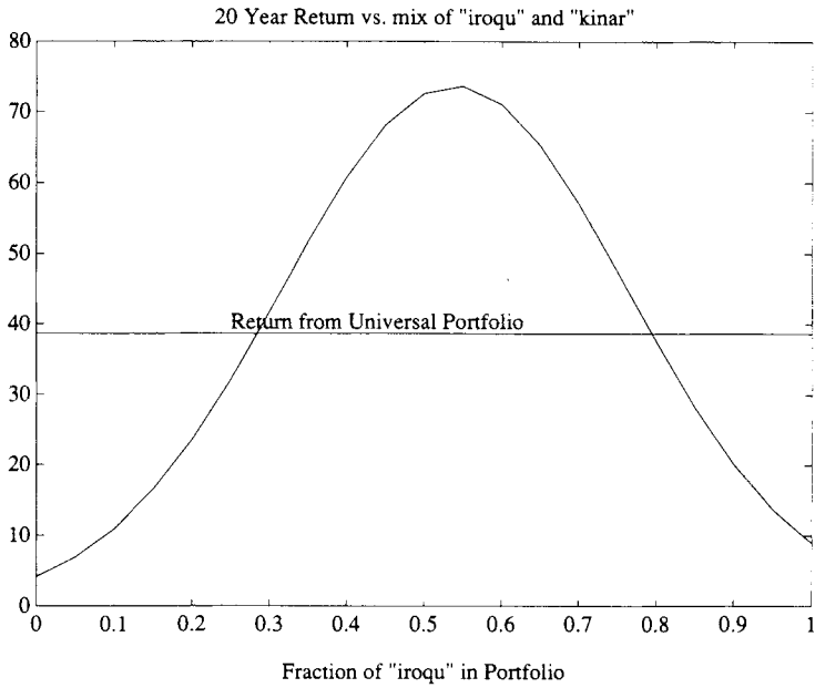
FIGURE 8.2. Performance of rebalanced portfolio.
