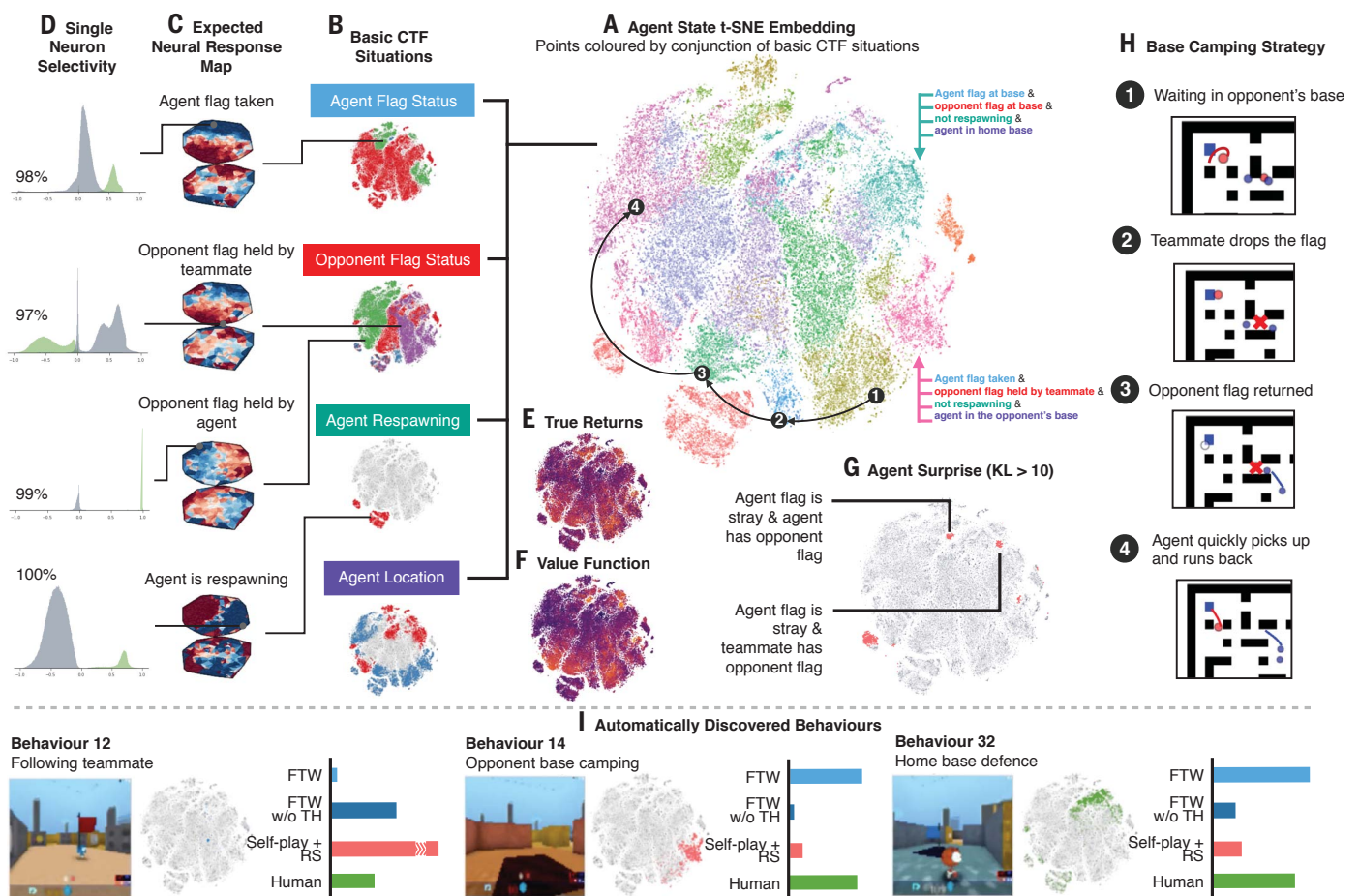
Fig. 3. Knowledge representation and behavioral analysis. (A) The 2D t-SNE embedding of an FTW agent’s internal states during gameplay. Each point represents the internal state ( h^p, h^q ) at a particular point in the game and is colored according to the high-level game state at this time—the conjunction of (B) four basic CTF situations, each state of which is colored distinctly. Color clusters form, showing that nearby regions in the internal representation of the agent correspond to the same high-level game state. (C) A visualization of the expected internal state arranged in a similarity-preserving topological embedding and colored according to activation (fig. S5). (D) Distributions of situation conditional activations (each conditional distribution is colored gray and green) for particular single neurons that are distinctly selective for these CTF
