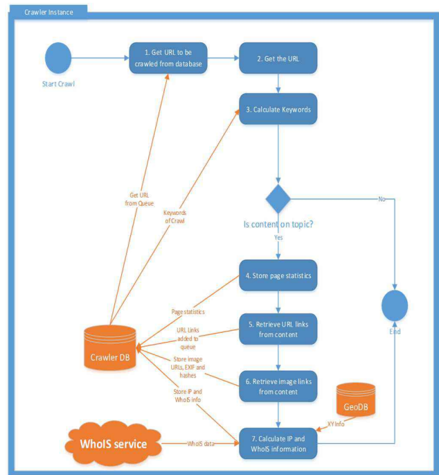
Fig. 1. Workflow associated with a thread of Dark Crawler
