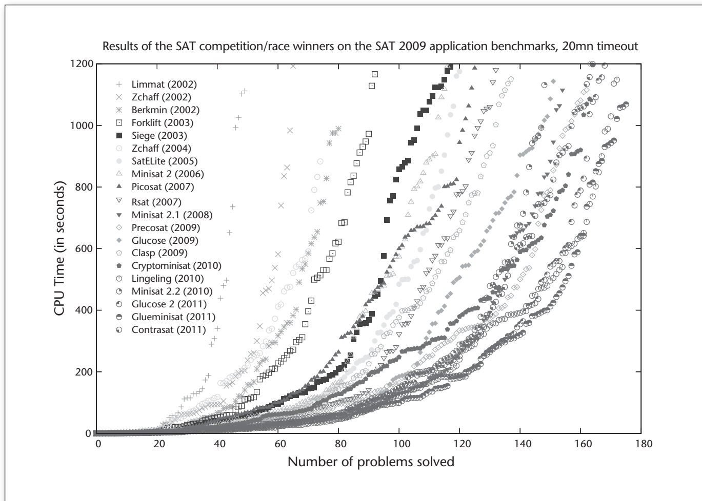
Figure 2. Performance Evolution of the Best SAT Solvers from 2002 to 2011.
