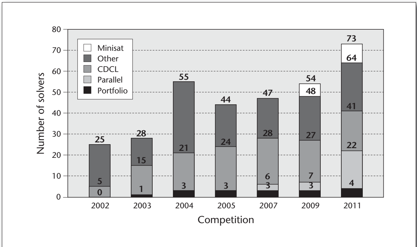
Figure 1. Evolution of SAT Competition Participation.
