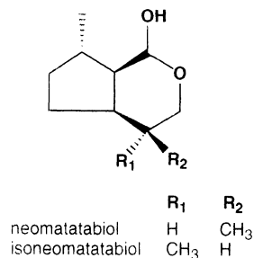
Fig. 2A,B. Structures of biologically active monoterpenoids from Actinidia polygama . (Sakan et al. 1964)
