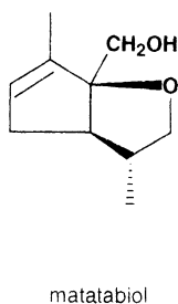
Fig. 2A,B. Structures of biologically active monoterpenoids from Actinidia polygama . (Sakan et al. 1964)
