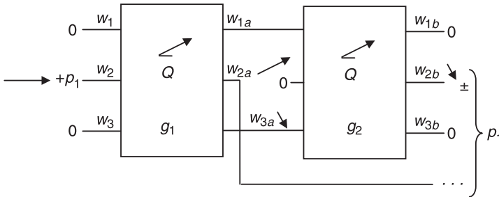
Figure 4.6 Again, reusing the same measurement angle causes no further state-splitting.
