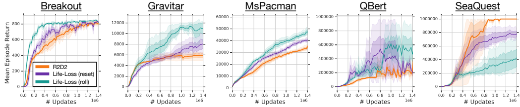
Figure 8: Ablation results for the use of life loss as episode termination on Atari, with standard deviations shown by shading (3 seeds). ‘reset’ refers to the agent variant using life losses as full episode terminations (preventing value function bootstrapping across life loss events, as well as resetting the LSTM state), whereas ‘roll’ only prevents value function bootstrapping, but unrolls the LSTM for the duration of a full episode (potentially spanning multiple life losses).
