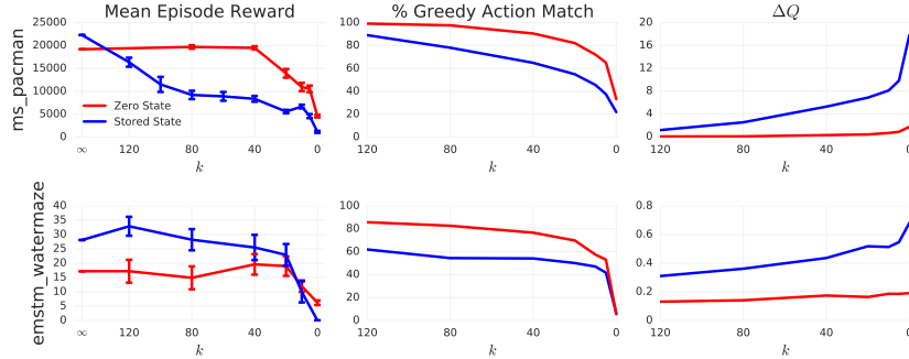
Figure 5: Effect of restricting R2D2's policy's memory on Ms.PACMAN and EMSTM_WATERMAZE.
