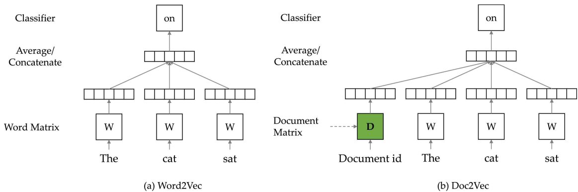
Figure 4: word2VecvsDoc2Vec Architecture [3]
