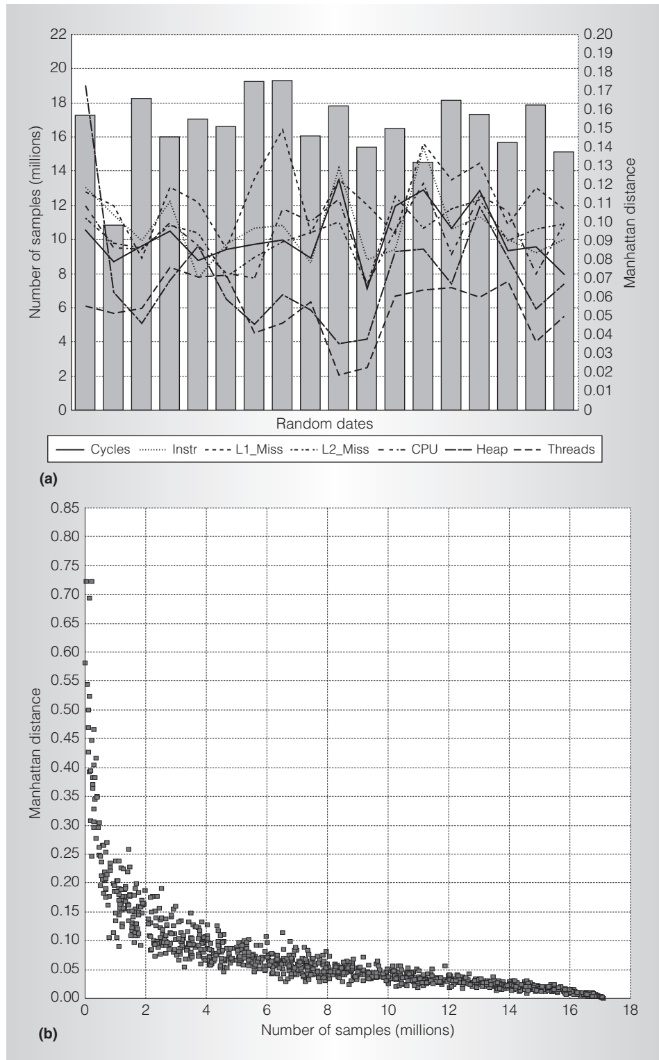
Figure 6. The Manhattan distance between daily application-level profiles for various profile types (a). The correlation between the number of samples and the Manhattan distance of profiles (b).
