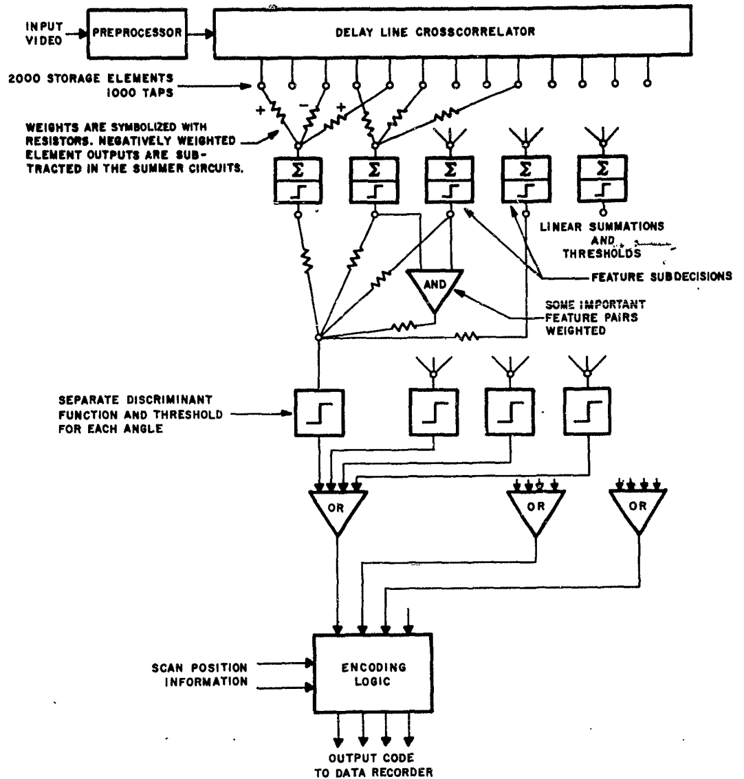
Figure 5-5 Organization of Recognition Logic
