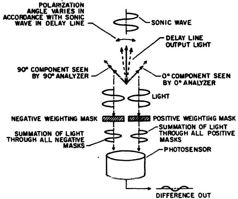
Figure 4-8(b) Another Way to Look at Carrier Commutation Subtraction
