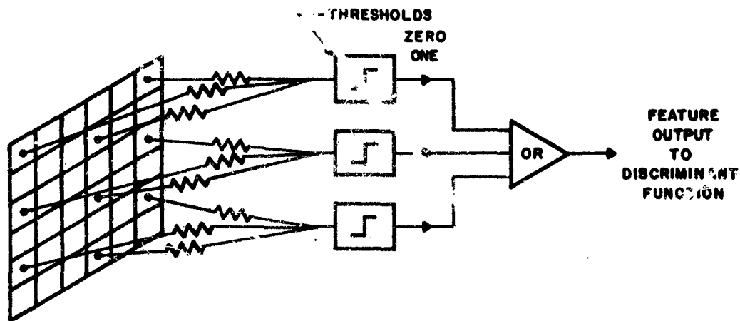
(b) FEATURE DETECTORS DISPLACED IN REGISTRY AS ABOVE BUT COMBINED IN OR GATE BEFORE USE BY THE DISCRIMINANT FUNCTION.
